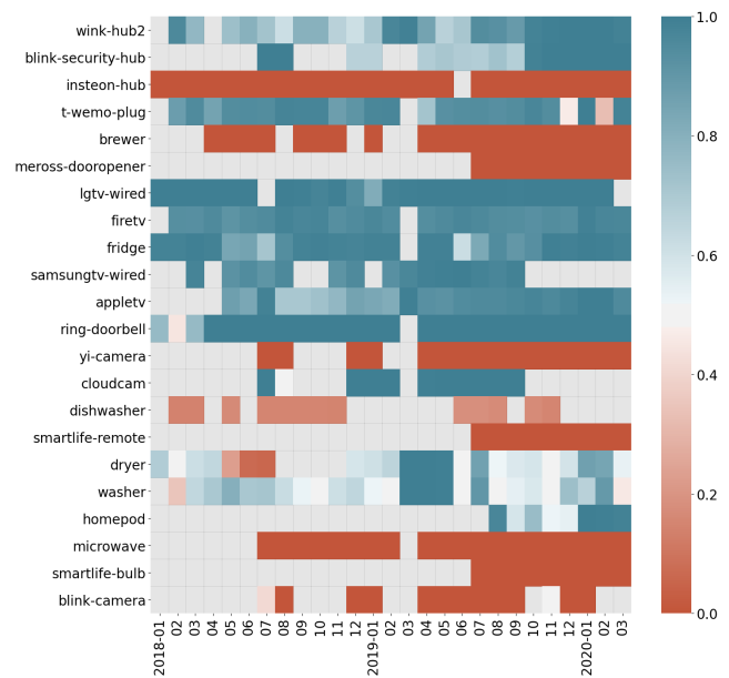
Figure 3: IoT devices that establish connections with strong ciphersuites (higher is better). Most devices do not adopt these ciphersuites over time. 18 devices use such ciphersuites for the vast majority of their established connections, and are not shown in this figure.
