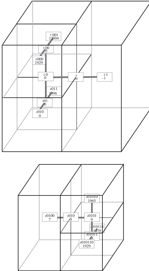
Figure 5.1. Six levels of subdivision, in two projections, with all the trimmings.
