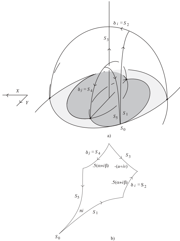
Figure 2.3. Two versions of the degenerate right-angled hexagon.
