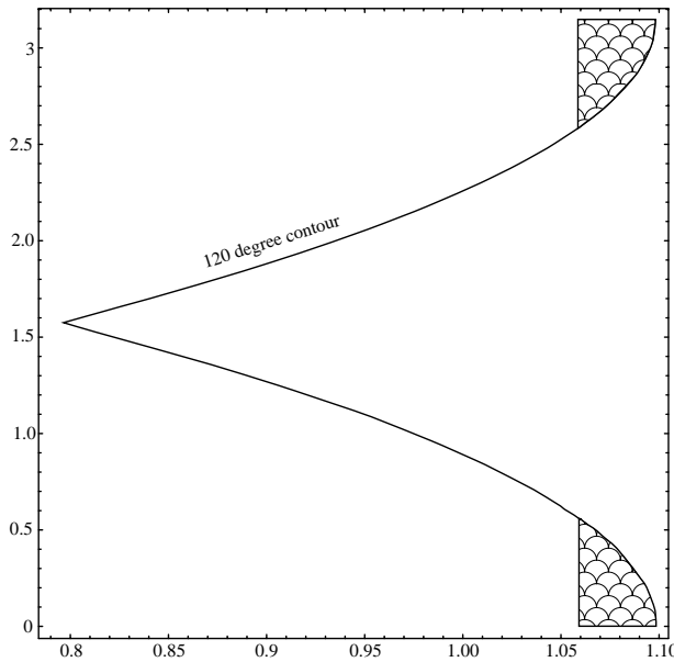
Figure 2.4. The 120-degree contour for the corona function \mathcal{C}(u, v) , and a decorated region which corresponds to corona greater than or equal to 120 degrees and u value greater than or equal to 1.059.
