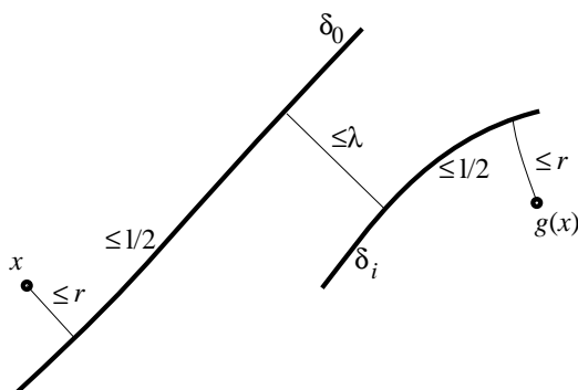
Figure 3.6. Controlling the based ortholength spectrum.
