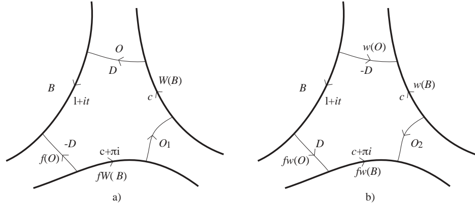
Figure 3.2. Two right-angled hexagons arising from Figure 3.1. Here B denotes the axis B_{(0,\infty)} .
