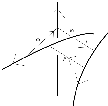
Figure 3.5. \cosh(P) = \cosh^2(\omega) + \sinh^2(\omega) \cosh(i(\pi/2 + \pi)) has solution P = \bar{\omega} .
