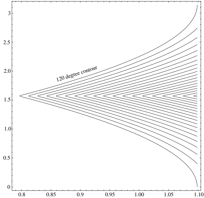
Figure 2.1. The 102 to 120 degree contours for the corona function \mathcal{C}(u, v) (for example, the 120 degree contour corresponds to where the corona function takes on value 2\pi/3 ).
