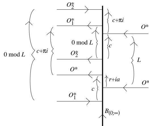
Figure 3.3. The values shown are the distances along B_{(0,\infty)} , between the indicated oriented ortholines and O_i^* denotes a g \in G translate of the orthocurve O_i .
