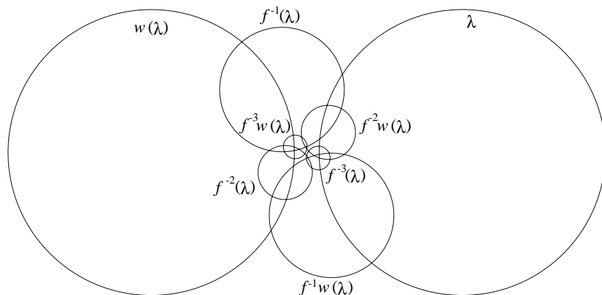
Figure 3.4. There is no tri-linking from \mathcal{O}(1) .
