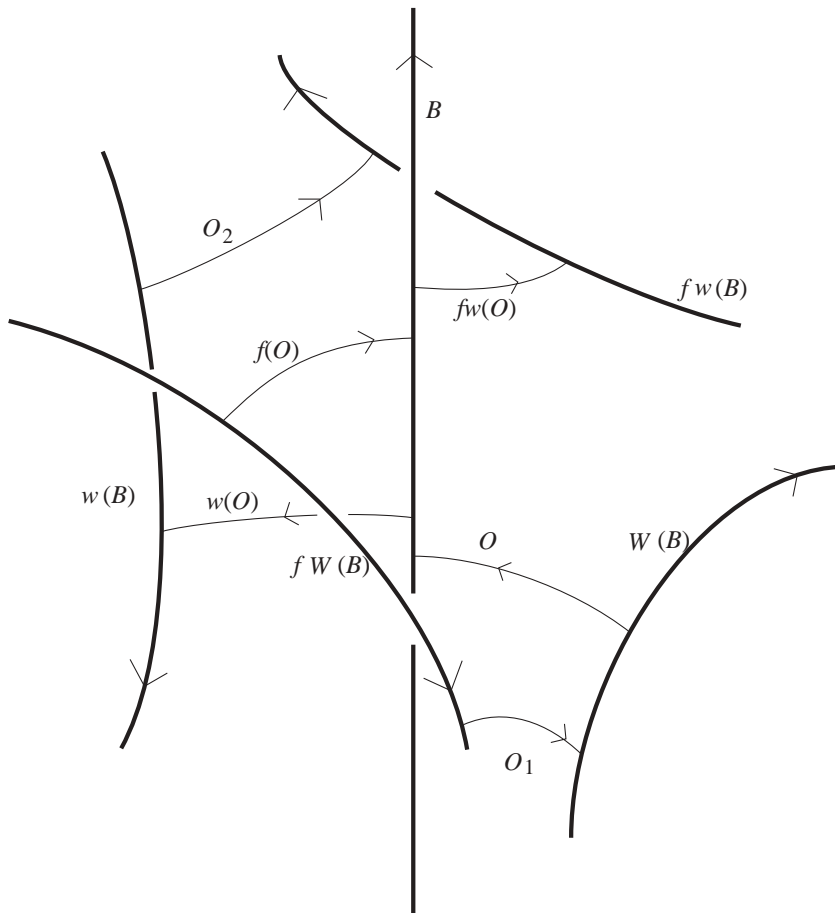
Figure 3.1. Various geodesics around B = B_{(0;\infty)} in \mathbf{H}^3 .
