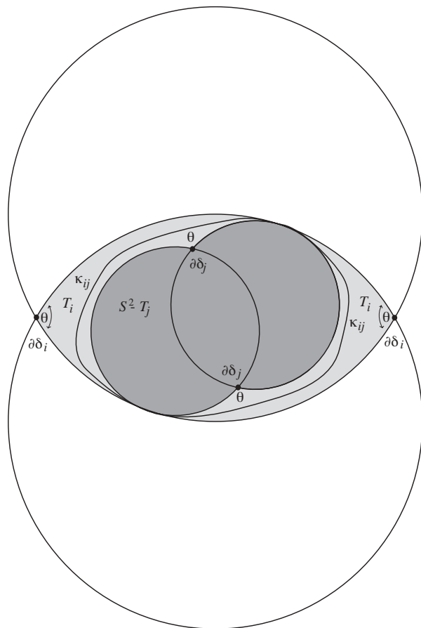
Figure 2.2. Here \text{dist}(\delta_i, \delta_j) is approximately .9 + (2\pi/5)i and C(\text{dist}(\delta_i, \delta_j)) is approximately 2\pi/3 . Note that the lightly shaded region is T_i \cap T_j while the darkly shaded region is S_\infty^2 - T_j .
