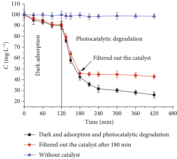
FIGURE 10: Leaching experiment ( V = 500 \text{ mL} , C_0 = 100 \text{ mg} \cdot \text{L}^{-1} ; mass of catalyst: 100 mg).
