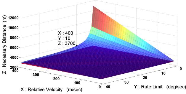
Fig. 6. Envelope for successful collision avoidance when \sigma = 20 (deg).
