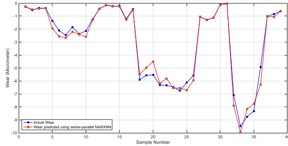
Fig. 13 Actual and predicted wheel wear using series-parallel NARXNN under dry conditions (based on unseen input data)
