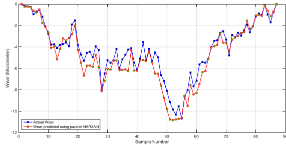
Fig. 14 Actual and predicted wheel wear using parallel NARXNN under dry conditions (based on unseen input data)
