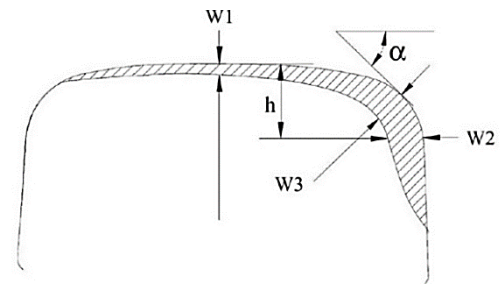
Fig. 2 Rail wear [3]
