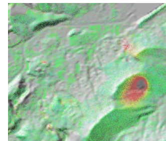
Average deformation rate over a small section of the Baisha Hu mining area, derived from 9 LuTan-1 scenes between Jul. and Nov. 2023, Color scale is between -25cm/y and 25cm/y, brightness is shaded relief of Copernicus DEM.
