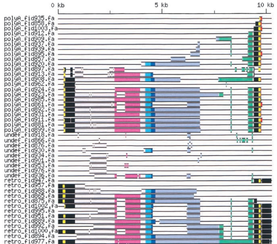
Figure 1 Genomic structure of HERV-W copies on chromosomes 6 and 7 shown schematically as a multiple alignment of elements. Only internal sequences containing elements are included, 35 soloLTRs are not shown. Sequences were aligned to the Repbase Update consensus (see Methods). In the consensus of 3' LTR, we introduced 50 A nucleotides to show the poly(A) tail (positions 9733–9782 in red). The LTR U5 and U3 regions are shown in black (positions 1–780 and 9407–10236), LTR R regions are in yellow. They were defined from TATA-box (TATAAA sequence, pos. 228–233 and 9634–9639 for the 5' and 3' LTR, respectively) to poly(A) signal (ATTAAA, pos. 308–313 and 9714–9719). ORFs are colored as follows: gag (pos. 2718–3923) in purple, pro (pos. 4192–4641) in cyan blue, pol (pos. 4450–7692) in light blue, and env (pos. 7720–9348) in green. The overlapping region of pro and pol is in dark blue. Other regions are contrasted in gray. In addition to several deletions, several splice variants are visible, see also Supplementary Figure 1S (online at http://www.genome.org ). The last element, retro_fid977 , is the syncytin-coding virus on chromosome 7.
