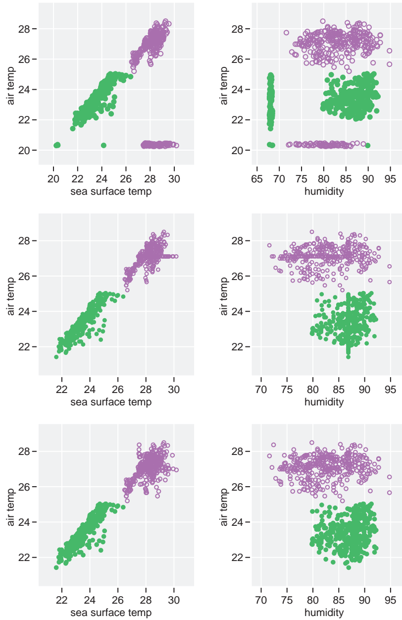
Fig. 3.5. Comparison of simple, widely used imputation schemes. Missings in the margin, as in Fig. 3.1 ( Top row ). Missing values have been replaced with variable means, conditional on year , producing vertical and horizontal stripes in each cluster ( Middle row ). Missing values have been filled in by randomly selecting from the recorded values, conditional on year ( Bottom row ). The imputed values are a little more varied than the recorded data.
