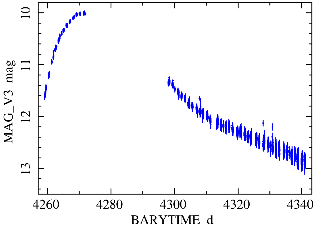
Figure 20: OMC light curve of the supernova SN2011fe discovered in M101 on August 24th, 2011. Time is in INTEGRAL Barycentric Julian days (Credits: OMC Team)
