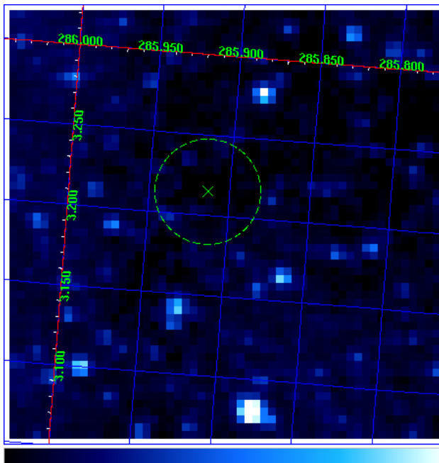
Figure 5: This image corresponds to the High Mass X-ray Binary 4U 1901+03, which generated a mosaic of 5x5 OMC sub-windows (16'x16'). The green cross and circle are, respectively, the position and positional error of 4U 1901+03 in the IBIS catalogue.
