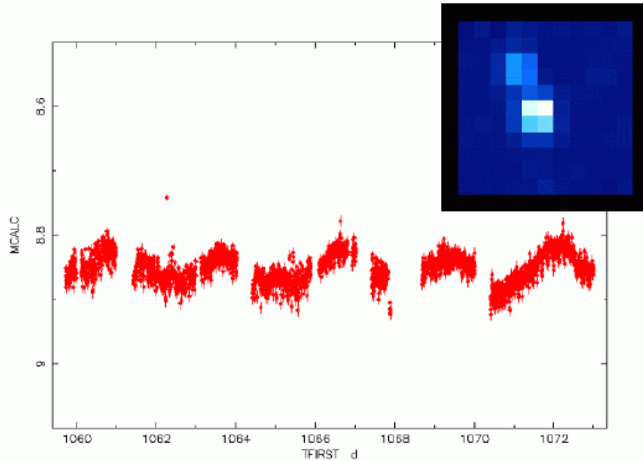
Figure 14: OMC light curve of high-mass X-ray binary Cygnus X-1 obtained using single exposures of 10 and 30 s. The OMC sub-window for this source is shown on the upper right corner of the graph. Time is in INTEGRAL Julian days. (Credits: OMC Team)
