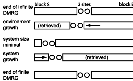
FIG. 3. Finite-system DMRG algorithm: block growth and shrinkage.
