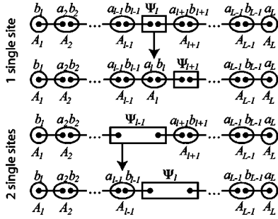
FIG. 6. Pictorial representation of S \bullet E (above) and S \bullet \bullet E (below) DMRG schemes for open boundary conditions as introduced by Verstraete, Porras, and Cirac, 2004. Paired dots represent auxiliary state spaces linked to a local state space. Straight lines symbolize maximal entanglement, ellipses and rectangles map to local state spaces as detailed in the text. Note the special role of the boundary sites. Adapted from Verstraete, Porras, and Cirac, 2004.
