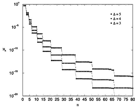
FIG. 9. Density-matrix eigenvalues w_n vs eigenvalue number n for a gapped XY Heisenberg chain of L=98 and three values of anisotropy \Delta > \Delta_c=1 . Degeneracies are as predicted analytically. From Peschel, Kaulke, and Legeza, 1999. Reprinted with permission.
