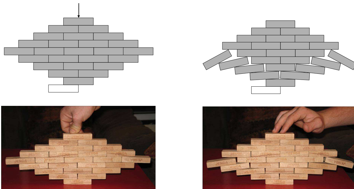
Figure 5: The instability of a 5-diamond in theory and practice.
