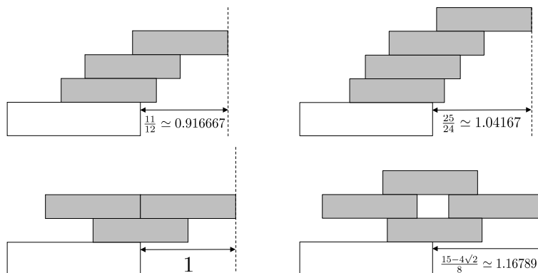
Figure 1: Optimal stacks with 3 and 4 blocks, compared to the corresponding harmonic stacks. The 4-block solution is from [1]. Like the harmonic stacks it can be made stable by minute displacements.
