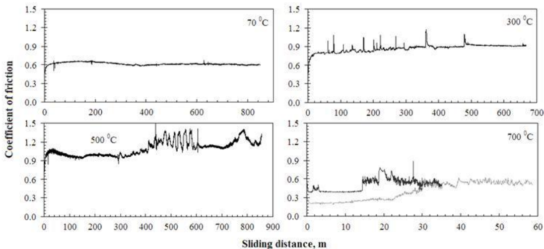
Figure 3 Friction coefficient curves at various testing temperatures.
