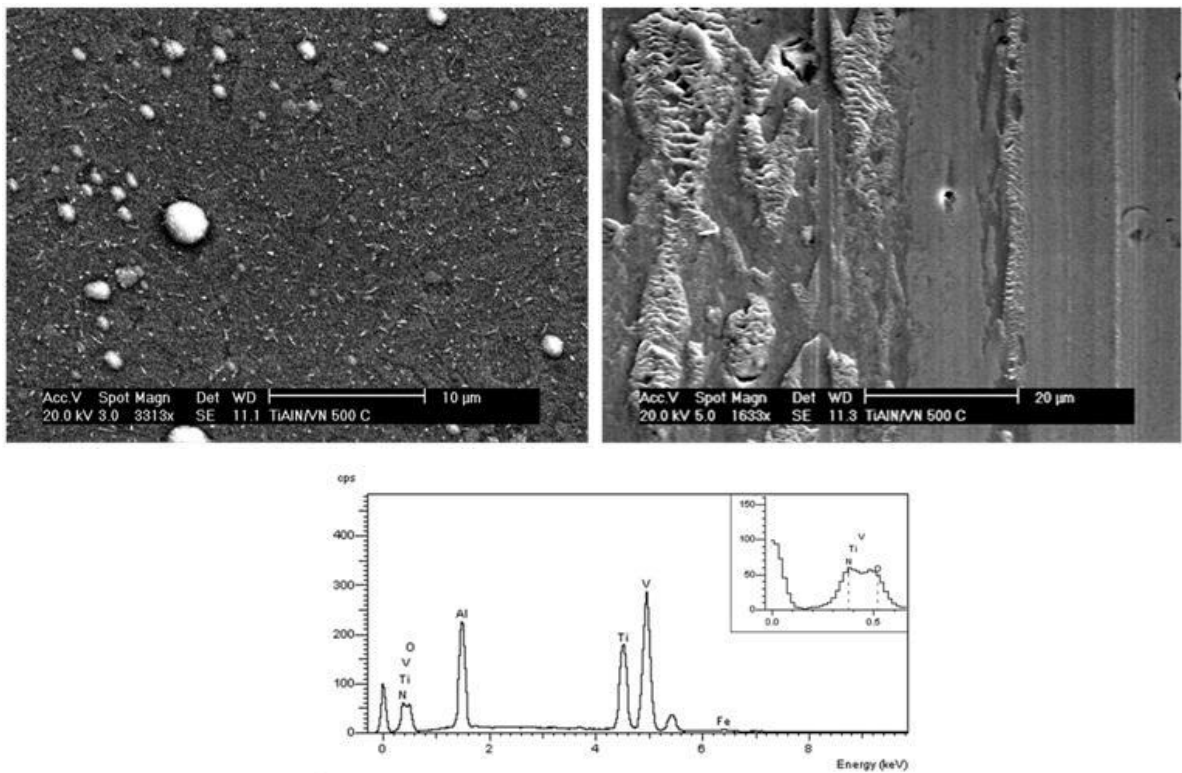
Figure 11 SEM and EDX analysis of the TiAlN/VN coating after the 500 °C wear test. (a) The un-tested area shows generally the as-deposited surface morphology in addition to the dispersed needle-like fine particles of initial oxidation product. (b) The worn surface shows both smooth area (on the right hand side) and transferred wear debris or thick tribofilm (fish-scale like patterns on the left hand side). (c) An EDX spectrum of the tribofilm shows the coexistence of oxygen and nitrogen, indicative of tribo-oxidation.
