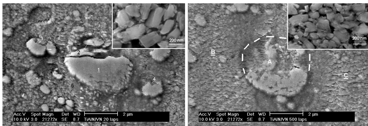
Figure 5 Mechanical wear and tribofilm generation of the TiAlN/VN coating observed after sliding wear at room temperature. (a) After 20 cycles of sliding, a large defect grain in the middle of the imaged area (labelled 1) shows surface flattening and spalling wear (labelled 2). Two smaller sized defect grains also show spalling wear (labelled 3 and 4). The fish-scale-like patterns, labelled 5 - 8, indicate initial form of tribofilm. The insert in the upper-right corner shows initial wear particles extrapped along the wear track edge. (b) A large defect grain (labelled A) observed on the 500-cycle wear track had been mostly worn by spalling. The remaining area (labelled B and C) is full of fish-scale like patterns indicating the developing tribofilm. The insert in the upper-right corner indicates reduced wear particle size after longer period of sliding wear.
