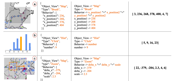
Fig. 2. Examples the encoding process of (a) Brush, (b) Click, and (c) Zoom. These interactions are examples of interactions in Table. 1. They are converted to JSON representations, then to CFG Parsed Tree, and then to numerical vectors based on the rules generated by CFG Tree. the same rule-governed format since the method is conducted over the whole dataset. The parsed-tree consists of the following keys:
