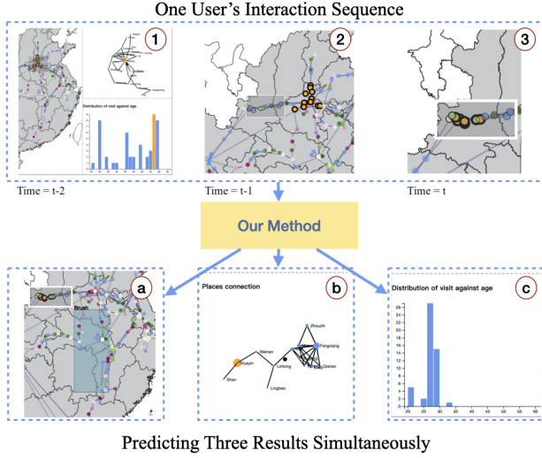
Fig. 6. One example of recommendation results of one input sequence of interaction logs. ①click a column on the Histogram View ②brush an area on the Map View ③zoom into an area on the Map View, compose a sequence of user interactions and the corresponding visual states. @brush on the Map View @click on the Force-Directed View @click on the Histogram View are the recommendations given by our model.
