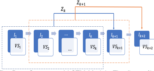
Fig. 3. The Data Structure of LSTM Model. The first k {Interaction, Visual States} are sequenced together to form an input value Z_k , and the corresponding label value is the next interaction I_{k+1}
