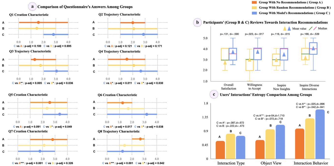
Fig. 7. Data Insights. Questionnaire Rating (a) shows the distribution of the acceptance degree of insight statements, with the results of paired t -tests' p -value between our model and two control groups (*, ** and *** denote p < .05 , .01 and .001 , respectively). The higher degree of acceptance of the correct statement (Q1-Q6), the better the data insight obtained by the user. 5-Points Likert Scales (b) shows users' reviews of random recommendations and our model's recommendations. Bar Chart (c) shows user's interactions' entropy in the aspect of interaction types, object views, and interaction behaviors among three different groups, along with the results of t -tests.
