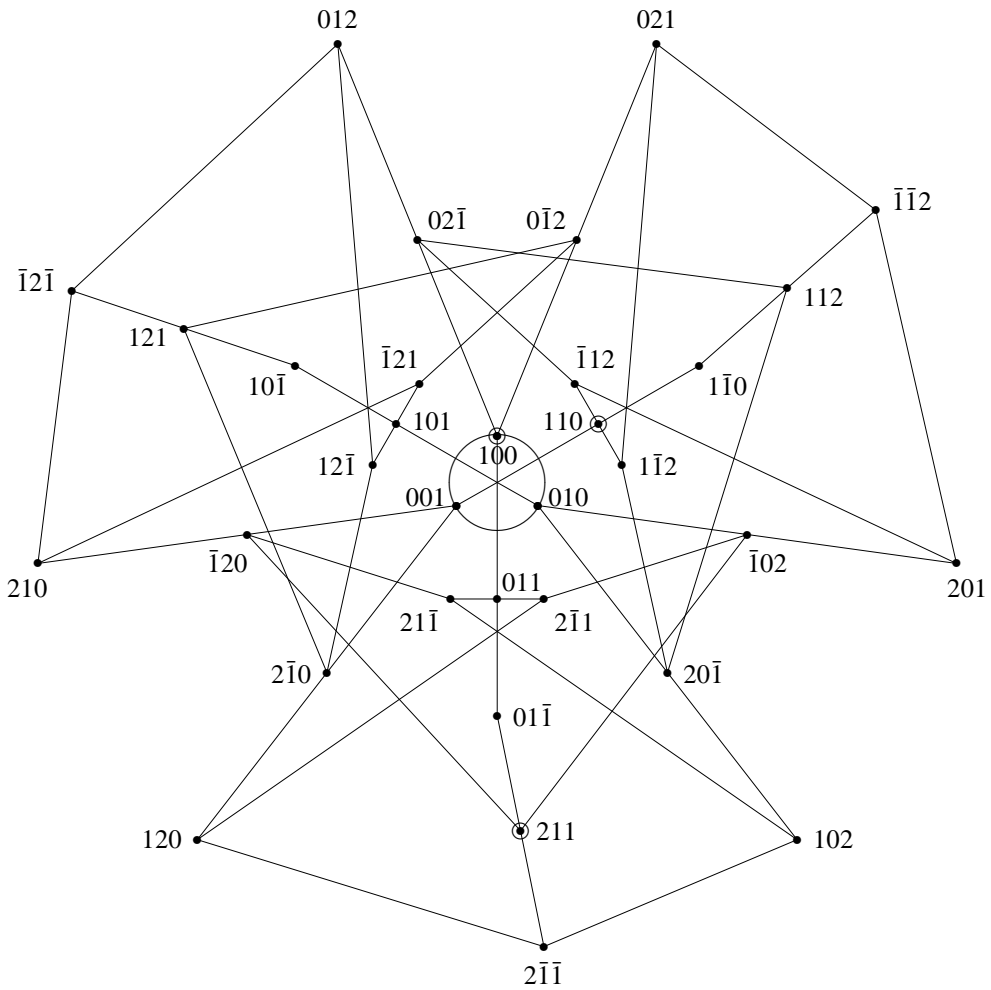
Figure 9: ‘Almost’ Greechie diagram of a suborthoposet of H_3 without any two-valued state (e.g. 1\bar{1}2 denotes \text{Sp}(1, -1, \sqrt{2}) ).
