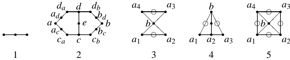
Figure 2: Greechie diagrams of orthomodular posets with finite 3-atomic blocks demonstrating differences of state spaces (a \ominus b denotes the diagram 2).
