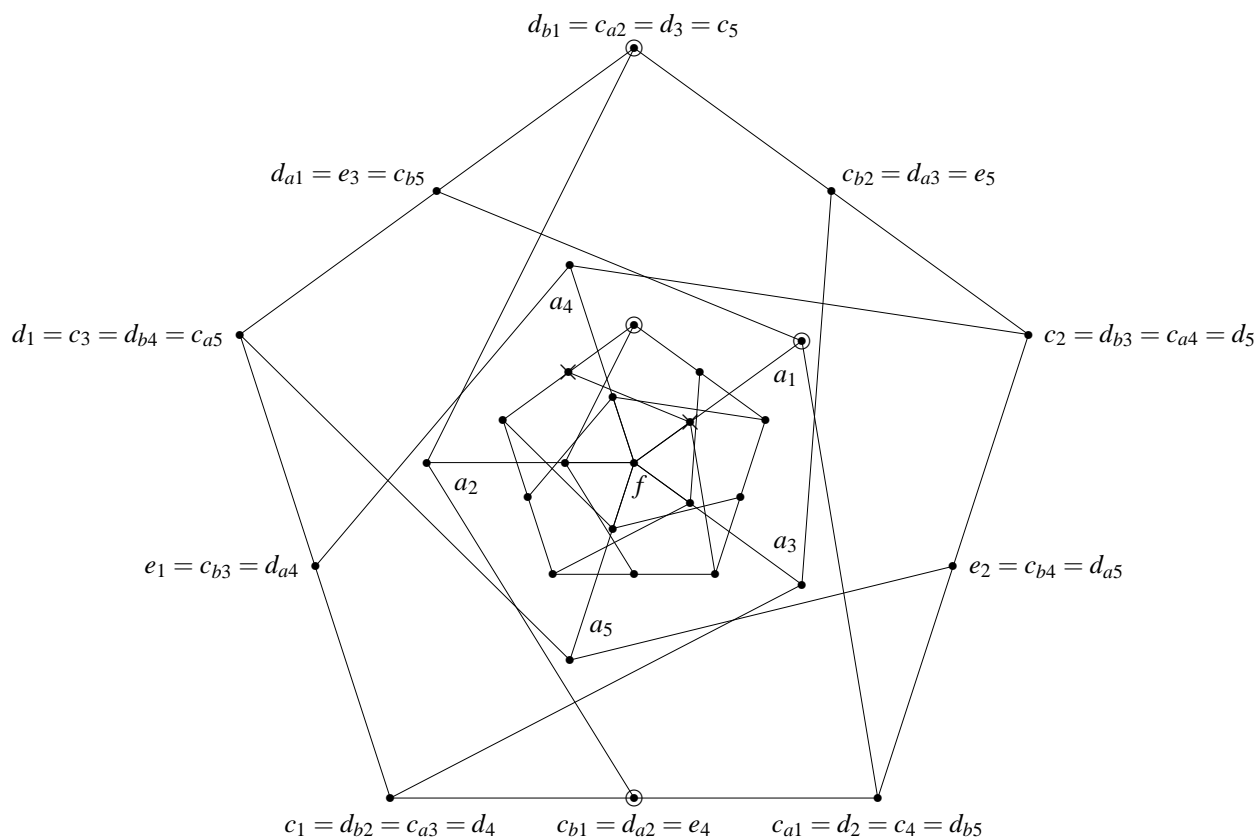
Figure 8: ‘Almost’ Greechie diagram of a suborthoposet of H_3 without a unital set of two-valued states.
