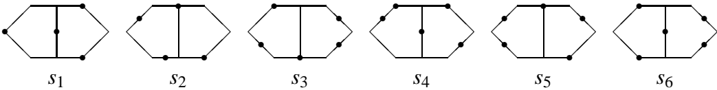
Figure 3: Separating set of two-valued states on an orthomodular lattice from Fig.2.2. (only atoms in which the corresponding state is equal to 1 are marked).
