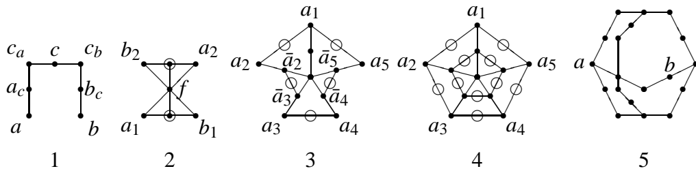
Figure 7: Greechie diagrams of orthomodular lattices weakly realizable in H_3 .
