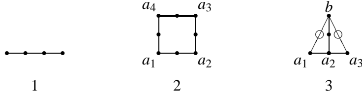
Figure 6: Greechie diagrams of some orthomodular posets nonrealizable in H_3 ( a \bullet \ominus \bullet b is an abbreviation of the Greechie diagram in Fig. 2.2.).
