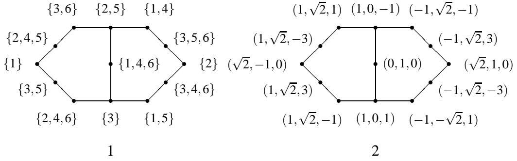
Figure 4: Various representations of an orthomodular lattice from Fig. 2.2.
