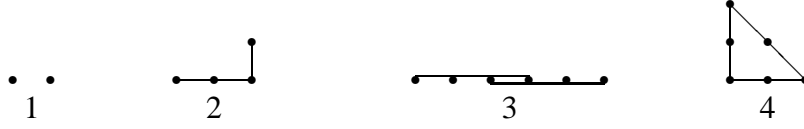
Figure 1: Examples of diagrams which are not Greechie diagrams.
