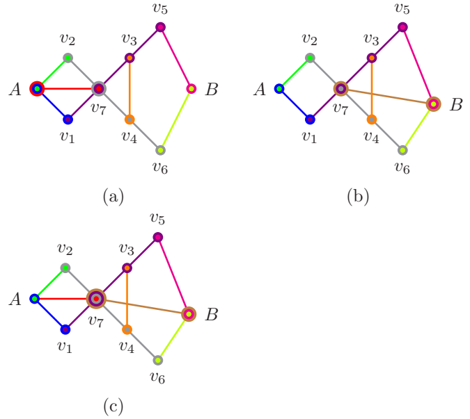
FIG. 4. (a)–(c) Greechie orthogonality diagrams of the three minimal TIFSs in d = 4 . The one in (a) appears in Hardy’s proof of Bell’s theorem [22] (see details in Refs. [32,35,37]).
