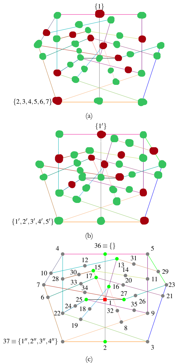
FIG. 2. (a) TIFS cloud, and (b) TTTS cloud with only a single overlaid classical value assignment if the system is prepared in state |1\rangle (Svozil 2018b). (c) The combined cloud from (a) and (b) has no value assignment allowing 36 = \{\} to be true/1; but still allows 8 classical value assignments enumerated by Table I, with overlaid partial coverage common to all of them. A faithful orthogonal realization is enumerated in Ref. (Abbott et al 2015, Table. 1, p. 102201-7).
