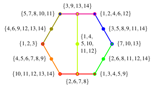
FIG. 1. The convex structure of classical probabilities in this (Greechie) orthogonality diagram representation of the Specker bug quantum or partition logic is reflected in its partition logic, obtained through indexing all 14 two-valued measures, and adding an index 1 \leq i \leq 14 if the i th two-valued measure is 1 on the respective atom. Concentrate on the outermost left and right observables, depicted by squares: Positivity and convexity requires that 0 \leq \lambda_i \leq 1 and \lambda_1 + \lambda_2 + \lambda_3 + \lambda_7 + \lambda_{10} + \lambda_{13} \leq \sum_{i=1}^{14} \lambda_i = 1 . Therefore, if a classical system is prepared (a generalized urn model/automaton logic is “loaded”) such that \lambda_1 + \lambda_2 + \lambda_3 = 1 , then \lambda_7 + \lambda_{10} + \lambda_{13} = 0 , which results in a TIFS: the classical prediction is that the latter outcome never occurs if the former preparation is certain.
