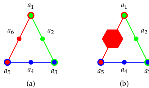
Figure 3. Greechie orthogonality hypergraph (a) of the scheme of a true implies true gadget realizable by a partition logic but not as a faithful orthogonal representation in 3-dimensional Hilbert space (in three-dimensional Hilbert space all three “inner” vertices a_2, a_4 and a_6 would “collapse” into any of the three “outer” vertices a_1, a_3 or a_5 ): suppose a_1 = 1 ; then, according to the admissability axioms WAD1&WAD2, a_3 = a_5 = 0 and thus a_4 = 1 . (b) To achieve a faithful orthogonal representation one could modify this triangular scheme by following Kochen and Specker ([ \Gamma_1 , p. 68 in [122]): they substituted one of the three contexts, say \{a_5, a_6, a_1\} , by a Specker bug which also provides a “true implies false” property at its terminal vertices a_1 and a_5 , and thereby acts just as admissability rule WAD1.
