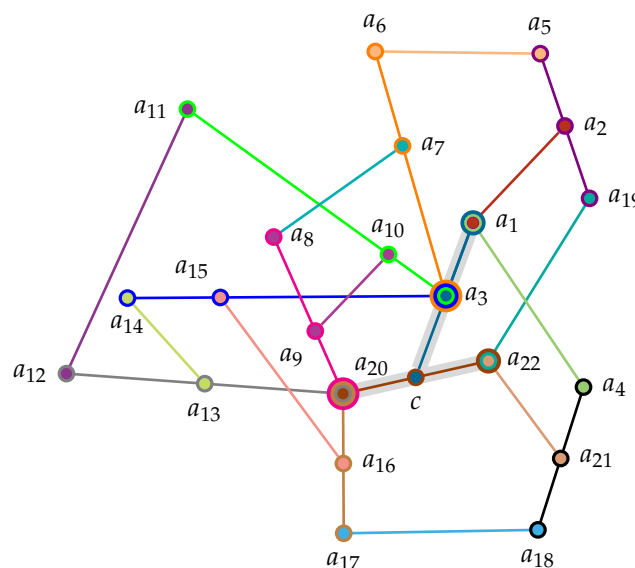
Figure 2. Greechie orthogonality hypergraph [148] (some observables which are not essential to the argument are not drawn) from proof of Theorem 3 in Ref. [119]. The advantage of this true-implies-false gadget is a straightforward parametric faithful orthogonal representation allowing angles 0 < \angle_{a_1, a_{22}} \leq \frac{\pi}{4} radians ( 45^\circ ) of, say, the terminal points a_1 and a_{22} . The corresponding logic including the completed set of 34 vertices in 21 blocks is set representable by partition logics because the supported 89 two-valued states are (color) separable. It is not too difficult to prove (by contradiction) that say if both a_1 as well as a_{22} are assumed to be 1, then a_2, a_3, a_4 , as well as a_{19}, a_{20} and a_{21} should be 0. Therefore, a_5 and a_{18} would need to be true. As a result, a_6 and a_{17} would need to be false. Hence, a_7 as well as a_{16} would be 1, rendering a_8 and a_{15} to be 0. This would imply a_9 as well as a_{14} to be 1, which in turn would demand a_{10} and a_{13} to be false. Therefore, a_{11} and a_{12} would have to be 1, which contradicts the admissibility rules WAD1&WAD2 for value assignments. It is also a true-implies-true gadget for the terminal points a_1 - a_{20} .
