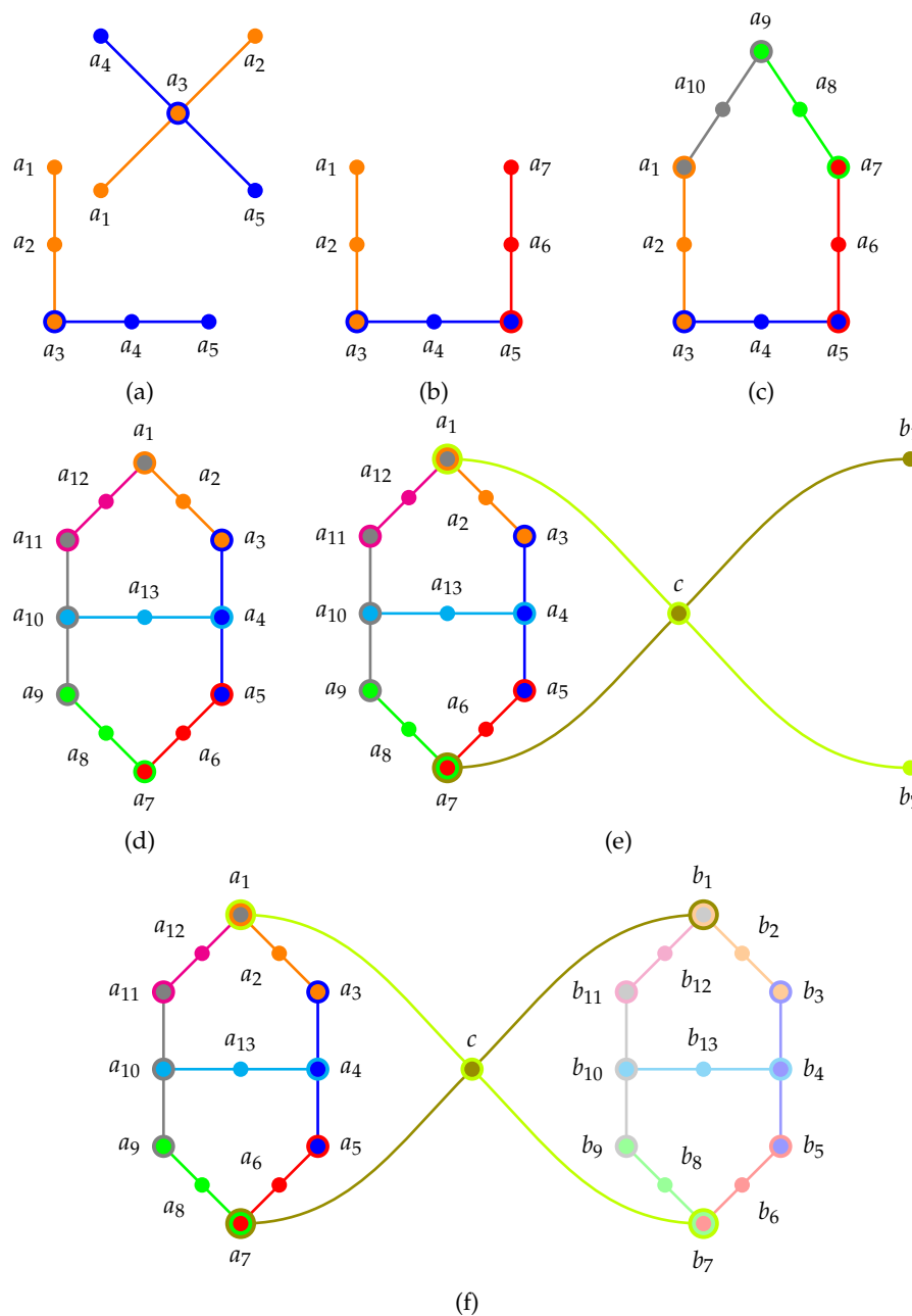
Figure 1. Greechie orthogonality hypergraphs representing historic configurations of complementary observables arranged in 3-element blocks. (a) Two renditions of the firefly gadget; (b) Two firefly gadgets with a common block; (c) house/pentagon/pentagram gadget; (d) Specker bug/cat’s cradle logic; (e) extended Specker bug logic with a 1-1/true-implies-true property; (f) combo of interlinked Specker bugs with a non-separable set of two-valued states (at a_1 - b_1 as well as a_7 - b_7 ).
