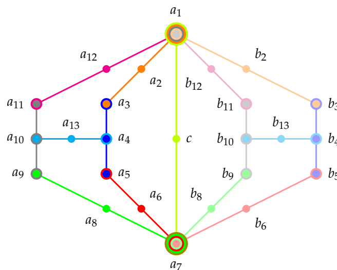
Figure 5. Greechie orthogonality hypergraph of the classical remainder of a combo of interlinked Specker bugs with a non-separable set of two-valued states depicted in Figure 1f.
