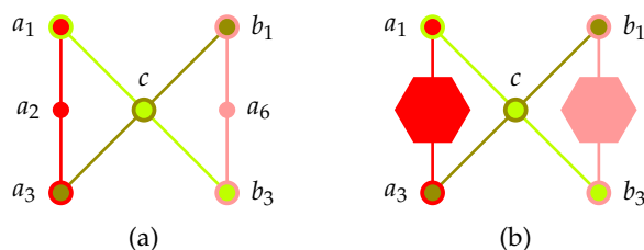
Figure 4. Greechie orthogonality hypergraph (a) of the scheme of a logic with a nonseparable set of two-valued states not as a faithful orthogonal representation in 3-dimensional Hilbert space: suppose a_1 = 1 ; then, according to the admissability axioms WAD1&WAD2, a_3 = b_3 = c = 0 and thus b_1 = 1 (and, by symmetry, vice versa: B_1 = 1 implies a_1 = 1 ). (b) To achieve a faithful orthogonal representation one could modify this bowtie scheme by following Kochen and Specker ( \Gamma_3 , p. 70 in [122]): they substituted two of the four contexts \{a_1, a_2, a_3\} and \{b_1, b_2, b_3\} by Specker bugs which also provide a “true implies false” property at their terminal vertices a_1 and a_3 , as well as b_1 and b_3 , respectively, and thereby act just as admissability rule WAD1.
