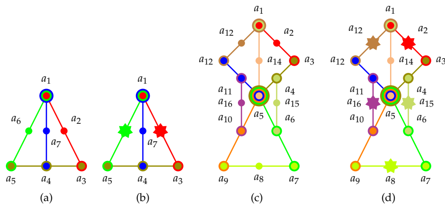
Figure 6. Greechie orthogonality hypergraph schemes of observables with non-unital sets of two-valued states with impossible or unknown faithful orthogonal representations (a) simplest scheme without a faithful orthogonal representation: if v(a_1) = 1 then v(a_3) = v(a_4) = v(a_5) = 0 which contradicts admissibility rule WAD1; (b) the same as in (a) but with a_2 and a_6 substituted by a “true-implies-false gadget” (for example, the Specker bug gadget is taken in Figures 2.4 and 6.3 of Ref. [35]); (c) another scheme for a logic with a non-unital set of two-valued states: if v(a_1) = 1 then v(a_3) = v(a_5) = v(a_{12}) = 0 ; therefore v(a_4) = v(a_{11}) = 0 ; and therefore v(a_6) = v(a_{10}) = 0 and v(a_7) = v(a_9) = 1 which contradicts admissibility rule WAD2; (d) the same as in (a) but with a_2 and a_6 substituted by a “true-implies-false gadget” (for example, the Specker bug gadget is taken in Figure 7.3 of Ref. [35]).
