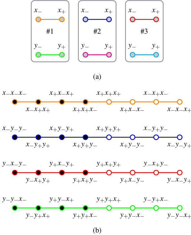
Fig. 1 Hypergraphs representing (a) the six disconnected classical single-particle contexts representing the observables of the first, second, and third particle, respectively; (b) four isolated, nonintertwining contexts, with eight atoms each, employed in the GHZ argument (there are eight contexts in total, but only half of them are considered). Filled circles indicate states which are classically allowed in a modified GHZ game requesting negativity for all products xyy = yxy = yyx = xxz = -1 . Every column represents a viable noncontextual winning strategy.
