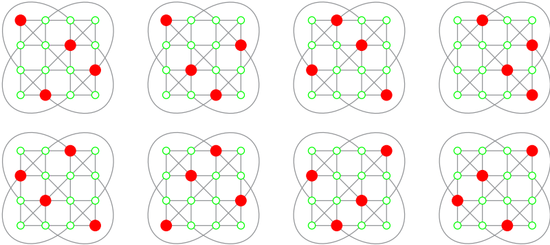
Fig. 4 Enumeration of the eight two-valued states of the “tightened” GHZ logic.
