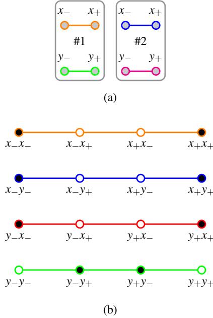
Fig. 5 Hypergraphs representing (a) the four disconnected classical single-particle contexts—two contexts per particle—representing the observables of the first and second particle, respectively; (b) the four separated, nonintertwined two-partite contexts, with four atoms each, that are the Cartesian products of these single-particle contexts. Filled circles indicate states which are involved in a stranger-than-GHZ game requesting positivity for all products xx = xy = yx = +1 and negativity for yy = -1 .
