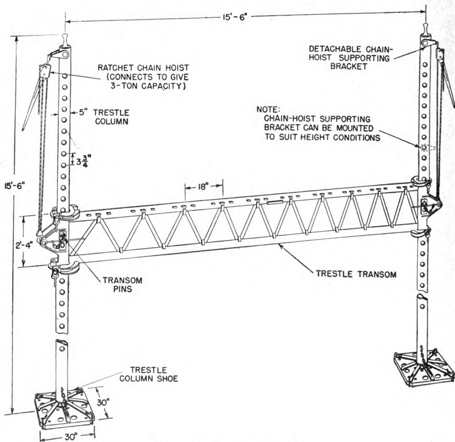
Figure 12. Assembled trestle.
