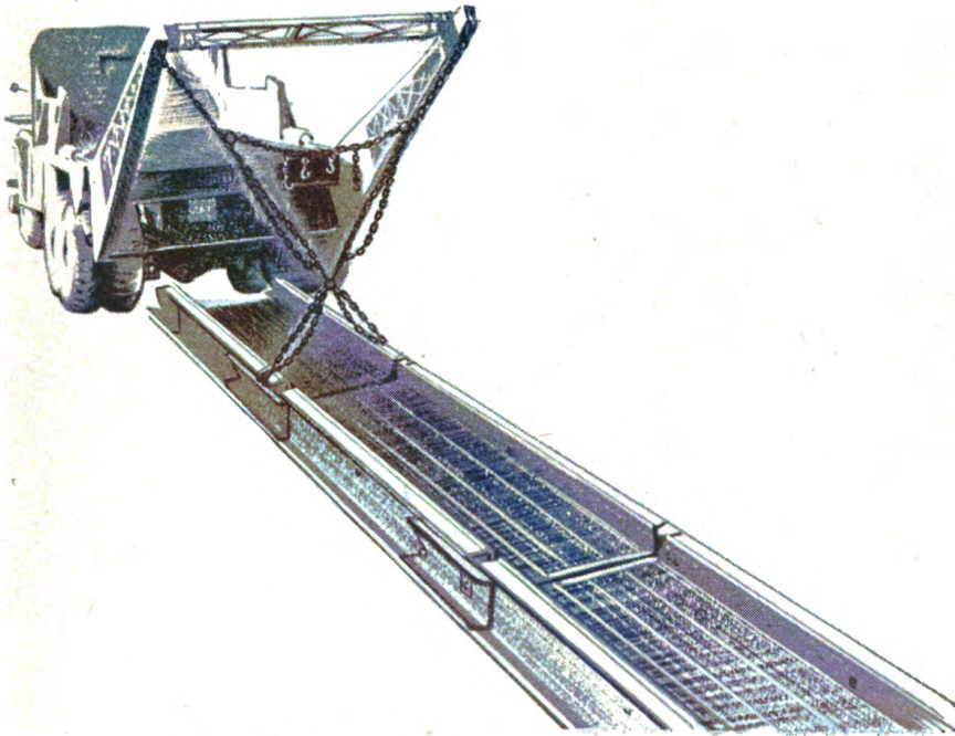
③ Handling treadways connected longitudinally.
