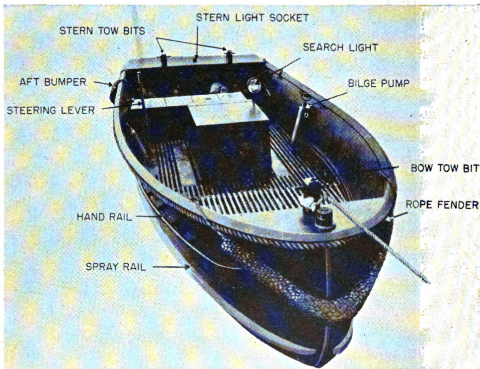
Figure 18. Power utility boat.
