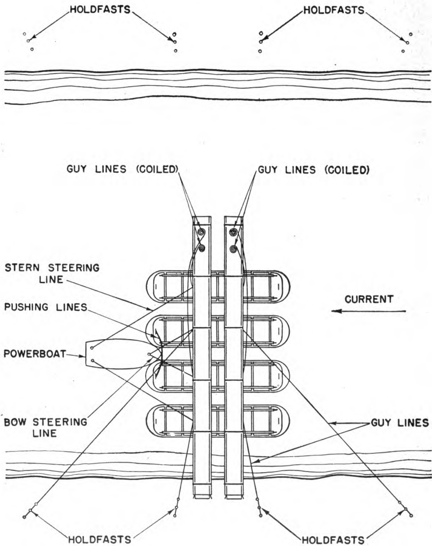
Figure 42. Arrangement of rigging for rafts.
