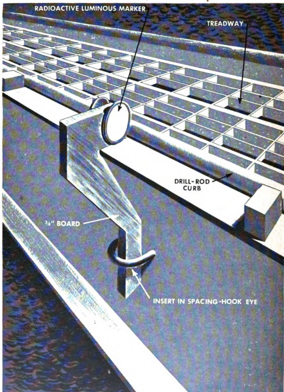
Figure 44. Method of attaching radioactive luminous marker on treadway.
