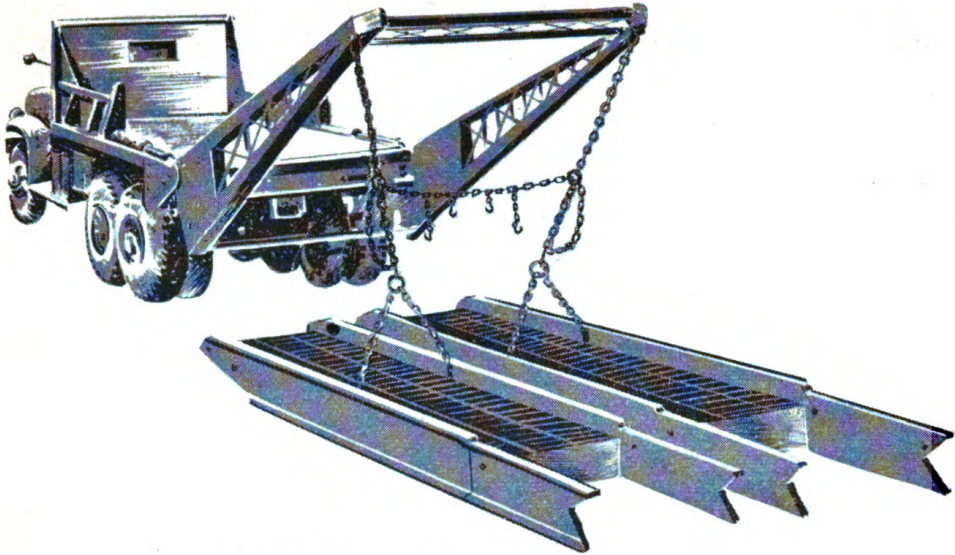
② Handling treadways in pairs.
