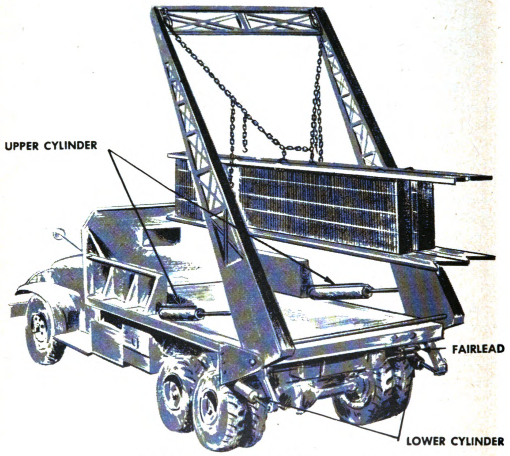
① Treadways being unloaded from truck. Figure 23. Operation of treadway truck.
