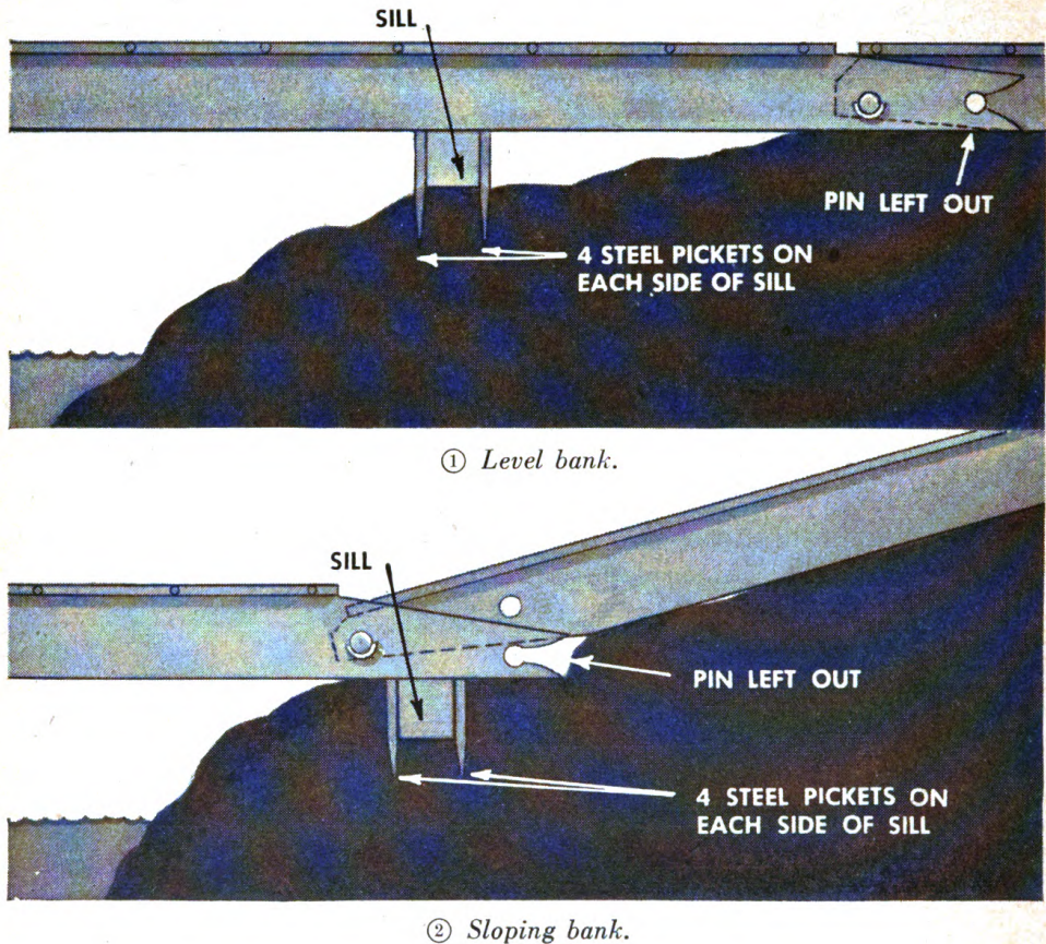
Figure 37. Shore connections without trestles.
