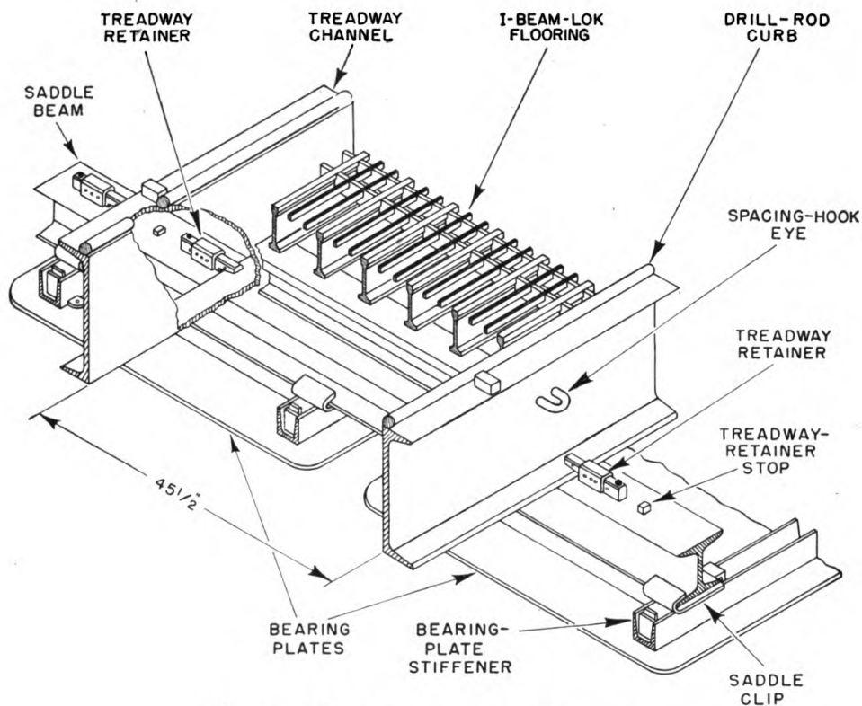
Figure 8. Assembly of treads on saddle.
