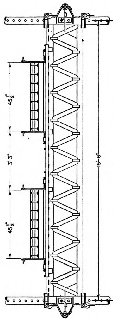
TREADWAYS IN PLACE ON TRESTLE Figure 13. Treadway adaptor.
