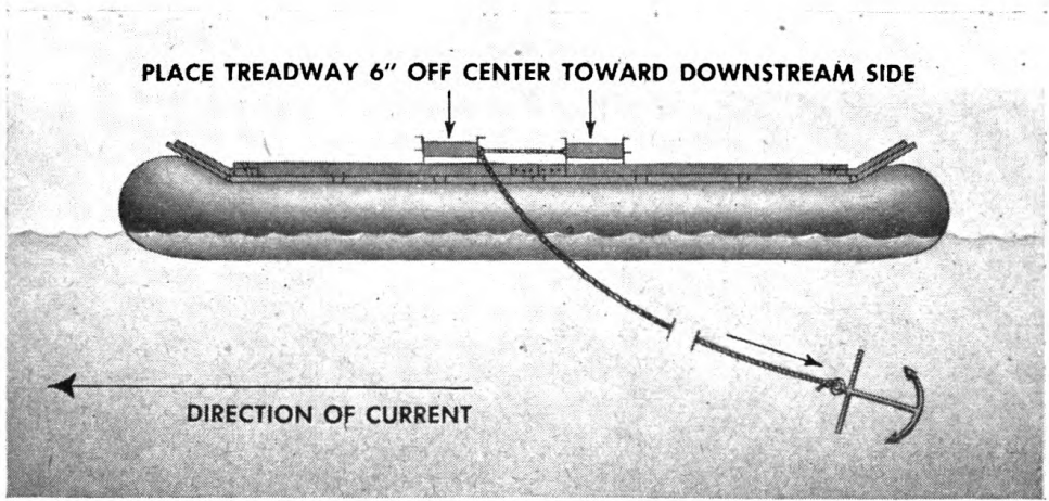
① Elevation.
