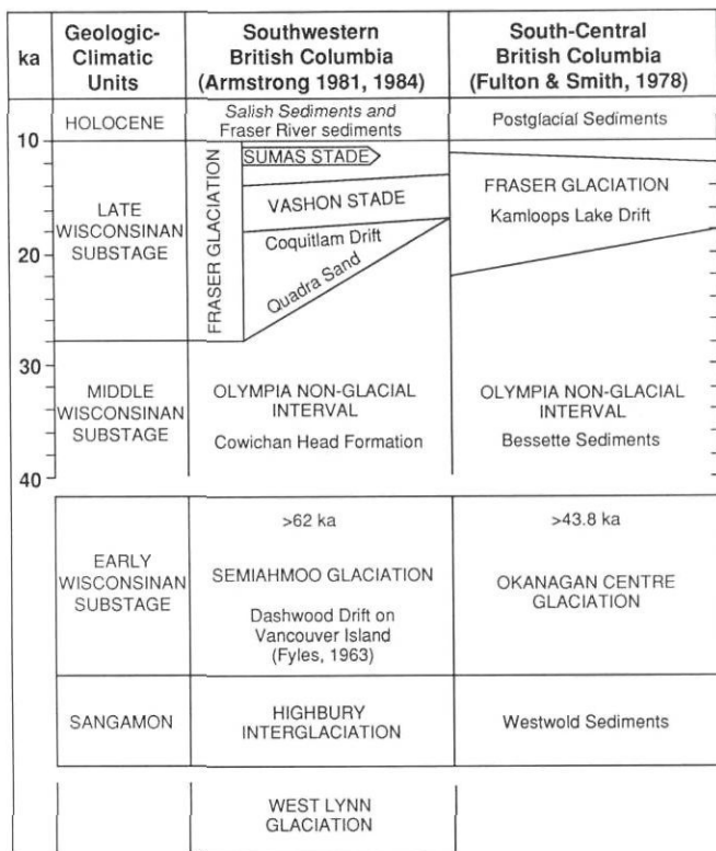
FIGURE 5. Quaternary events and stratigraphic units in southern and central British Columbia. Stratigraphic names are shown only where they differ from those of the glacial and non-glacial intervals.
