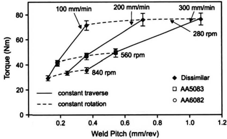
Figure 16: Variation of torque on the tool with weld pitch [111].
