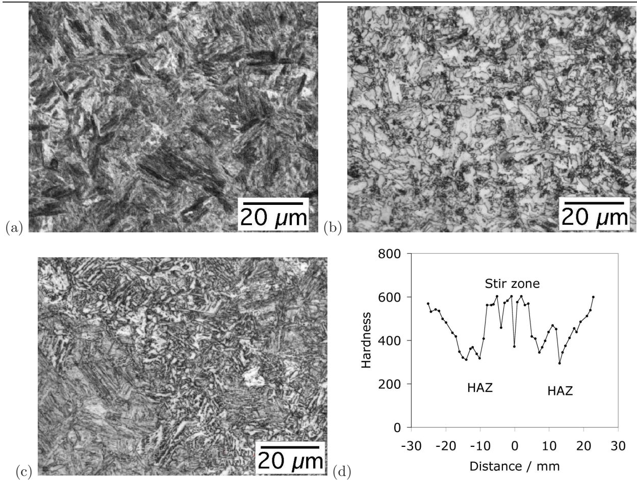
Figure 31: Typical microstructure of an FSW weld in a C–Mn steel (micrographs courtesy of P. Konkol [181]). (a) Tempered martensite in parent steel. (b) Mixed microstructure in the fine-grained HAZ. (c) Stir zone. (d) Hardness distribution.
