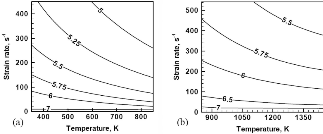
Figure 4: Computed contours of \log_{10}(\text{viscosity in Pa s}) [41] as a function of temperature and strain rate for (a) AA 6061-T6. (b) 1018 C-Mn steel.
