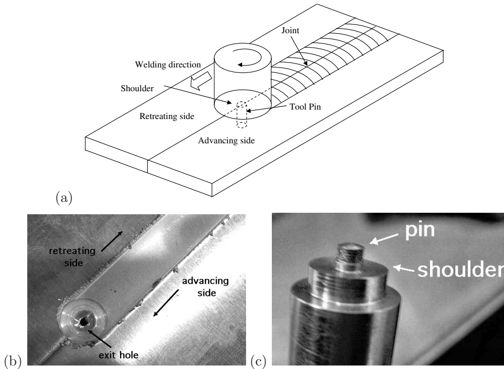
Figure 1: (a) Schematic illustration of the friction stir welding process. (b) An FSW weld between aluminium sheets. (c) An actual tool, with a threaded-pin.
