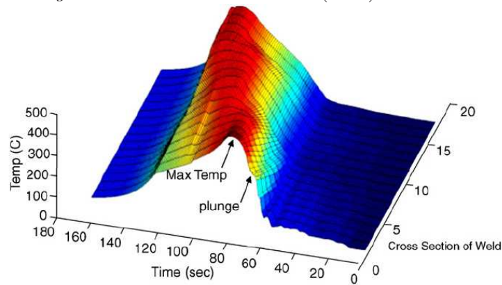
Figure 10: 3D plot of thermal cycles at the bottom surface along the weld centerline of AA 6061-T6 [97]. The thermal cycle at the front is for the location where tool pin is inserted into the workpiece while other thermal cycles correspond to locations along the weld centreline in the direction of tool movement.
