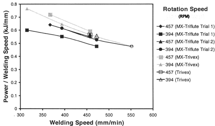
Figure 3: Heat input at various welding speeds used to weld 6.35 mm thick AA 7075-T7351 plates using MX-Triflute, MX-Trivex and Trivex tools [44].
