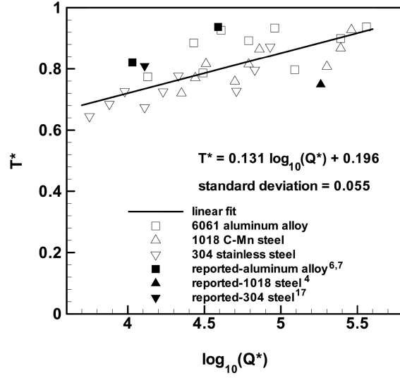
Figure 14: Variation of dimensionless peak temperature [102] with non-dimensional heat input.
