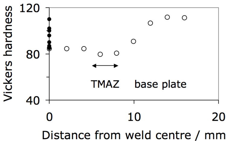
Figure 23: Open circles are data from friction stir weld, plotted relative to the centreline of the FSW for alloy AA2219 [149]; similar data have been reported by [150]. Filled circles from a variety of arc and electron-beam welds [148]. In the latter case all values are plotted at zero on the horizontal axis to represent the fusion zone.
