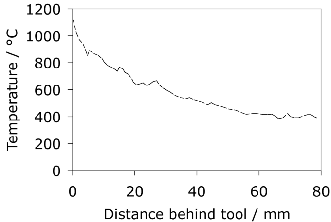
Figure 27: Temperature as a function of distance behind a tool after 250 mm of welding with the tool advancing at 3 \text{ mm s}^{-1} (after [176], for alloy 1 in Table 3).
