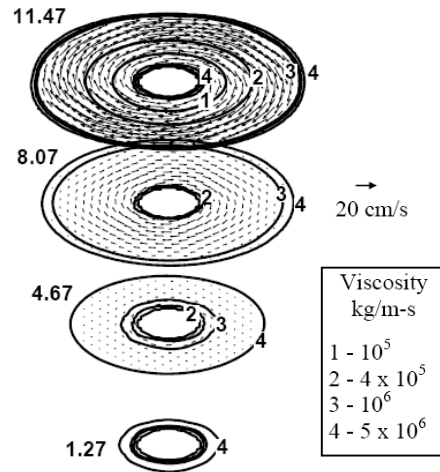
Figure 6: Spatial variation of viscosity and velocity in AA 6061-T6 [39] at planes corresponding to z = 1.27, 4.67, 8.07 and 11.47 mm for a plate thickness of 12.7 mm. Distances in x and y direction were equivalent, but that in the z -direction was increased eight fold to enhance clarity. The welding velocity was 1.59 \text{ mm s}^{-1} and the rotational speed was 637 \text{ rpm} .
