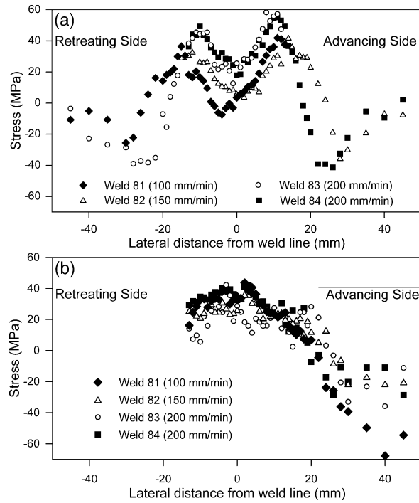
Figure 20: Measured (a) longitudinal x -direction and (b) the lateral y -direction stresses in AA5083 welds at different welding speeds across a transverse section [134].
