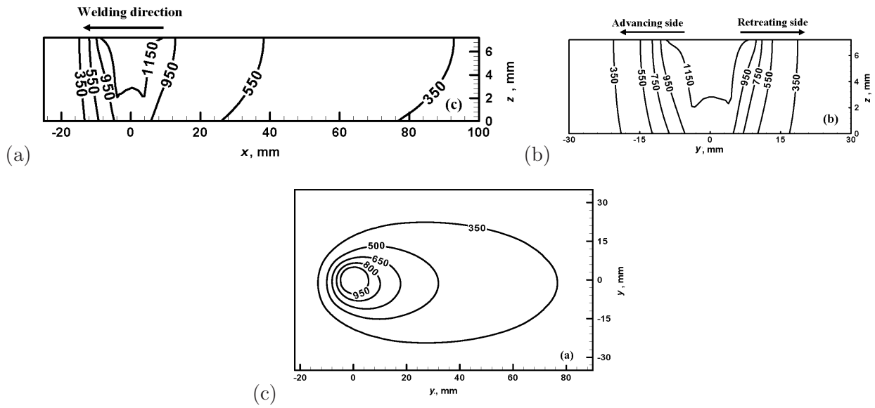
Figure 13: Computed temperature profiles (K) in (a) xz -plane, (b) yz -plane and (c) z -plane i.e top surface of 7.2 mm thick workpiece of Ti-6Al-4V alloy welded with translational speed of 1.6 mm/s and rotational speed of 275 rpm. [72].
