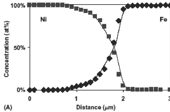
Figure 7: Concentration profiles of Fe and Ni at a location in stir region for FSW of pure Fe and Ni. Points represent data obtained by atomic emission spectroscopy and the solid lines indicate computed results. [78]
