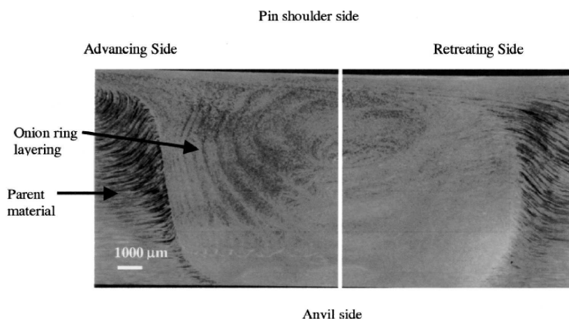
Figure 9: Optical image showing the macroscopic features [81] in a transverse section of a friction stir welded 2195-T81 Al-Li-Cu alloy. Note the onion ring and the adjacent large upward movement of material.
