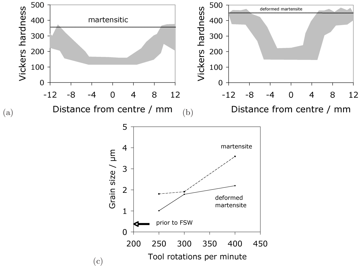
Figure 30: Hardness as a function of the distance from the FSW weld centreline; the horizontal line indicates the starting hardness. The upper limit of the shaded region corresponds to the slowest rotation speed and vice-versa. (a) Welded in the as-quenched martensitic state. (b) Welded after rolling the martensite to a 35% cold reduction. (c) Changes in the grain size within the stir zone. Adapted from [182].
