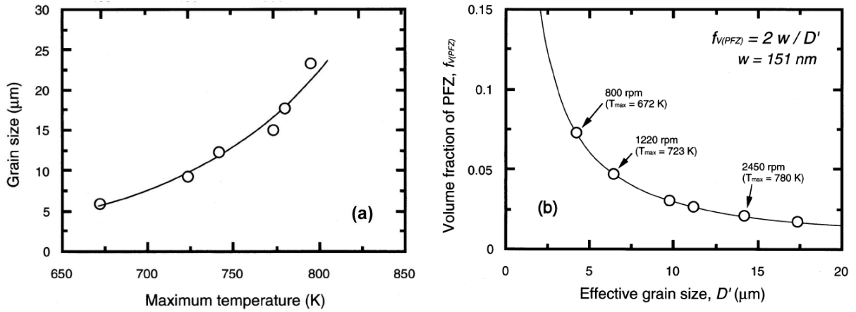
Figure 25: Relationship between (a) peak temperature and grain size in AA 6063 [110] and (b) grain size and volume fraction of PFZs.
