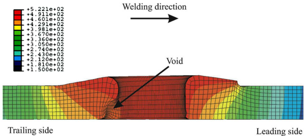
Figure 19: Void formation at the lower advancing side due to incomplete filling [36] modeled using ALE formulation of FEM. Temperature contours are shown in °C.
