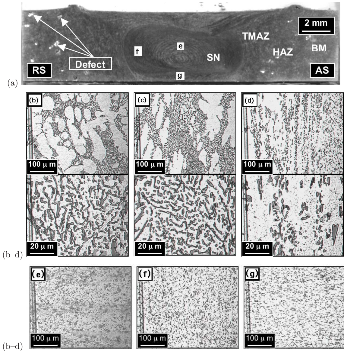
Figure 26: (a) A section through a friction stir weld made in an Al-Si casting alloy. There are pores indicated in the base metal (BM). HAZ represents the heat affected zone, TMAZ the thermomechanically affected zone, and SN the stir nugget. (b–d) Optical micrographs showing the microstructure in (b) the base metal; (c) heat-affected zone; (d) the thermomechanically affected zone, where considerable refinement of the silicon has occurred. (e–g) Optical micrographs of regions (e), (f) and (g) of the stir nugget as identified in macroscopic section presented above. Micrographs courtesy of Professor H. Fujii.
