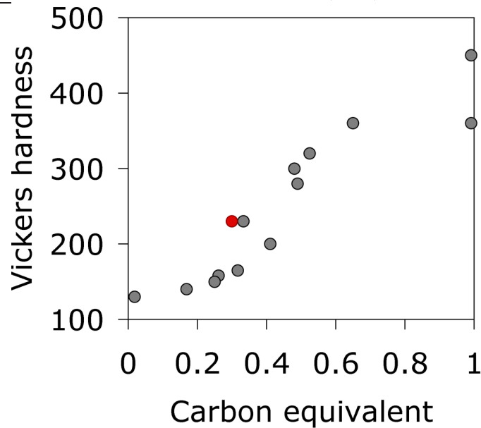
Figure 32: The Vickers hardness of the TMAZ as a function of the IIW carbon equivalent of the steel. The > 2.5 value of carbon equivalent corresponds to Alloy 1, Table 3.
