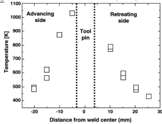
Figure 12: Peak temperature distribution along the intersection of horizontal midplane and transverse plane through the tool axis, for the FSW of 304L stainless steel using a tool rotational speed of 600 rpm and a welding speed of 10.2 mm/min. The tool shoulder and tool pin diameters were 25.4 and 5.6 mm, respectively. [4].
