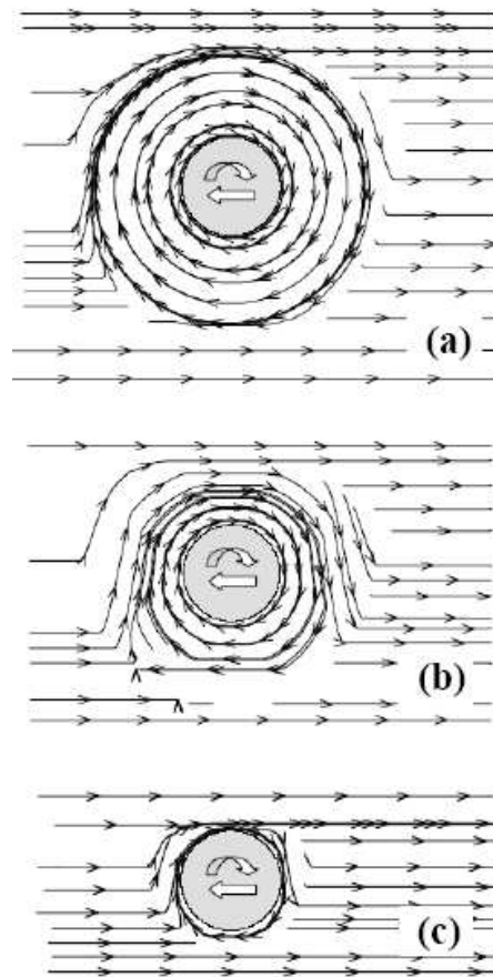
Figure 5: Stream traces on different horizontal planes (a) 0.35 mm, (b) 1.59 mm and (c) 2.28 mm below the top surface for a 304 stainless steel plate of thickness 3.18 mm. Welding speed 4 \text{ mm s}^{-1} with tool rotation at 300 rpm [40].
