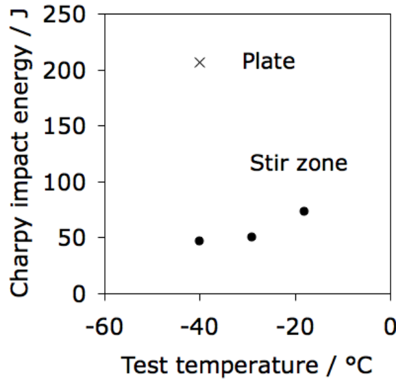
Figure 29: Charpy impact toughness of the stir zone of friction stir weld in HSLA65 steel [181].
