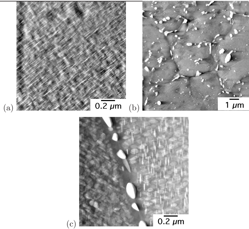
Figure 24: Microstructure variations across aluminium alloy AA2219 joined using friction stir welding. (a) Unaffected parent material in the precipitation hardened condition. (b) The nugget (c) The heat-affected zone. Micrographs courtesy of Dr Christian Paglia.
