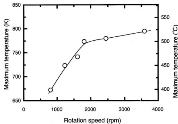
Figure 15: Relationship between rotational speed and peak temperature in FS-welds of AA 6063 [110]
