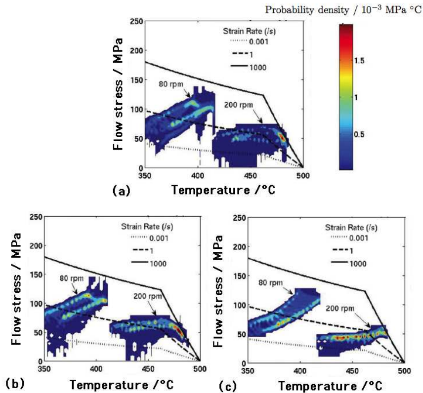
Figure 18: Material condition maps for a) Triflat, b) Trivex and c) Cylindrical tool pin at 80 and 200 rpm [124].
