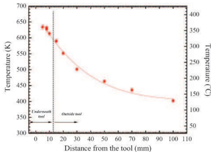
Figure 11: Instantaneous temperature distribution, measured using neutron-diffraction, on the top surface along the weld centerline behind the the tool pin, for FSW of AA 6061-T6 [98].
