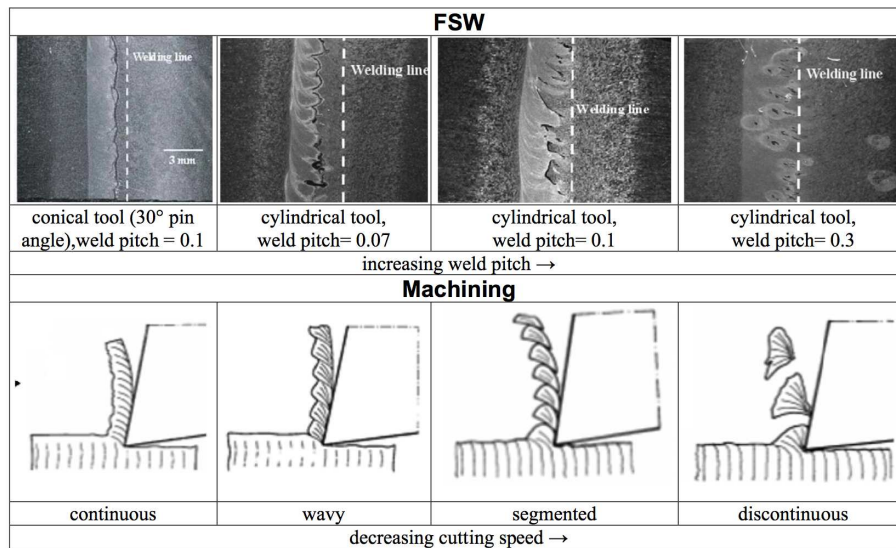
Figure 8: Analogy between chip morphology in machining and material flow in FSW [79]. Mid-plane horizontal sections of AA 7075-T6 show the re-distribution of copper about the center-line after welding when copper foil is placed between the plates to be welded. Tool was made of C40 Steel, with shoulder diameter of 12 mm. The cylindrical pin had a diameter of 3.0 mm while the conical pin had a major diameter equal to 5.00 mm and minor diameter of 1.90 mm and both were 2.70 mm in height (for the conical pin, this corresponds to cone angle 30°).
