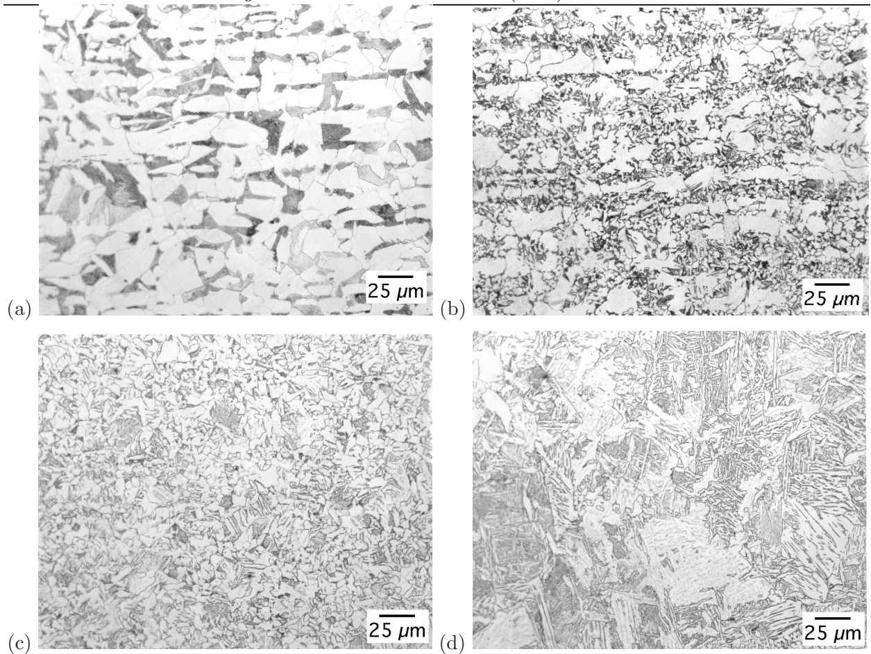
Figure 28: Typical microstructure of an FSW weld in a C–Mn steel (micrographs courtesy of P. Threadgill [177]). (a) Parent steel, with bands of allotriomorphic ferrite and pearlite. (b) Intercritically heated region of HAZ. (c) TMAZ (fine-grained region near stir zone). (d) Stir zone.
