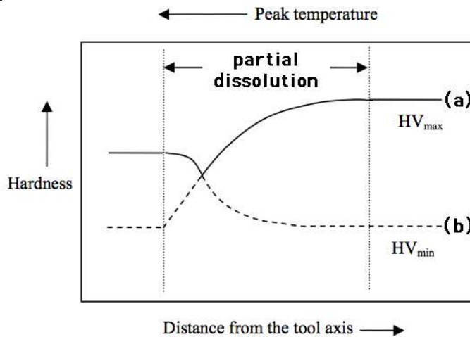
Figure 22: A schematic diagram showing dissolution and re-precipitation in age-hardenable aluminium alloys. HV denotes the Vickers hardness number. Adapted from [146].
