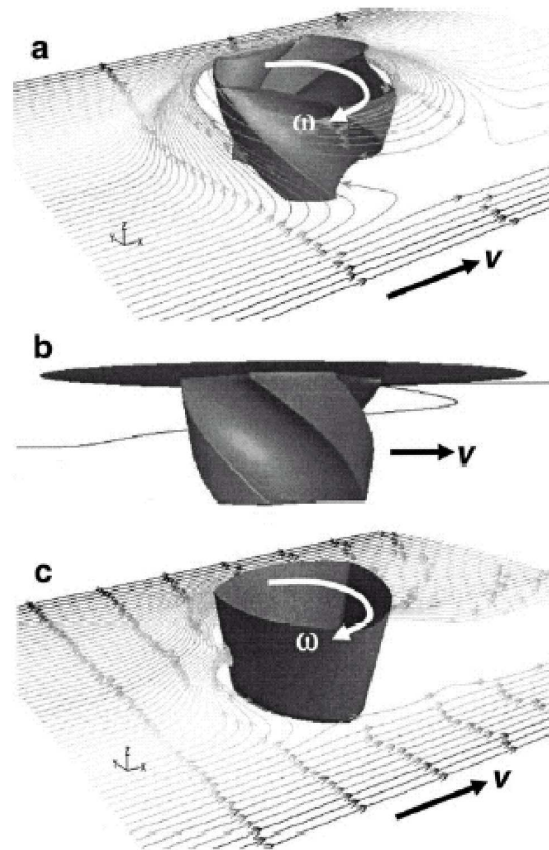
Figure 17: Streamlines for isothermal model [47] that used a limiting shear stress of 40 MPa: a) Triflute tool, b) single streamline for Triflute tool showing vertical movement and c) Trivex tool. Tool rotation 457 rpm and translation at 457 mm min -1 .
