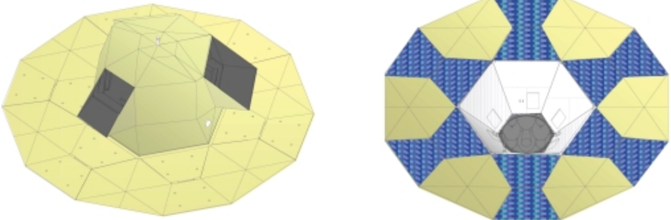
Figure 10: The GAIA satellite in orbit, with solar panels and sun shield deployed, viewed from above (left) and below (right). In the left figure, the entrance apertures of the telescopes can be seen, shielded from direct solar illumination by the solar array/sunshield assembly.
