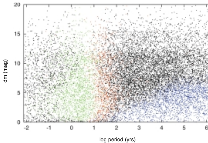
Figure 4: Simulated bright binaries (black) in a \log P versus \Delta m diagram. The other colours denote systems detected as non-single by GAIA: blue for resolved system, red for 'quadratic', and green for 'stochastic' proper motion deviations.
