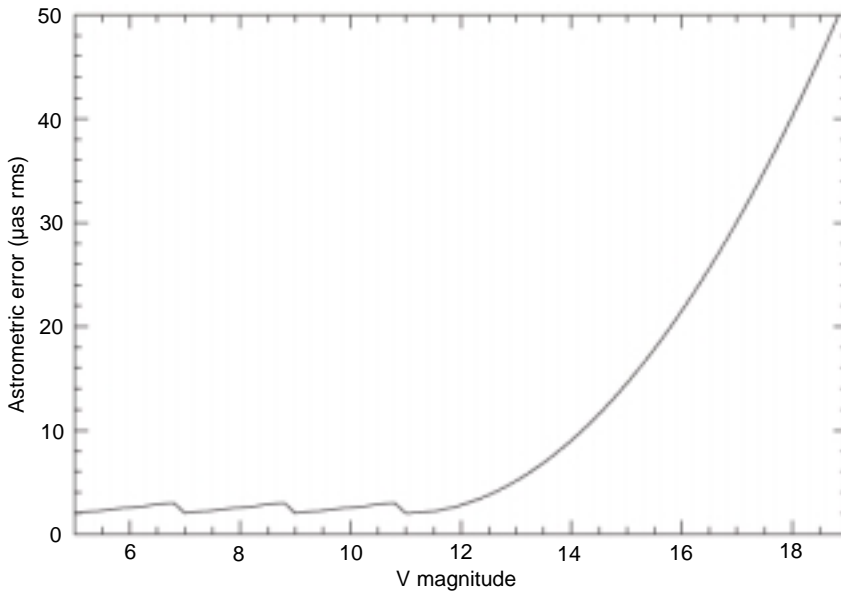
Figure 14: Nominal accuracy performance versus magnitude, for a G2V star. For V < 15 mag the astrometric performance improves because the number of detected photons increases until the detector saturation level is reached ( V \sim 11.6 mag for G2V star). Once saturation is reached, the performance is practically independent of magnitude.
