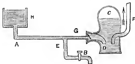
Fig. 2.—Whitehurst's Machine.
