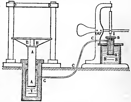
FIG. 2.—Hydraulic Press.
