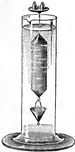
FIG. 1.—Nicholson's Hydrometer.
