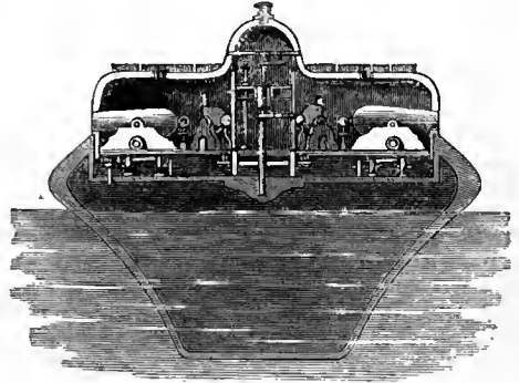
Fig. 7.—Timby's Revolving Turret.
