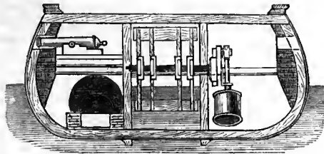
FIG. 2.—Demologos (section).
