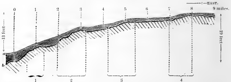
LEGEND.—0, Davenport Bridge; 1, Lower Chain; 2, Moline Chain; 3, Duck Creek Chain; 4, Winnebago Chain; a , surface of water; b , river bottom; horizontal scale, 1-142,560; vertical scale, 1-238.
