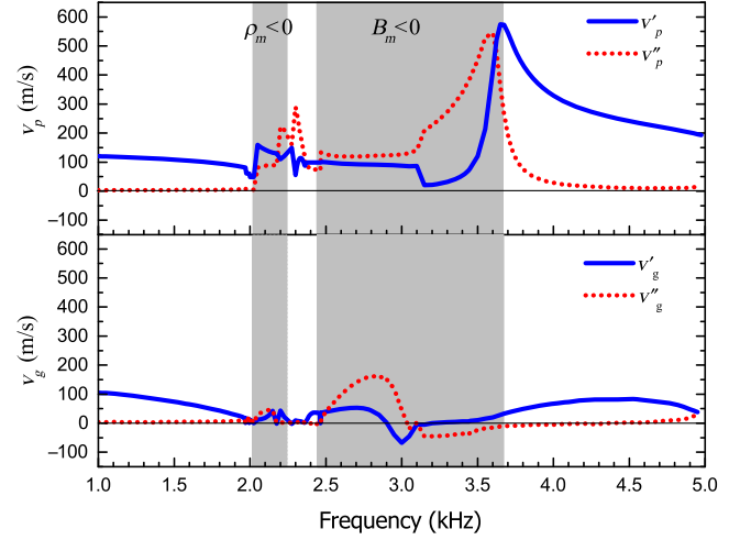
FIG. 5. Components of the extracted phase velocity ( v_p ) and group velocity ( v_g ) for the metamaterial where the viscothermal effects are considered. The shadowed zones define the regions where the metamaterial is single negative, according to the results shown in Fig. 2.
