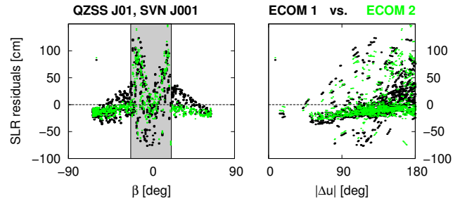
Fig. 9 SLR residuals of QZS-1 from 2014 as a function of the \beta -angle (left) and the argument of latitude \Delta u (right). Gray: orbit normal mode
