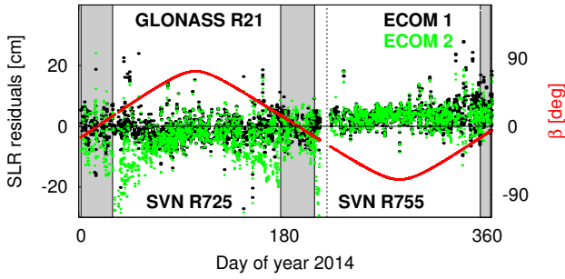
Fig. 6 SLR residuals of GLONASS R21 as a function of time. SVN R725 was replaced by SVN R755 on 02 Aug 2014. Gray: eclipse seasons. Red: \beta -angle
