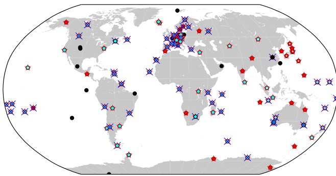
Fig. 2 Distribution of GNSS tracking stations contributing to the CODE MGEX orbit solution on DOY 30/2015. Black dots: GPS. Red stars: GLONASS. Cyan stars: Galileo. Black X-es: BeiDou. Small white dots: QZSS
