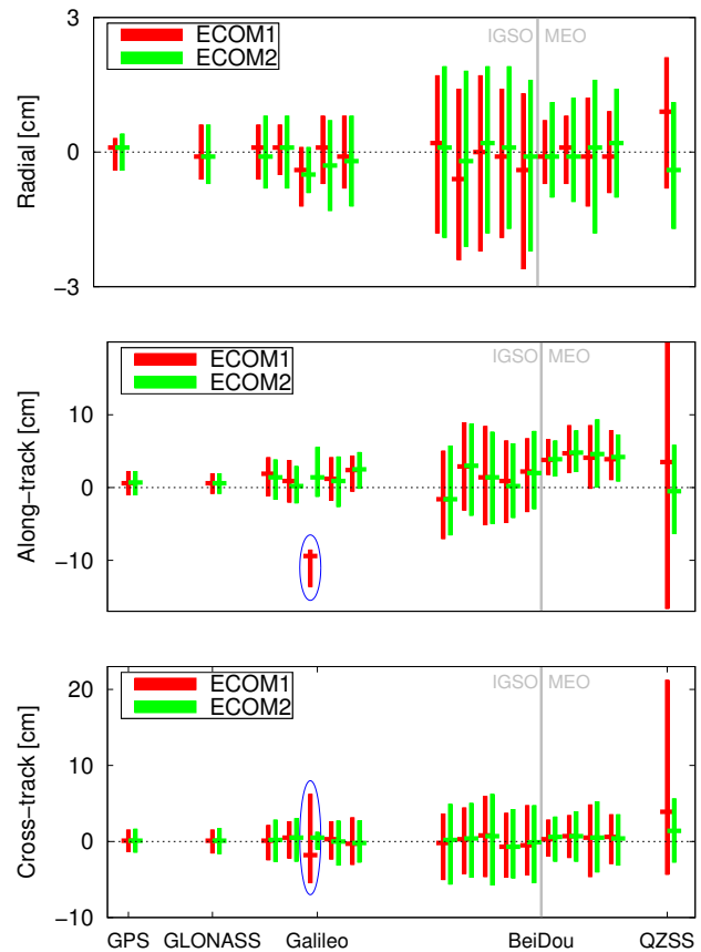
Fig. 3 Median (horizontal bars) and IQR (vertical bars) of the orbit misclosures for COM orbits of 2014 based on the ECOM1 or ECOM2 SRP models, respectively. GPS and GLONASS: system-wise. Other systems: satellite-wise with PRNs increasing from left to right. Note the different scales of the orbit components
