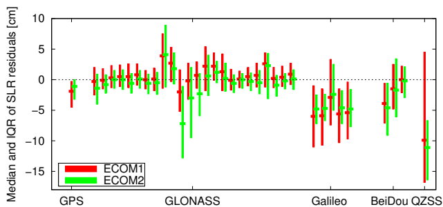
Fig. 4 Median offset (horizontal bars) and IQR (vertical bars) of the SLR residuals of COM orbits of 2014 based on the ECOM1 or ECOM2 SRP models, respectively. Satellite PRNs are increasing from left to right
