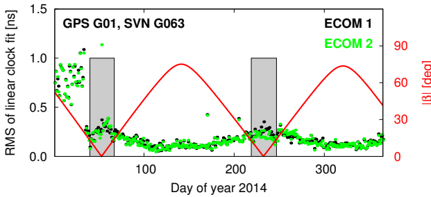
Fig. 11 RMS of linear fit through clock corrections of GPS G01/SVN G063 (Block IIF) based on the ECOM1 or ECOM2 SRP models, respectively. Gray: eclipse seasons. Red: absolute value of \beta
