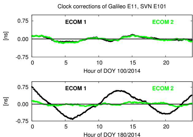
Fig. 14 Satellite clock corrections of Galileo E11 when using the ECOM1 and ECOM2 SRP models, respectively. Top: DOY 100/2014. Bottom: DOY 180/2014
