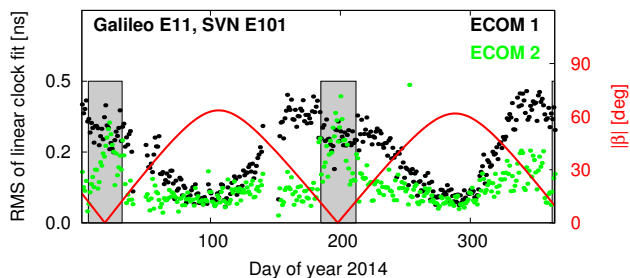
Fig. 13 RMS of linear fit of Galileo E11 clocks when using the ECOM1 and ECOM2 SRP models, respectively. Gray: eclipse seasons. Red: absolute value of \beta
