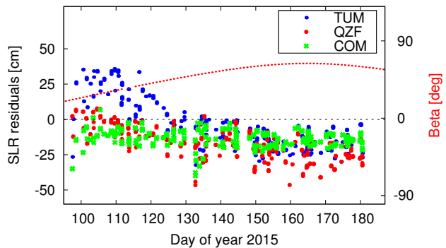
Fig. 17 SLR residuals of QZS-1 orbits from different MGEX ACs during the time interval DOY 95/2015–DOY 180/2015. Red: \beta -angle
