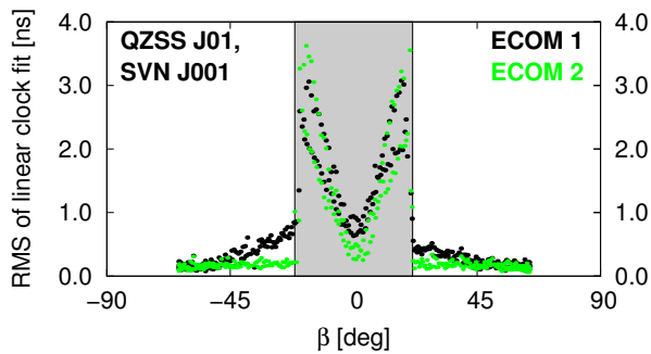
Fig. 16 RMS of linear fit as a function of the \beta -angle for the QZS-1 satellite clocks of 2014 based on the ECOM1 and ECOM2 SRP models, respectively. Gray: orbit normal mode
