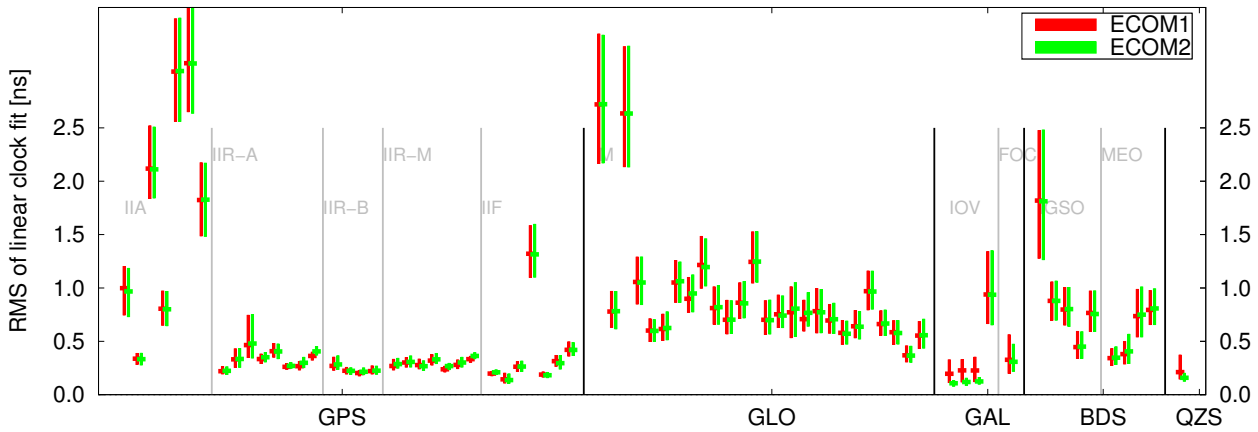
Fig. 10 Median (horizontal bars) and IQR (vertical bars) of the daily RMS of linear clock fit for COM clocks of 2014 when using the ECOM1 or ECOM2 SRP models, respectively. GNSS are separated by vertical black lines. Blocks are separated by vertical gray lines. Satellite SVNs are increasing from left to right within each block
