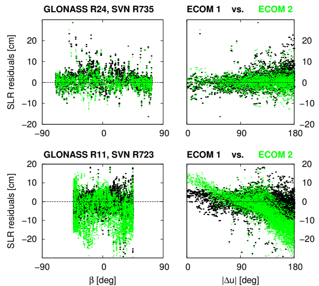
Fig. 5 SLR residuals of GLONASS satellites from 2014 as a function of the \beta -angle (left) and the argument of latitude \Delta u (right). Top: R24 (group 1). Bottom: R11 (group 2)
