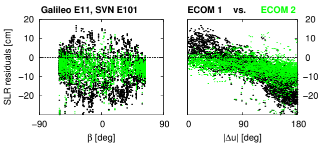
Fig. 7 SLR residuals of Galileo E11 from 2014 as a function of the \beta -angle (left) and the argument of latitude \Delta u (right)
