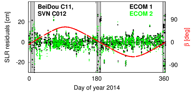
Fig. 8 SLR residuals of BeiDou C11 (MEO) as a function of time. Gray: orbit normal mode. Red: \beta -angle
