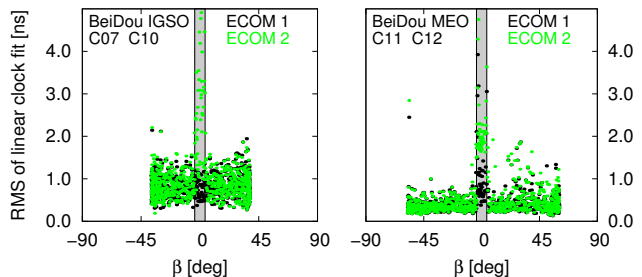
Fig. 15 RMS of linear fit as a function of the \beta -angle for BeiDou satellite clocks from 2014 based on the ECOM1 and ECOM2 SRP models, respectively. Left: IGSOs C07 and C10. Right: MEOs C11 and C12. Gray: orbit normal mode
