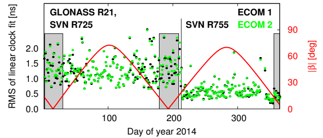
Fig. 12 RMS of linear fit through clock corrections of GLONASS R21 based on the ECOM1 or ECOM2 SRP models, respectively. Gray: eclipse seasons. Red: absolute value of \beta
