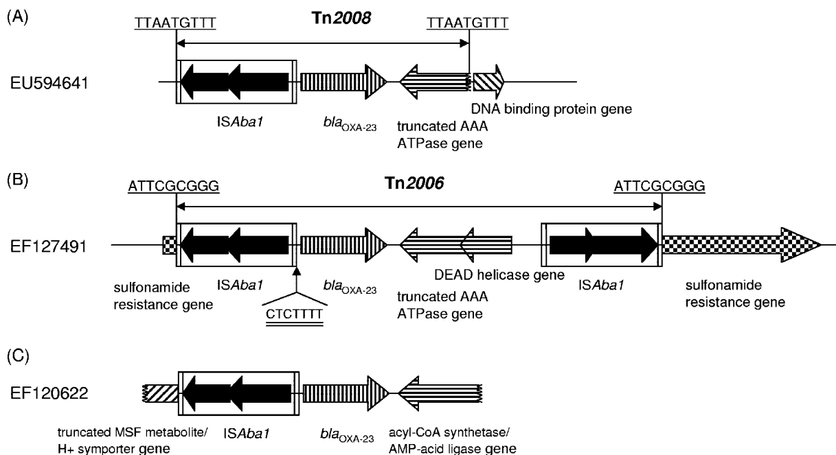
FIG. 2. Schematic representation of the genetic environments of bla OXA-23 from the United States, France, and Turkey. (A) Strain AB017 (investigated in the present study); (B) strain AB13 (7); (C) strain AcKOU1 (GenBank accession no. EF120622). The boundaries of Tn2006 and Tn2008 are indicated, along with the target site duplications (underlined). The 7-bp difference in the site of insertion of ISAbal for strain AB13 is double underlined. Target site duplication was not identified within the available sequence for strain AcKOU1.
