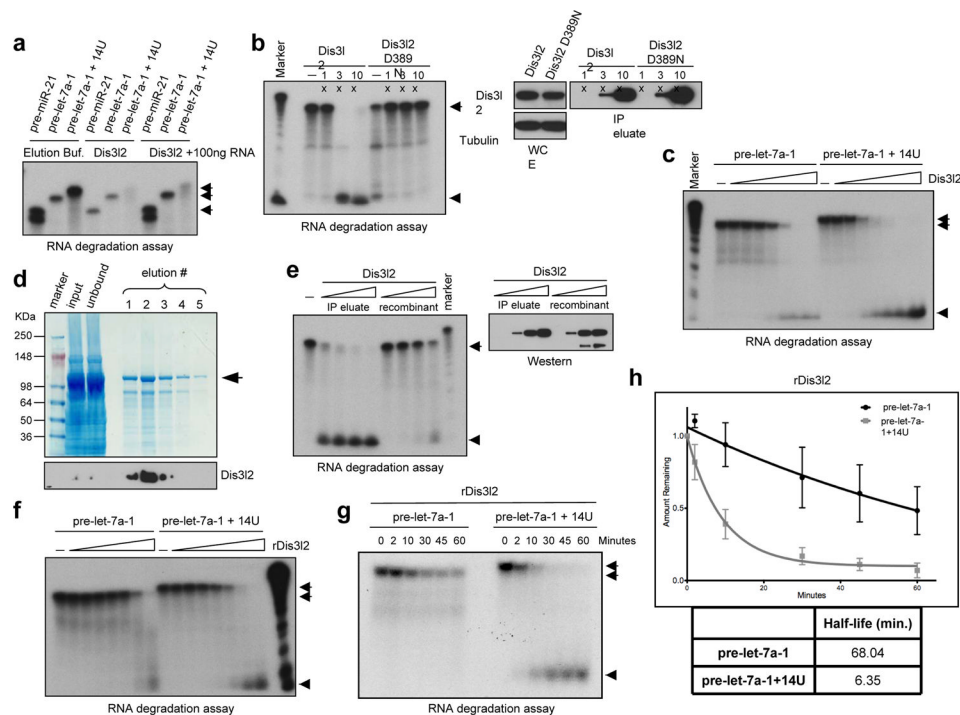
Figure 2. Dis3l2 preferentially degrades uridylated pre-let-7
