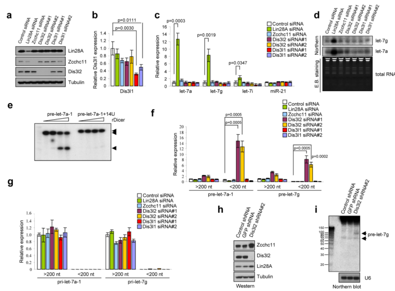
Figure 4. Dis312 is required for degradation of uridylated pre-let-7 in embryonic stem cells (a) Western blot analysis of siRNA knockdown. (b) quantitative RT-PCR (q.RT-PCR) analysis of Dis311 knockdown. Error bars \pm S.D. (n=3). (c) mature miRNA levels measured by q.RT-PCR. Error bars \pm S.D. (n=3) and (d) Northern blot. (e) Dicer processing assay with Arrows indicating pre-miRNA and arrowhead indicating Dicer products. (f)(g) 1 \mu g of total RNA from the samples in (a) was fractionated into >200 nt and <200 nt long RNA and relative levels of pre-let-7 (f) or pri-let-7 (g) RNA were quantitated by real-time PCR. Error bars \pm S.D. (n=3). (h) Western blot analysis of Dis312 cells. (i) Northern blot analysis of pre-let-7g.
