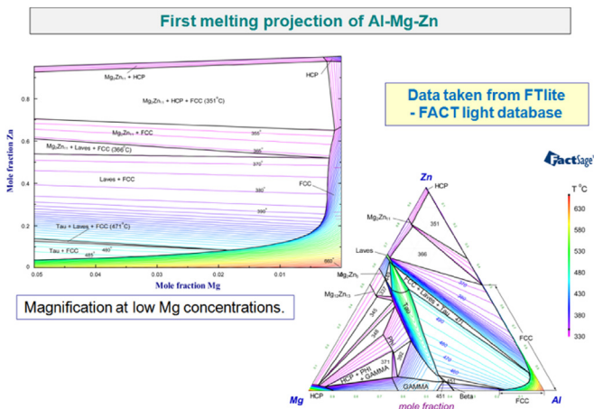
Fig. 27. Phase Diagram –Zn–Mg–Al polythermal first-melting (solidus) projection using data from FTlite.
