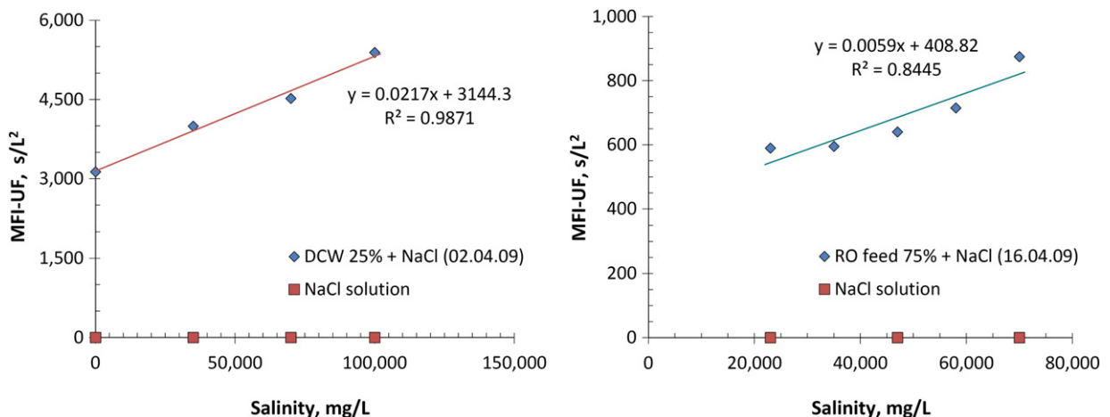
Fig. 14. Salinity effect on particles – MFI-UF of Delft canal water diluted to 25% (left) and SWRO feed (right). PES 10 kDa membranes at flux = 250 L/m 2 /h.
