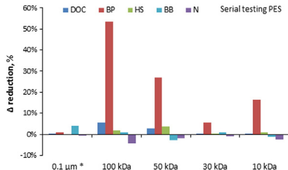
Fig. 16. LC-OCD results – North Sea water batch 1 – serial fractionation.
