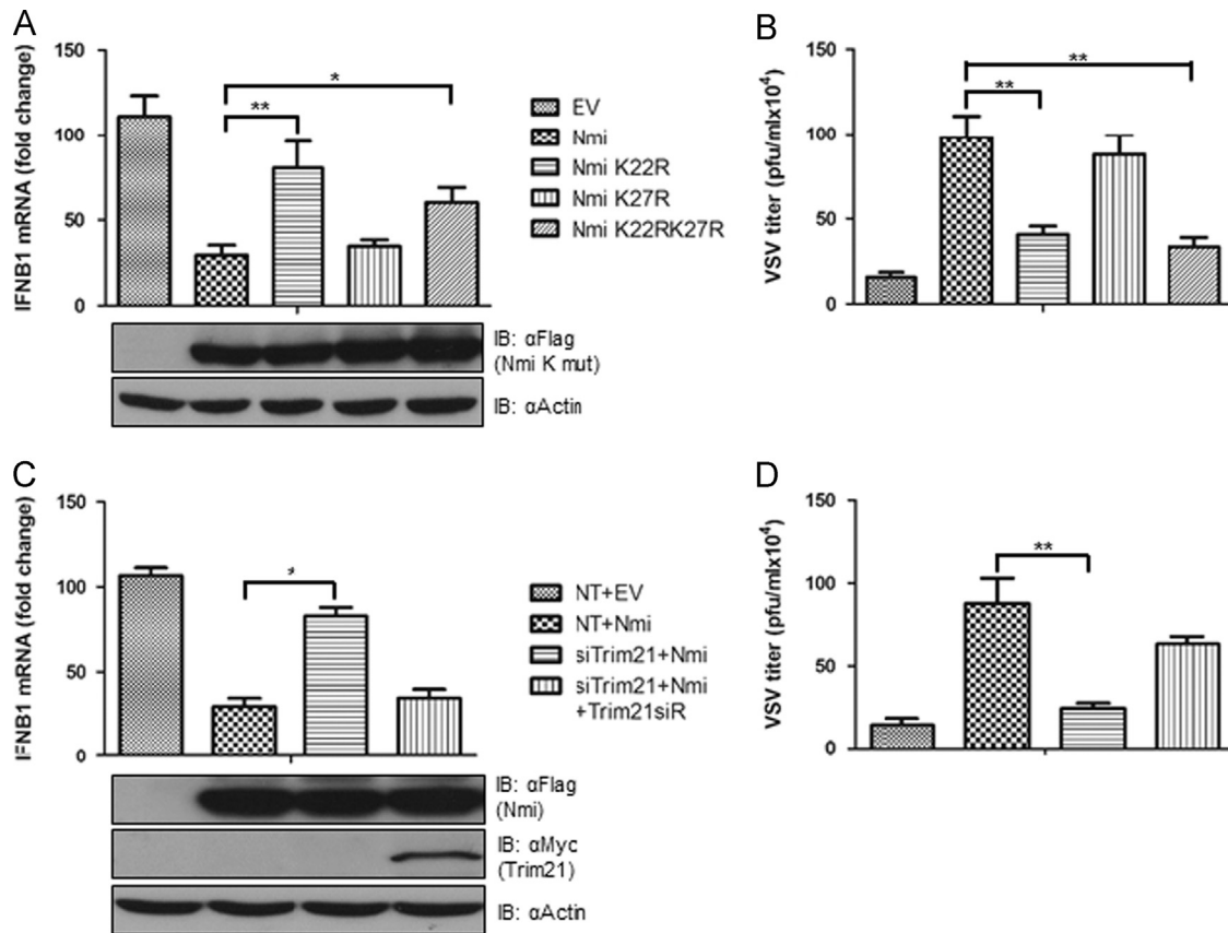
Fig. 6. Trim21 regulates Nmi-mediated inhibition of the innate antiviral response. (A) HEK 293T cells were transfected with an empty vector (EV) control or the indicated Nmi lysine mutants. At 24 hpt, these cells were infected with 80 HA units/ml of SeV for another 16 h. Finally, total RNA was extracted from these cells for qRT-PCR assay. IFNB1 and GAPDH mRNA levels were determined using specific Taqman primer and probes. Values were normalized to the internal control GAPDH and expressed as relative fold changes compared to mock-infected cells transfected with the EV. Expression of the Nmi lysine mutants (Nmi K mut) are shown in the immunoblots. Actin served as the loading control. (B) VSV-IFN bioassay. Supernatants from the experiment described in panel A, were UV-inactivated and added to fresh HEK 293T cells and incubated for 12 h. Then, cells were infected with 0.1 MOI VSV-GFP for another 16 h. Finally, the supernatants were used to determine VSV titers (pfu/ml) by plaque assay on BHK-21 cells. (C) Cells were transfected with 10 nM of NT or siTrim21 for 48 h. Subsequently, NT-transfected cells were re-transfected with an EV or Nmi encoding plasmids, whereas siTrim21-transfected cells were re-transfected with Nmi alone or in combination with Trim21-siR plasmids for another 24 h. Finally, IFNB1 mRNA was quantitated as described in panel A. Expression of Nmi and Trim21 are shown in the immunoblots. Actin served as the loading control. (D) Supernatants from the experiment described in panel C, were UV-inactivated, added to fresh HEK 293T cells and VSV-IFN bioassay was performed as described in panel B. Data presented in the panels are from three independent experiments and the values represent mean and SD for duplicate samples. * P < 0.05 , ** P < 0.01 .
