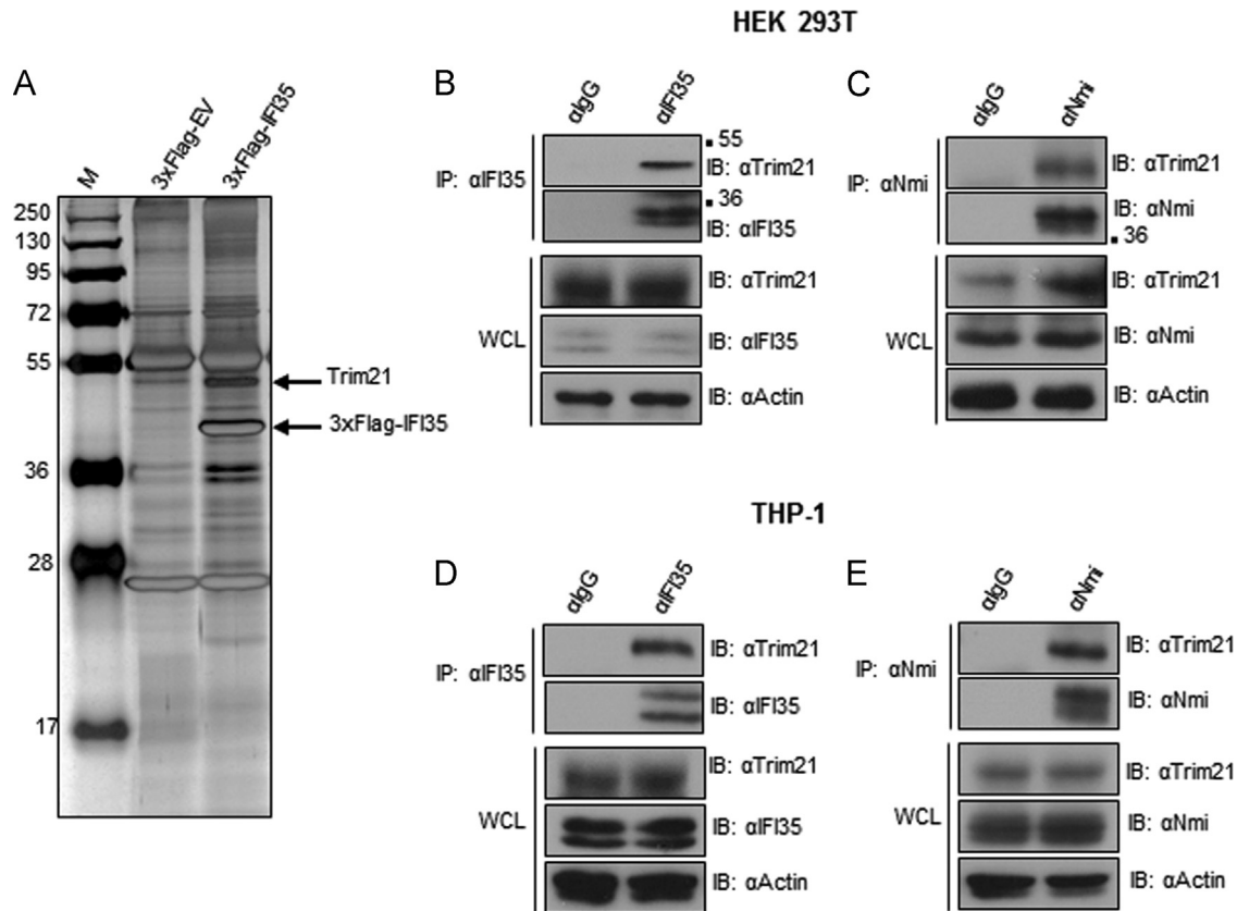
Fig. 1. Trim21 interacts with IFI35 and Nmi. (A) HEK 293T cells were transfected with 5 \mu g of 3xFlag-EV and 3xFlag-IFI35 plasmids. At 24 h post transfection (hpt), cell lysates were subjected to immunoprecipitation with anti-Flag monoclonal antibody (Mab), separated on 10% SDS-PAGE and silver stained. Molecular mass markers (in kDa) are shown in lane M. The bands containing Trim21 and 3xFlag-IFI35, as identified by LC-MS analysis, are indicated with arrows. (B) HEK 293T cell lysates were subjected to immunoprecipitation with anti-IFI35 antibody and immunoblotting with anti-Trim21 antibody. (C) HEK 293T cell lysates were subjected to immunoprecipitation with anti-Nmi antibody and immunoblotting with anti-Trim21 antibody. (D) THP-1 cell lysates were subjected to immunoprecipitation with anti-IFI35 antibody and immunoblotting with anti-Trim21 antibody. (E) THP-1 cell lysates were subjected to immunoprecipitation with anti-Nmi antibody and immunoblotting with anti-Trim21 antibody. Expression of the endogenous proteins in the whole cell lysates (WCLs) were analyzed by immunoblotting with the indicated antibodies. Approximate positions of the molecular weight markers (in kDa) are shown on the right side of the blots.
