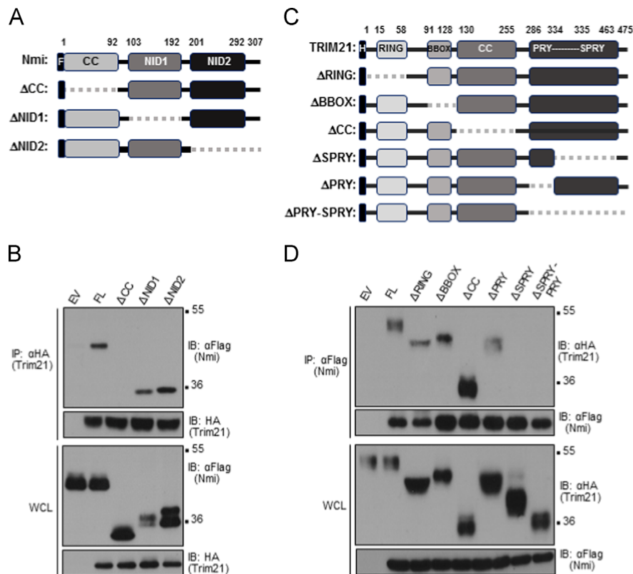
Fig. 3. Trim21 interacts with the coiled-coil domain of Nmi via its SPRY domain. (A) Schematic of the construction of domain deletion mutants of Nmi. F, Flag tag. Approximate amino acid positions of the domains are shown at the top. Various domains are boxed and discontinuous lines represent deletion of those regions. (B) The indicated domain deletion mutants of Nmi along with HA-Trim21 were transfected into HEK 293T cells. At 24 hpt, cell lysates were subjected to immunoprecipitation using anti-HA Mab. Interacting proteins were identified by immunoblotting with anti-Flag Mab. Expression of proteins from transfected plasmids were analyzed in the WCLs using the indicated antibodies. (C) Domain organization and deletion mutants of Trim21. H, HA tag. Approximate amino acid positions of the domains are shown at the top. Various domains are boxed and discontinuous lines represent deletion of those regions. (D) The indicated domain deletion mutants of Trim21 along with 3xFlag-Nmi were transfected into HEK 293T cells. At 24 hpt, cell lysates were subjected to immunoprecipitation using anti-Flag Mab. Interacting proteins were identified by immunoblotting with anti-HA Mab. Expression of proteins from transfected plasmids were analyzed in the WCLs using the indicated antibodies. Approximate positions of the molecular weight markers (in kDa) are shown on the right side of the blots.
