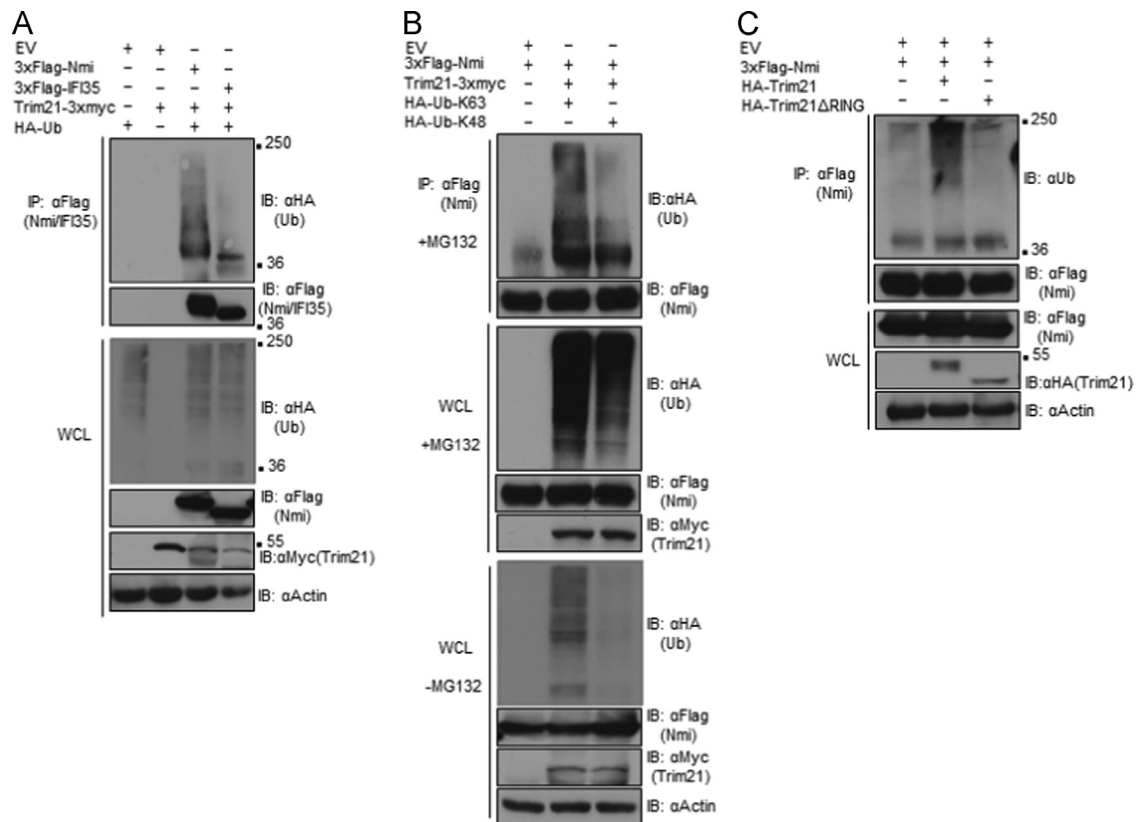
Fig. 2. Trim21 mediates K63-linked ubiquitination of Nmi. (A) HEK 293T cells were transfected with 1 \mu g each of 3xFlag-Nmi or 3xFlag-IFI35 along with 0.5 \mu g each of Trim21-3xMyc and HA-Ub. At 24 hpt, cell lysates were subjected to immunoprecipitation with anti-Flag polyclonal antibody. Ubiquitination of Nmi and IFI35 were detected using anti-HA Mab. Expression of proteins from transfected plasmids were analyzed in the WCLs using the indicated antibodies. (B) Cells were transfected with 1 \mu g of 3xFlag-Nmi along with 0.5 \mu g each of Trim21-3xMyc, HA-Ub-K63 or HA-Ub-K48 plasmids. At 24 hpt, cells were treated with 10 \mu M MG132 or equivalent amount of vehicle (DMSO) for 12 h and cell lysates were subjected to immunoprecipitation with anti-Flag polyclonal antibody. Ubiquitination of Nmi was detected using anti-HA Mab. Expression of proteins from transfected plasmids were analyzed in the MG132 treated and untreated WCLs using the indicated antibodies. (C) Cells were transfected with 1 \mu g of 3xFlag-Nmi along with 0.5 \mu g each of HA-Trim21 or HA-Trim21 \Delta RING plasmids. At 24 hpt, cell lysates were subjected to immunoprecipitation with anti-Flag polyclonal antibody. Ubiquitination of Nmi was detected using anti-Ub antibody. Expression of proteins from transfected plasmids were analyzed in the WCLs using the indicated antibodies. Approximate positions of the molecular weight markers (in kDa) are shown on the right side of the blots.
