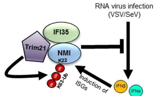
Fig. 7. Proposed model depicting the role of Trim21 in regulation of Nmi-mediated negative regulation of the innate antiviral response. Infection with RNA viruses like VSV or SeV leads to activation of the innate antiviral pathways, resulting in production of IFN- \alpha/\beta , which in turn leads to induction of many ISGs including Trim21, Nmi and IFI35 as shown here. Trim21 interacts with both Nmi and IFI35 but primarily ubiquitinates Nmi on K22 residue via K63-linked ubiquitination. This facilitates interaction between Nmi with IFI35, which then in a negative feedback manner leads to inhibition of IFN- \beta production, resulting in an overall down-regulation of the innate antiviral signaling.
