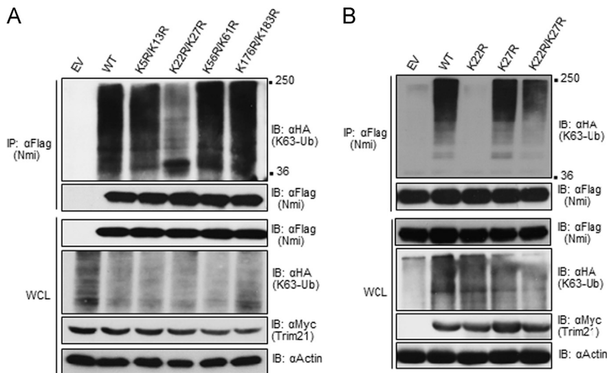
Fig. 4. Trim21 ubiquitinates Nmi on lysine 22 residue. (A) HEK 293T cells were transfected with 1 μg each of a panel of double lysine mutants of Nmi (Flag-tagged) along with 0.5 μg each of Trim21-3xMyc and HA-Ub-K63 plasmids. At 24 hpt, the cell lysates were subjected to immunoprecipitation using anti-Flag Mab. K63-linked ubiquitination of Nmi was detected using anti-HA Mab. Expression of the proteins from transfected plasmids were analyzed in the WCLs using the indicated antibodies. (B) Similar experiment was performed as described in panel A, except the single lysine mutants of Nmi were used. Approximate positions of the molecular weight markers (in kDa) are shown on the right side of the blots.
