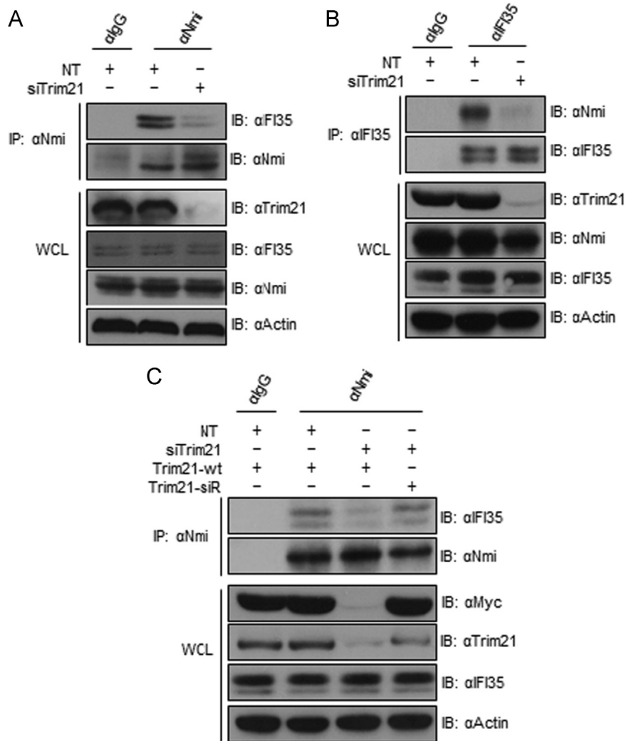
Fig. 5. Trim21 is required for Nmi-IFI35 interaction. (A) HEK 293T cells were transfected with 10 nM of control (NT) or Trim21 siRNA for 72 h. Cell lysates were subjected to immunoprecipitation with isotypic IgG control antibody or anti-Nmi antibody. Presence of endogenous IFI35 in the immunoprecipitates was detected by anti-IFI35 antibody. Endogenous expression of proteins in the WCLs was analyzed by using the indicated antibodies. (B) Similar experiment was performed as in panel A, except the cell lysates were subjected to immunoprecipitation with isotypic IgG control antibody or anti-IFI35 antibody. Presence of endogenous Nmi in the immunoprecipitates was detected by anti-Nmi antibody. (C) Cells were transfected with 10 nM of control (NT) or Trim21 siRNA (siTrim21) for 48 h. Subsequently, cells were re-transfected with 2 μg each of Myc-tagged wild-type Trim21 (Trim21-wt) or siRNA resistant mutant (Trim21-siR) plasmids for another 24 h. Finally, the cell lysates were subjected to immunoprecipitation with anti-Nmi antibody. Presence of endogenous IFI35 in the immunoprecipitates was detected by anti-IFI35 antibody. Expression of endogenous and exogenously expressed proteins in the WCLs was analyzed by using the indicated antibodies.
