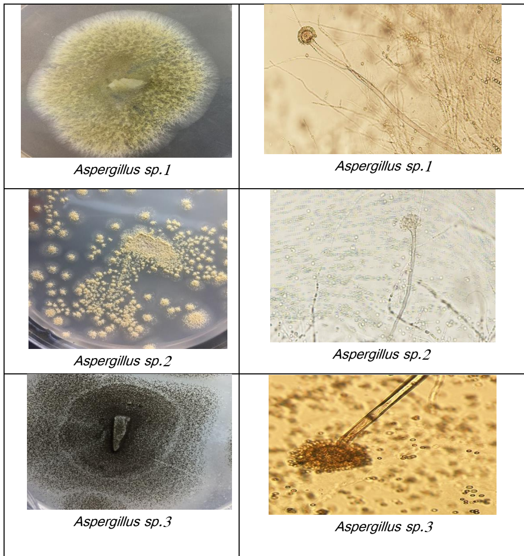
Figure 1. Images of fungal isolates for each genus isolated from different kinds of oil seeds, (A) Under microscope (40X) and (B) on a petri dish.
