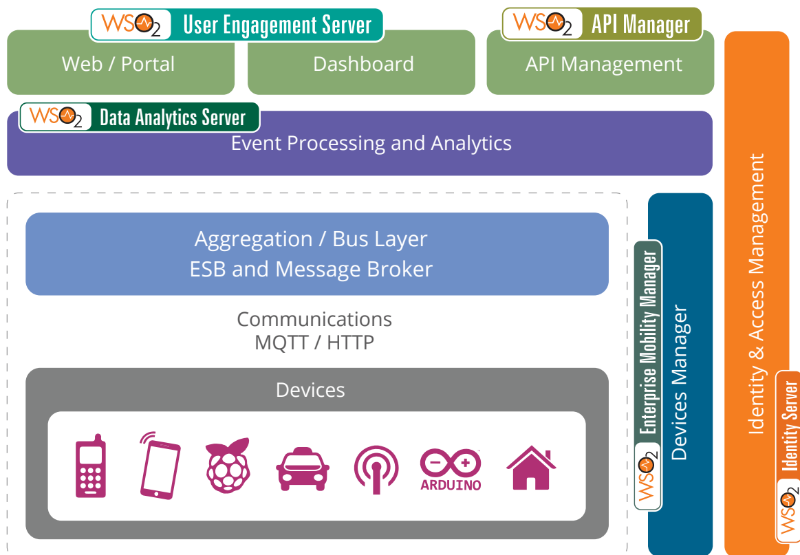
Figure 3: IoT reference architecture mapped to WSO2 platform components
