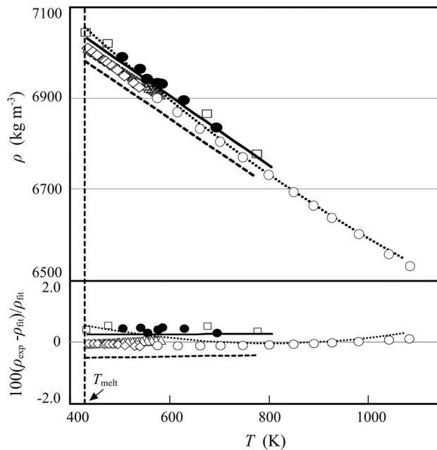
Fig. 4. Primary density data and their percentage deviations from Eq. (1) for liquid indium as a function of temperature. Alchagirov et al. 8 (Δ), Wang et al. 32 (⋯), Schneider and Heymer 10 (●), McClelland and Sze 33 (□), Stankus and Tyagel'sky 24 (○), Karamurзов 7 (—), Berthou and Tougas 53 (—), Crawley 9 (◇).
