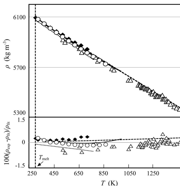
Fig. 3. Primary density data and their percentage deviations from Eq. (1) for liquid gallium as a function of temperature. Yagodin et al. 23 (Δ), Stankus and Tyagel'sky 24 (—), Alchagirov 25 (⋯), Na'giev and Ibragimov 26 (◆), Nizhenko et al. 28 (—), Köster et al. 27 (○).
