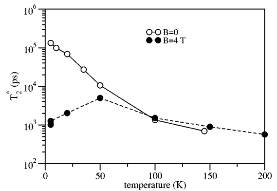
FIG. 19. Measured temperature dependence of the spin dephasing time for bulk n -GaAs doped with N_d = 1 \times 10^{16} \text{ cm}^{-3} Si donors, at B = 0 and B = 4 T. The sample is insulating at low T and nondegenerate at high T ( T \geq 50 K, assuming \approx 4 MeV for the donor binding energy), where donors are ionized. Adapted from Kikkawa and Awschalom, 1998.
