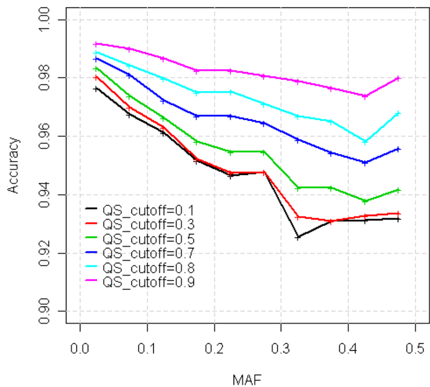
Impact of SNP MAF on Imputation Accuracy, Ilmn317K
