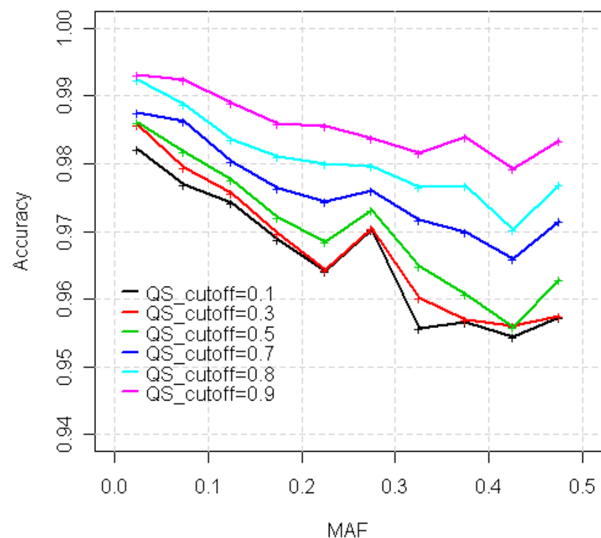
Impact of SNP MAF on Imputation Accuracy, Ilmn650Y
