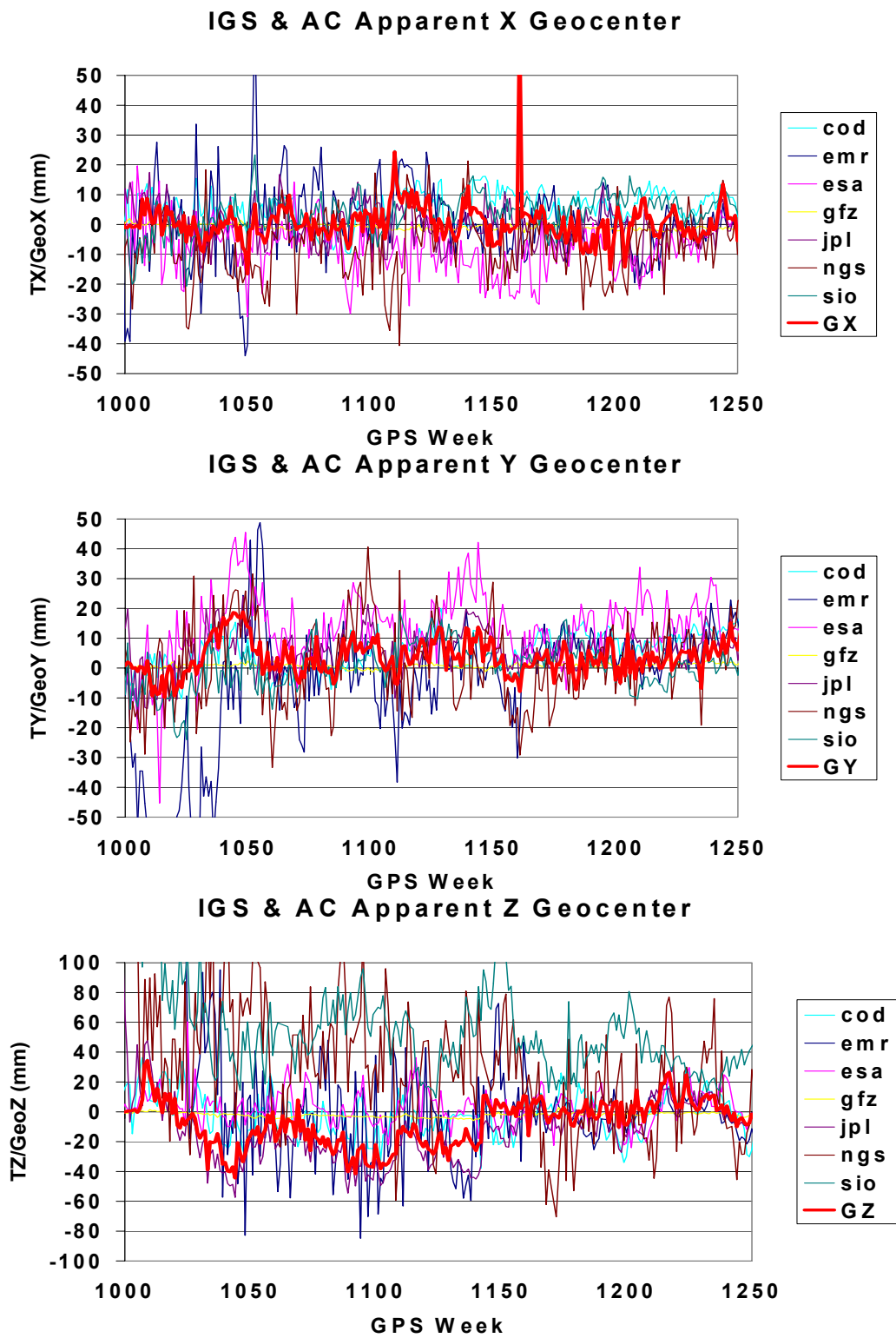
Figure 1: Weekly estimated transformation parameters using AC solutions and IGS "apparent geocenter".
