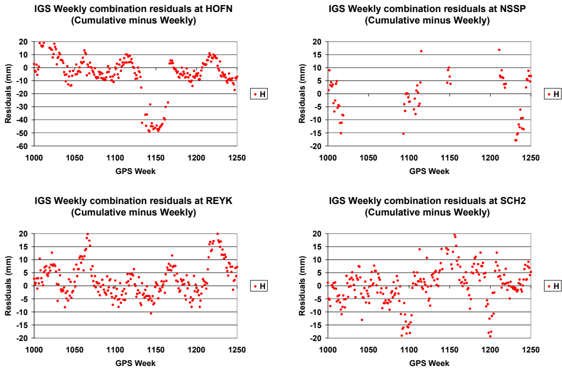
Figure 6: Station height residuals at four stations (HOFN, NSSP, REYK and SCH2).
