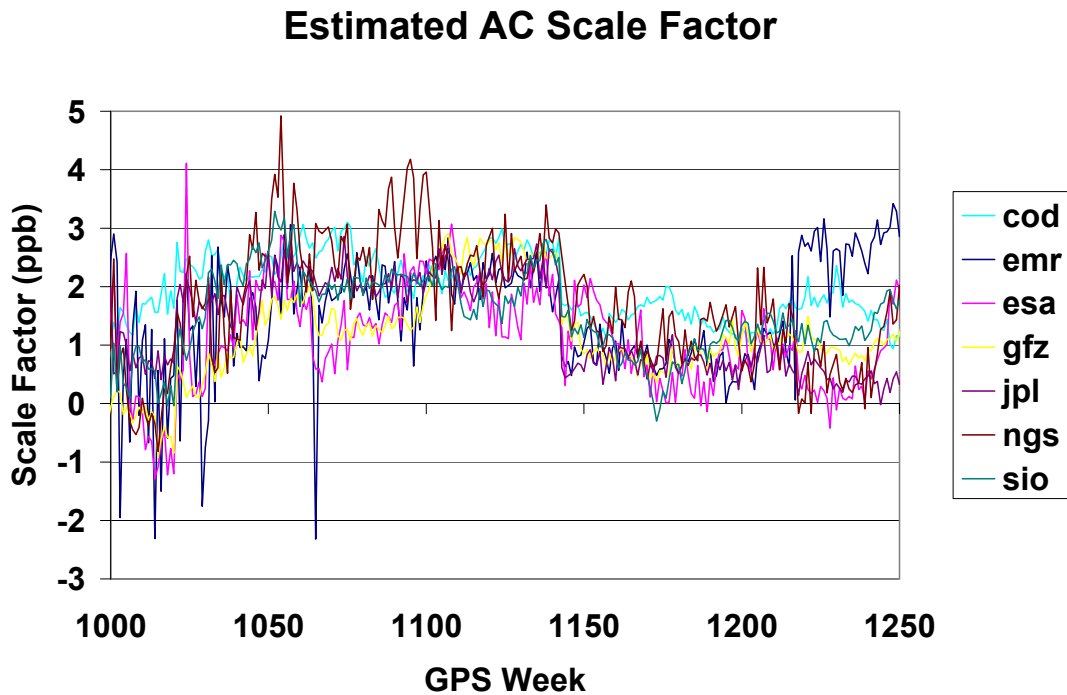
Figure 2: Weekly estimated AC scale
