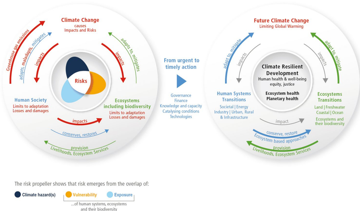
Figure 1. The concept of climate resilient development, based on interactions between climate, ecosystems, and human society. Source: IPCC AR6 WGII
