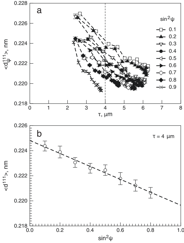
Fig. 3. a) As measured lattice spacing-depth, \langle d_{\psi}^{111} \rangle vs \tau profiles of expanded austenite measured with the scattering vector method applied to a nitrided 316 L stainless steel. b) A reconstructed \sin^2 \psi plot at chosen information depth, \tau , of 4 \mu\text{m} is also given.
