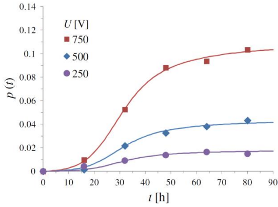
Fig. 13: Power degradation as function of the time with the system voltage as parameter. Reprinted from Hattendorf 2012 [133].
