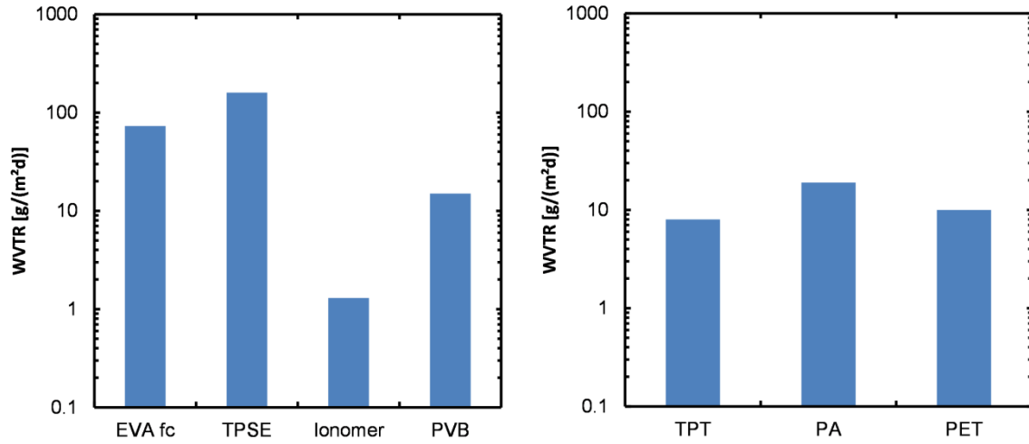
Fig. 2: Water vapour transmission rate (WVTR) through encapsulants, ethylene vinyl acetate (EVA), thermoplastic silicone elastomer (TPSE), an ionomer, and polyvinyl butyral (PVB), and through backsheets Tedlar-polyester-Tedlar (TPT) foil, a polyamide (PA) sheet, and a polyethylene terephthalate (PET) composite films. Adapted from [16].
