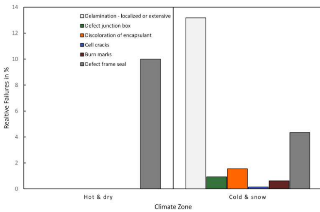
Fig. 60: Distribution of silicon PV module failures in the field classified in different climate zones according to Köppen-Geiger climate classification system [209].
