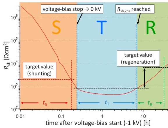
Fig. 17: Evolution of the shunt resistance with sequenced applied voltage. Reprinted from Taubitz 2014 [135].
