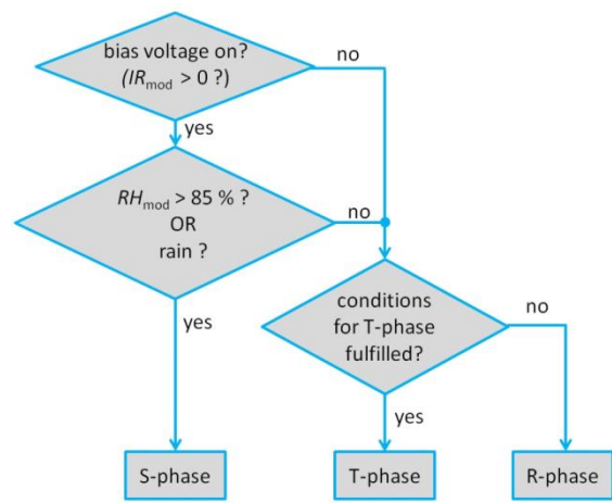
Fig. 18: Phase assignment process. Reprinted from Taubitz 2014 [135].
