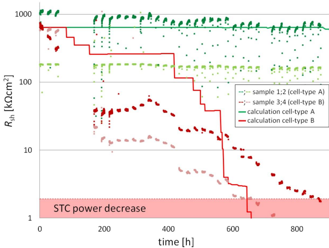
Fig. 19: Measured and modeled R_{sh} evolution. Reprinted from Hacke 2016 [137].
