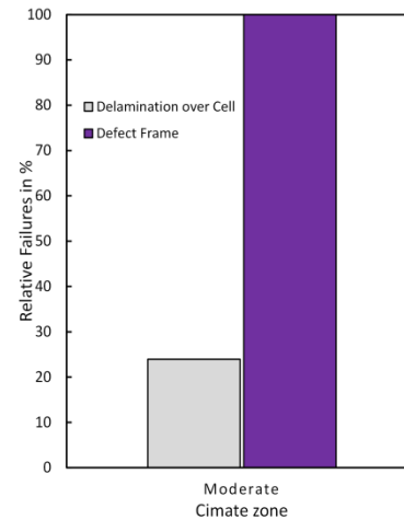
Fig. 62: Distribution of amorphous silicon module failures in the field classified in different climate zones according to Köppen-Geiger climate classification system [209]. The amorphous silicon modules were installed more than 30 years prior to inspection.
