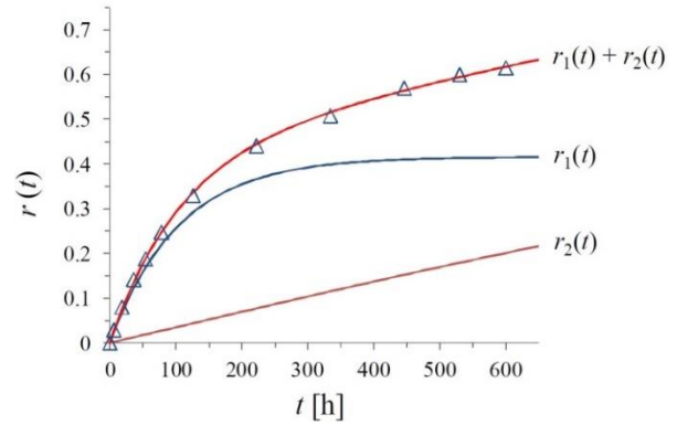
Fig. 16: The regeneration function r(t) and its two components. The graphic relates to the identically marked curve in Fig. 15 ( p_0 = 0.43 ). Reprinted from Hattendorf 2013 [134].
