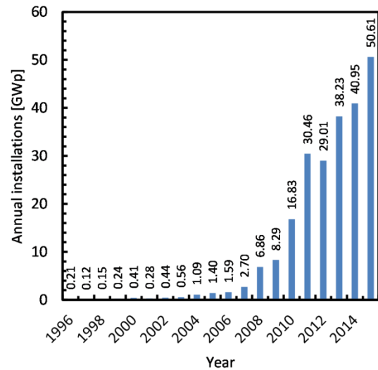
Fig. 55: Evolution of global annual PV system nameplate installations, composed from numbers in [206].
