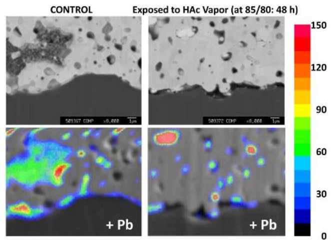
Fig. 30: Upper images: SEM images of cross sectional view a front silver paste/silicon interface. Lower images: Overlay of secondary electron microscope (SEM) and electron probe micro analysis (EPMA) images of the same sections. In the left side images of a control sample, on the right samples exposed to HAc vapour for 48h at 85°C are shown. The colour levels (ppm) indicate the concentration of Pb observed with EPMA.
