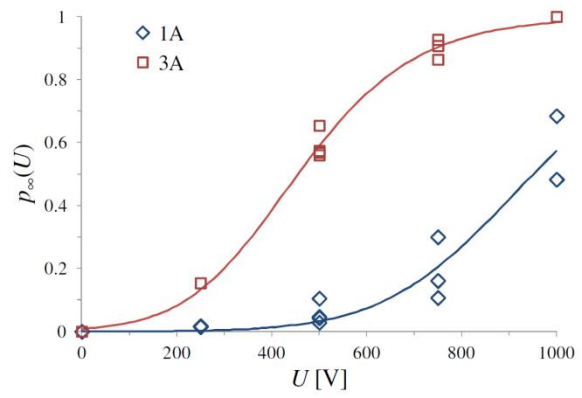
Fig. 14: Final power value as a function of the applied voltage with the module type as parameter. Reprinted from Hattendorf 2012 [133].
