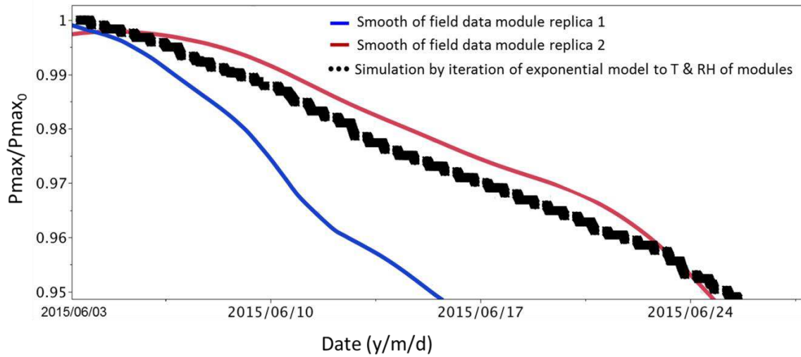
Fig. 20: Iteration of the chamber test-derived exponential model to 20-s interval data for CdTe module temperature T and surface humidity H in Florida and its correspondence to the measured module power P_{max} for two fielded replicas.
