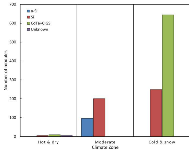
Fig. 59: Absolute number PV module technologies classified to Köppen-Geiger climate classification system [209].
