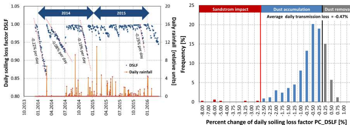
Fig. 33: Time evolution of Daily Soiling Loss Factor (DSLIF) at a location in Arizona desert.
