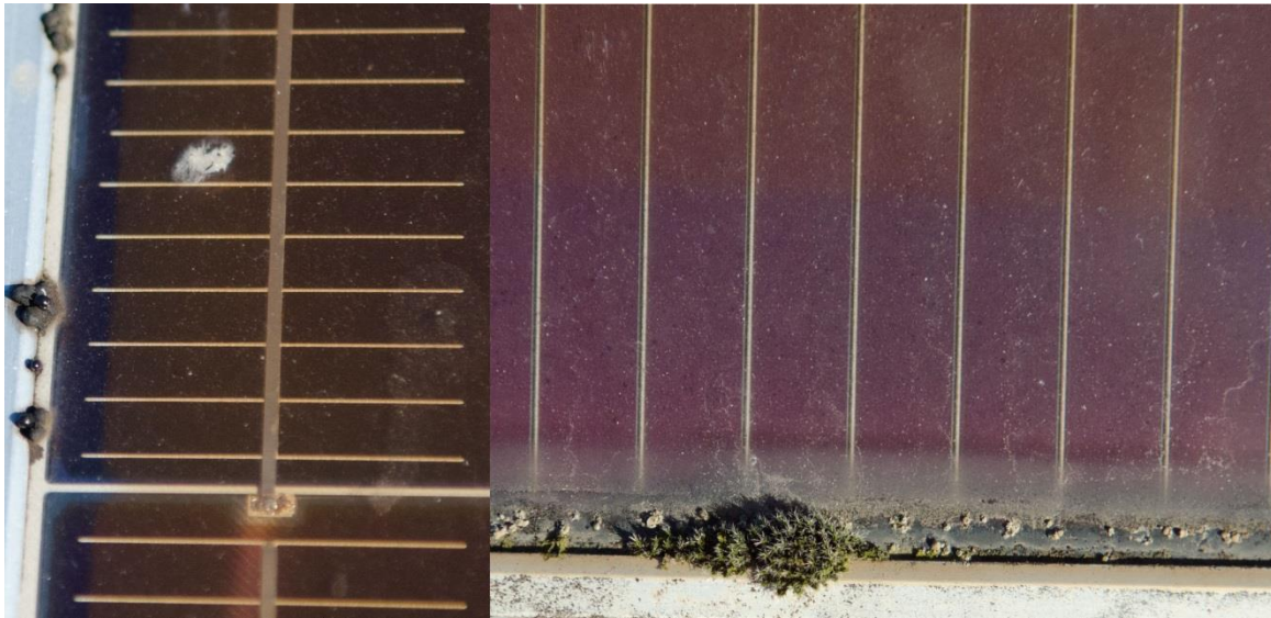
Fig. 38: Example of bird droppings (left) and moss (right) on a PV module.
