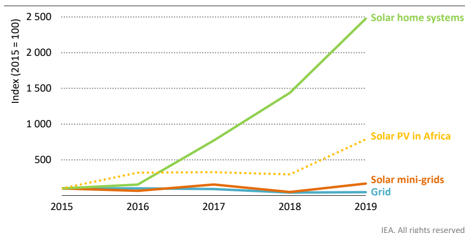
Figure 3.3 ▶ Increase in new connections in Ghana, Kenya and Nigeria by type versus solar PV overall in Africa
