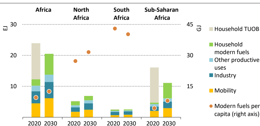
Figure 2.6 ▶ Total final energy consumption by sector and modern fuel use per capita by region in the SAS
