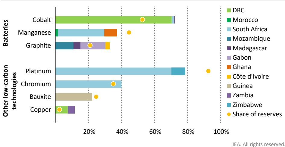
Figure 3.24 ▶ Share of Africa in global production of selected minerals, 2020
