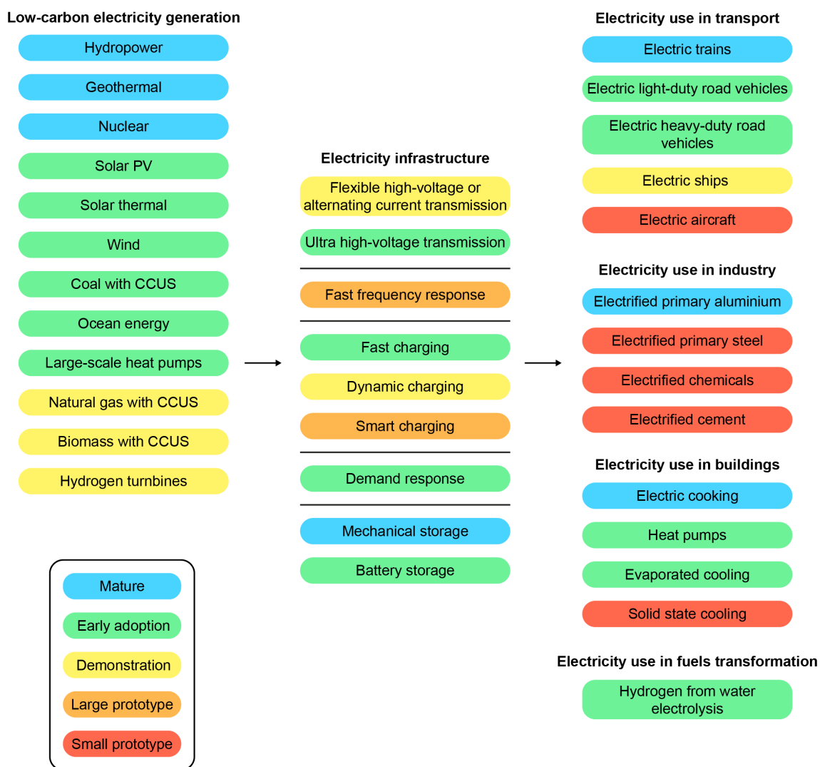
Figure 2.11 Technology readiness level of technologies along the low-carbon electricity value chain
