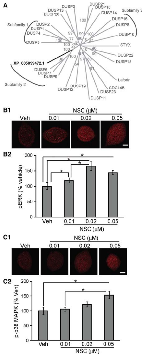
Figure 1. A low NSC concentration specifically activates ERK but not p38 MAPK. (A) Cladogram depicting the relative distance of the predicted protein sequence of Aplysia DUSP (NCBI: XP_005099472.1) from those of human DUSPs, constructed with QuickTree (Howe et al. 2002). The predicted protein shows greater similarity with proteins in subfamily 2. Bootstrap values are percentages based on 1000 replicates. (B1) and (C1) Representative confocal images of pERK and p-p38 MAPK immunofluorescence in SNs treated for 2 h with NSC at different concentrations. Scale bar, 20 μm. (B2 and C2) Summary data. In this and subsequent illustrations, error bars represent SEM and significant differences are indicated by * for P < 0.05 .
