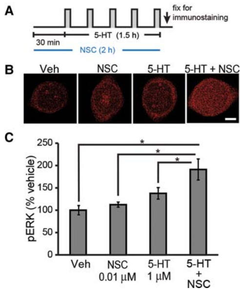
Figure 2. NSC and 5-HT activated ERK in cultured SNs. (A) Protocol for NSC application. (B) Representative confocal images of pERK immunofluorescence in SNs treated with 1 \mu M 5-HT or Veh in the presence or absence of 0.01 \mu M NSC. Scale bar, 20 \mu m. (C) Summary data. 5-HT + NSC gave a substantially greater increase in pERK than did NSC or 5-HT alone.
