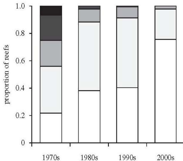
Figure 11. Proportion of reefs in five rugosity index categories across the Caribbean between 1969 and 2008. Number of studies for each decade: 1970s: n = 32; 1980s: n = 52; 1990s: n = 136 and 2000s: n = 167. Rugosity categories: Black, >3; dark grey, 2.5–3; mid grey, 2–2.5; pale grey, 1.5–2; white, 1–1.5.
