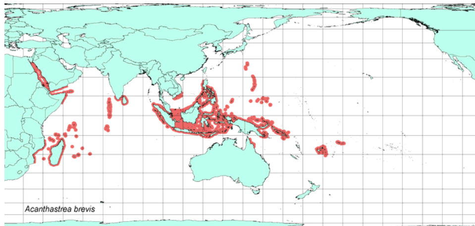
Figure 73. Range map for Acanthastrea brevis .
