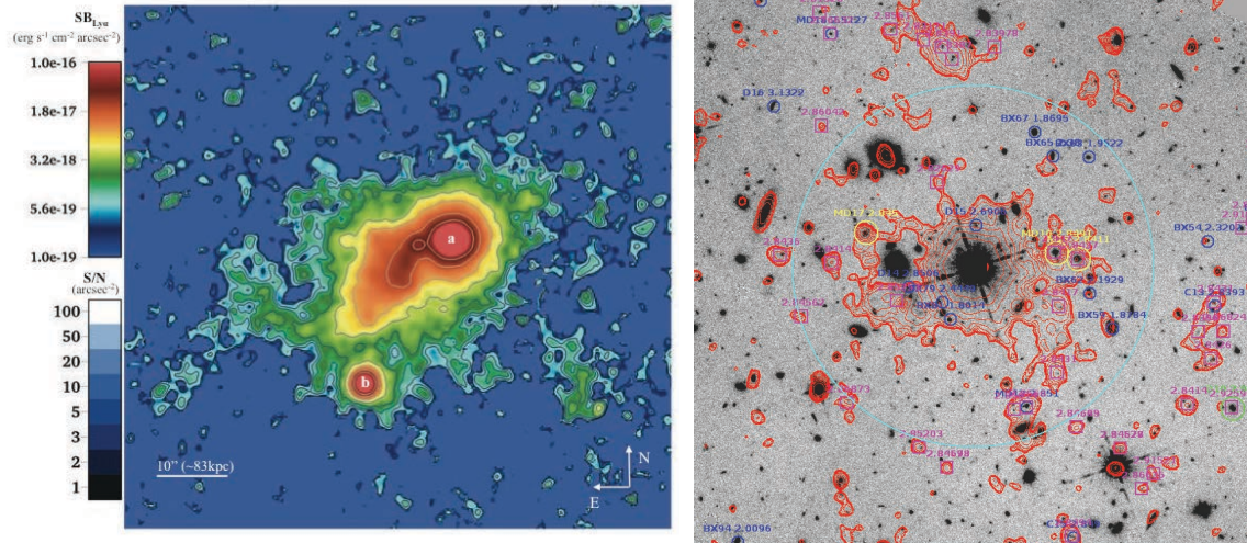
Figure 5.21: (Left) \text{Ly}\alpha image of the Slug Nebula surrounding UM287 (labeled “a”), obtained using narrow-band imaging with Keck/LRIS-B. The color map indicates the \text{Ly}\alpha surface brightness per \text{arcsec}^2 . The extended emission spans a projected angular size of \approx 55 \text{ arcsec} (about 460 physical kpc), measured from \sim 10^{-18} \text{ erg s}^{-1} \text{ cm}^{-2} \text{ arcsec}^{-2} contours. The nebula appears broadly filamentary and asymmetric, extending mostly on the eastern side of quasar “a” and towards south-east in the direction of a second, fainter quasar (labeled “b”). [Adapted from Cantalupo et al. 2014]. (Right) A 2' \times 2' region (the cyan circle has a diameter of 1' , or \sim 500 \text{ pkpc} ) surrounding the z=2.84 QSO HS1549+19; the grayscale is a deep HST WFC3 F160W image ( 1.6 \mu\text{m} ) centered on the QSO; red contours are \text{Ly}\alpha emitting regions at the same redshift, where magenta labels mark regions with \text{Ly}\alpha spectra. (Adapted from Trainor et al 2013).
