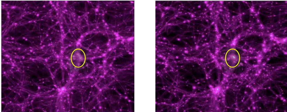
Figure 3.7: Snapshots at z=0 for N -body simulations of GR (left) and f(R) gravity (right). 256^3 particles are simulated in a B=64 Mpc/h box. The Hu-Sawicki model (Hu & Sawicki 2007) is adopted for the f(R) simulation [Zhao, Li & Koyama 2011a].
