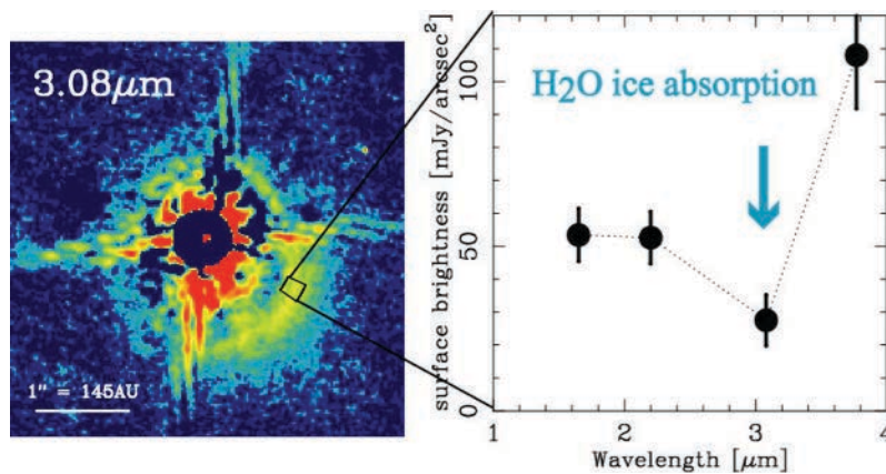
Figure 8.5: Scattered light image of the disk around the Herbig Fe star HD 142527 at 3.08 \mu\text{m} (left) and the scattered light spectra (right). The \sim 3.1 \mu\text{m} absorption feature, probably due to the scattering by water ice grains, is clearly seen in the spectra. As we go closer to the central star inside of the snow line, this absorption band will disappear due to the absence of water ice, which will directly show the snow line location at the disk surface.
