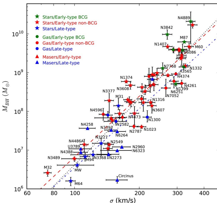
Figure 5.13: Recently compilation of M_{BH}-\sigma_* measurements from McConnell and Ma (2013). The black hole masses are measured using the dynamics of masers (triangles), stars (stars), or gas (circles). Error bars indicate 68% confidence intervals. The black dotted line shows the best-fitting power law for the entire sample.
