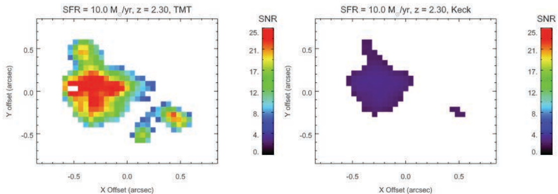
Figure 5.8: A simulated z=2.3 galaxy, with H\alpha redshifted into the K-band window and an integrated star formation rate of 10 M_{\odot} \text{ yr}^{-1} (left). This is compared to Keck observations of the same simulated galaxy (right). Complex structure with multiple knots can be seen with IRIS and TMT, while only the brightest portion of the galaxy is barely detectable ( \text{SNR} \sim 3 ) with Keck.
