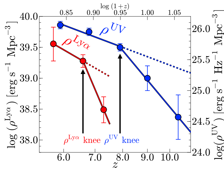
Figure 4.1: Evolution of Ly \alpha and UV luminosity densities based on recent observations (Konno et al. 2014). The red and blue circles represent the Ly \alpha and UV luminosity densities, respectively (labeled on the left and right vertical axes, respectively). Toward high- z , the decrease of Ly \alpha luminosity density is clearly more rapid than that of UV at z \sim 7 , indicative of strong scattering given by neutral hydrogen gas in the IGM.
