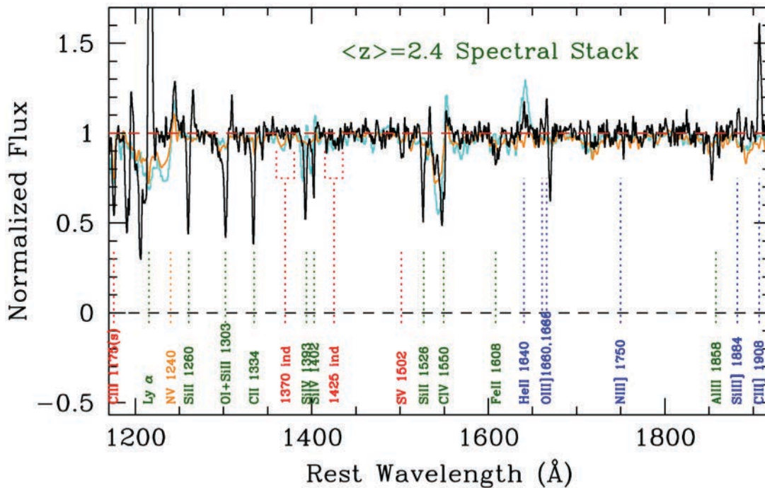
Figure 5.4: Rest-UV composite spectrum of star-forming galaxies at \langle z \rangle \sim 2.4 , obtained with R \sim 1500 . The labeled features are color-coded according to their origin: red=stellar photospheric (O-stars); blue=nebular; green=primarily interstellar; orange: hot star wind lines. The CIV feature includes both a stellar P-Cygni emission/absorption as well as interstellar; HeII includes both nebular (narrow) and stellar (broad) components. Superposed on the observed spectra are population synthesis models, both assuming Salpeter IMF and 0.2 solar metal abundance: cyan: BPASS (Eldridge & Stanway 2009); light orange: Rix et al (2004).
