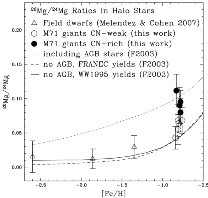
Figure 7.14: 26 Mg/ 24 Mg ratios in both field dwarfs (triangles; Melendez & Cohen 2007) and M71 giants (circles) as a function of [Fe/H]. Chemical evolution models by Fenner et al. (2003) including (dotted line) and excluding (solid and dashed lines) AGB stars are shown. At the metallicity of M71 ([Fe/H] = -0.8 dex) the isotopic ratios in the CN-weak stars (open circles) are explained by massive stars, but the CN-strong stars (filled circles) may have been polluted by intermediate-mass AGB stars. (Source: Melendez & Cohen 2009).
