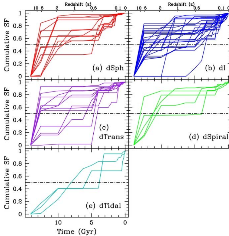
Figure 7.19: Cumulative star formation histories of 60 dwarf galaxies, split by morphological types, as derived by Weisz et al (2011). Statistical comparison of the star formation histories for each type reveals the similarities and key differences, and the epochs at which they occur.
