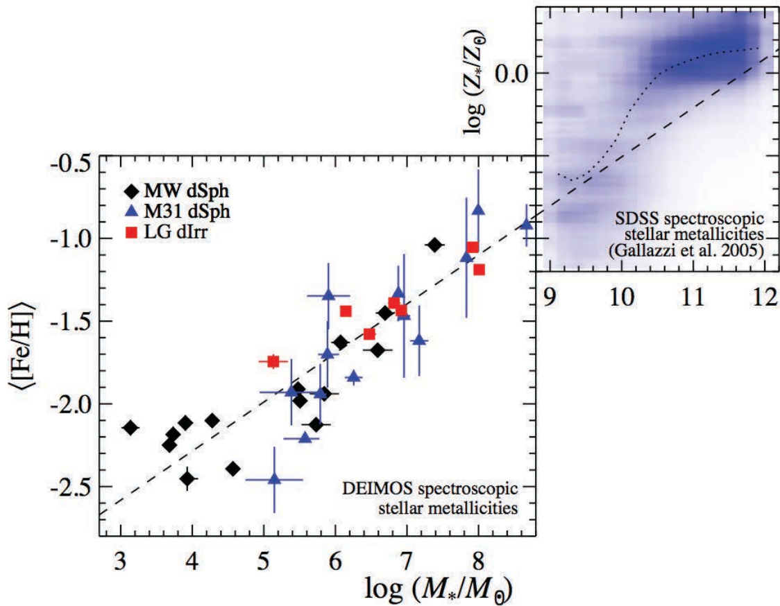
Figure 7.7: Stellar mass-stellar metallicity relation for Local Group dwarf galaxies (left) and more massive SDSS galaxies. The local group metallicities ( \langle [Fe/H] \rangle ) were measured from iron lines, and the SDSS metallicities ( \log Z_* ) were measured from a combination of absorption lines, mostly Mg and Fe. The conversion between \langle [Fe/H] \rangle and \log Z_* depends on [Mg/Fe] . The local group data is same as that in Figure 7.6, but it is plotted here vs. stellar mass rather than luminosity. The dashed line is the least-squares fit to the Local group galaxies, and the dotted line in the right panel is the moving median for the SDSS galaxies. Although the techniques at measuring both mass and metallicity differ between the two studies, the mass-metallicity relation is roughly continuous over nine orders of magnitude in stellar mass. (Kirby et al., 2013a)
