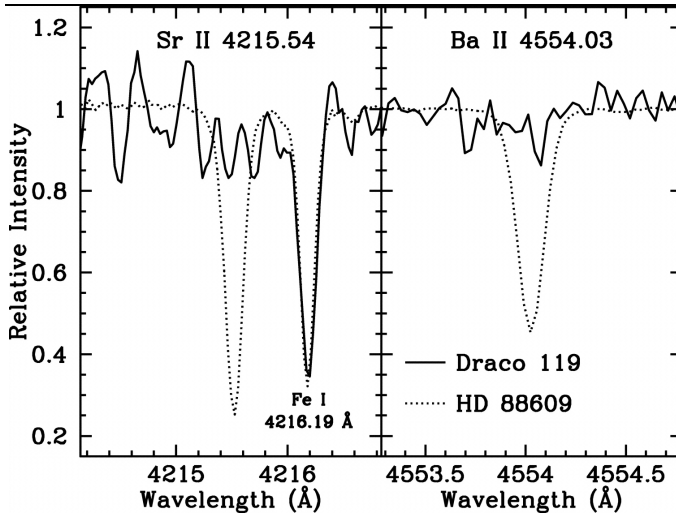
Figure 7.17: Neutron-capture elements are deficient in a red giant (D119) in the Draco Dwarf Spheroidal galaxy ( Fe/H = -2.95 ); comparison with HD 88609, which has similar metallicity (Fulbright, Rich, & Castro 2004). The Hercules dwarf spheroidal galaxy shows similar striking deficiencies (Koch et al. 2013). The proposed WFOS instrument on TMT would be capable of making measurements on giants similar to these even as distant as the Andromeda galaxy. Recently, a metal-poor giant has been found in a binary system in Hercules (Koch et al. 2014).
