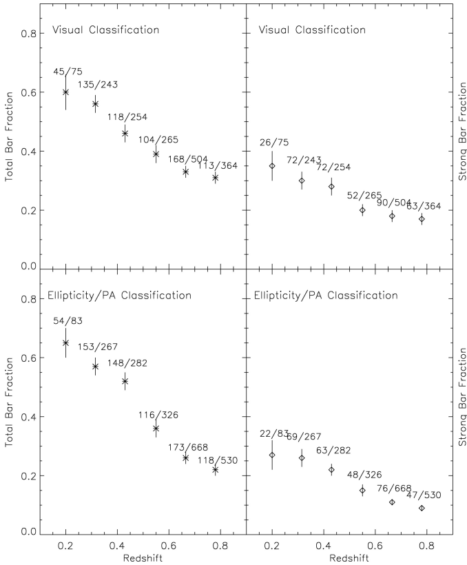
Figure 5.11: Bar fraction as a function of redshift in equal time bins of 1 Gyr to a look back time of 7 Gyr. The bar fraction drops from 65% in the local Universe to ~ 20% at z \sim 0.84 . The left panels show the bar fraction for all galaxies classified as barred, whereas the right panels show the same for only the strong bars. The two rows show two independent methods for the bar classification. Numbers above each data point indicate the total number of bars (or strong bars) / total number of galaxies in the bin and the error bars reflect the error in the measurement of the bar fraction. From Sheth et al. (2008).
