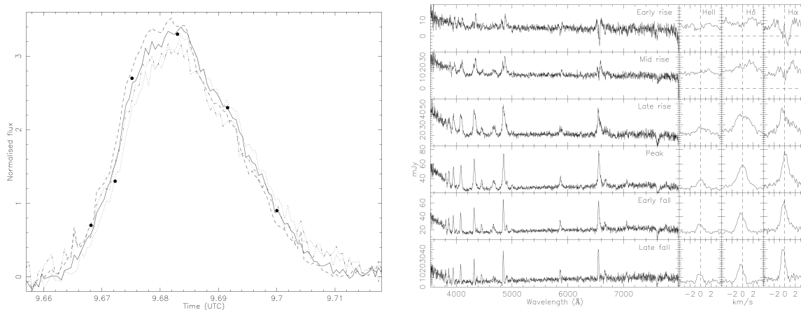
Figure 9.9: Left: Continuum light-curves of a small flare seen in the Dwarf Nova SS Cyg. Observations were made with Keck/LRIS. Light curves are 3615Å (dot-dashed), 4225Å (dashed), 5500Å (solid) and 7320Å (dotted). Right: Spectra at times (dots in left panel) throughout the flare. (Skidmore et al. 2004).
