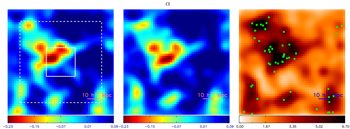
Figure 5.19: Simulation slices illustrating Ly \alpha forest tomography with map resolutions of 3.5 h^{-1} Mpc. (Left) A tomographic reconstruction from a set of simulated Ly \alpha forest absorption sightlines from sources down to a survey depth of m_{AB} = 24.5 , which include realistic modeling of spectral S/N assuming the Reddy et al. (2008) LBG UV luminosity function. The central panel shows the true underlying 3D Ly \alpha forest absorption field while the right panel shows the underlying dark-matter overdensity, \Delta = \rho/\langle\rho\rangle (both smoothed with a 3.5 h^{-1} Mpc Gaussian to match the reconstructed map). These slices have dimensions (100 h^{-1} \text{ Mpc}) \times 2 \times 2 h^{-1} \text{ Mpc} , and the line-of-sight direction is into the plane of the page — in real surveys, one covers \square 400 h^{-1} \text{ Mpc} along the line-of-sight. The green dots overlaid on the DM field show positions of R \leq 25.5 galaxies coeval with the Ly \alpha forest, obtained from halo abundance matching. The solid small rectangle overlaid on the left-panel shows the footprint covered by approximately 10 WFOS pointings, while the large dashed rectangle shows the area equivalent to 1 \text{ deg}^2 on the sky. [Image adapted from Lee et al. 2014]
