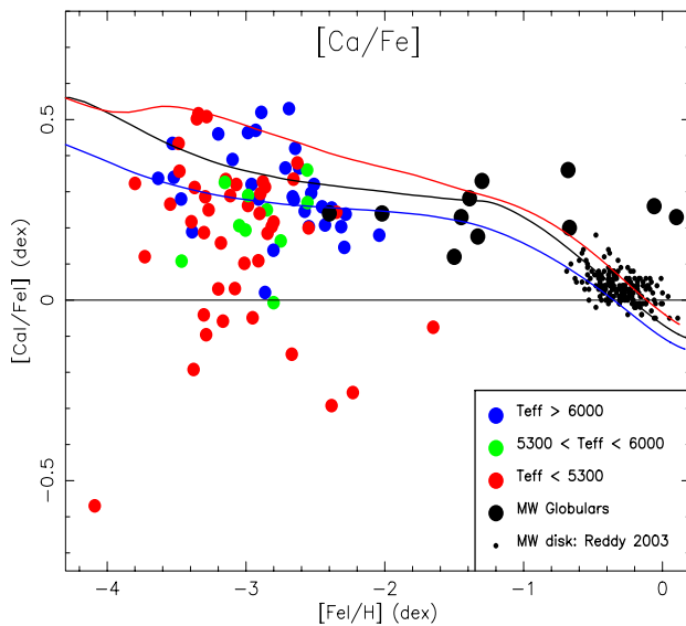
Figure 7.15: The element ratio [Ca/Fe] as a function of [Fe/H] for a large sample of C-normal extremely-metal-poor halo stars (Cohen et al. 2013); colors of the filled points indicates the T_{eff} of the star. The disk stars from Reddy et al. (2003) are indicated as small black dots concentrated near solar metallicity, large black dots indicate ratios for samples of stars within selected Milky Way globular clusters. The curves denote the predictions for Galactic chemical evolution by Prantzos (2007, 2014) adopting nucleosynthesis yields from various sources including Nomoto et al. (2006) or Woosley & Weaver (1995) for massive stars, Karakas (2010) for low mass stars, and Greggio (2005) for SNIa. (Source: J. Cohen).
