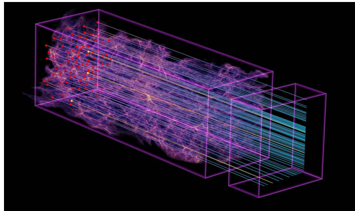
Figure 5.17: The “cosmic web” of the baryon distribution in a cosmological simulation. Here, HI in the IGM traces the dark matter distribution even in regions with low density contrast. A line of sight through the volume yields a one-dimensional map of both the HI and metallic species along the line of sight, as shown in the top panel. Densely sampled sightlines through a survey volume, together with detailed maps of the galaxy distribution, will provide unprecedented views of the distribution of baryons in the Universe, and their relation to the sites of galaxy formation. [Illustration Credit: Zosia Rostomian, LBNL; Nic Ross, BOSS Lyman-alpha team, LBNL; Springel et al, Virgo Consortium and the Max Planck Institute for Astrophysics]
