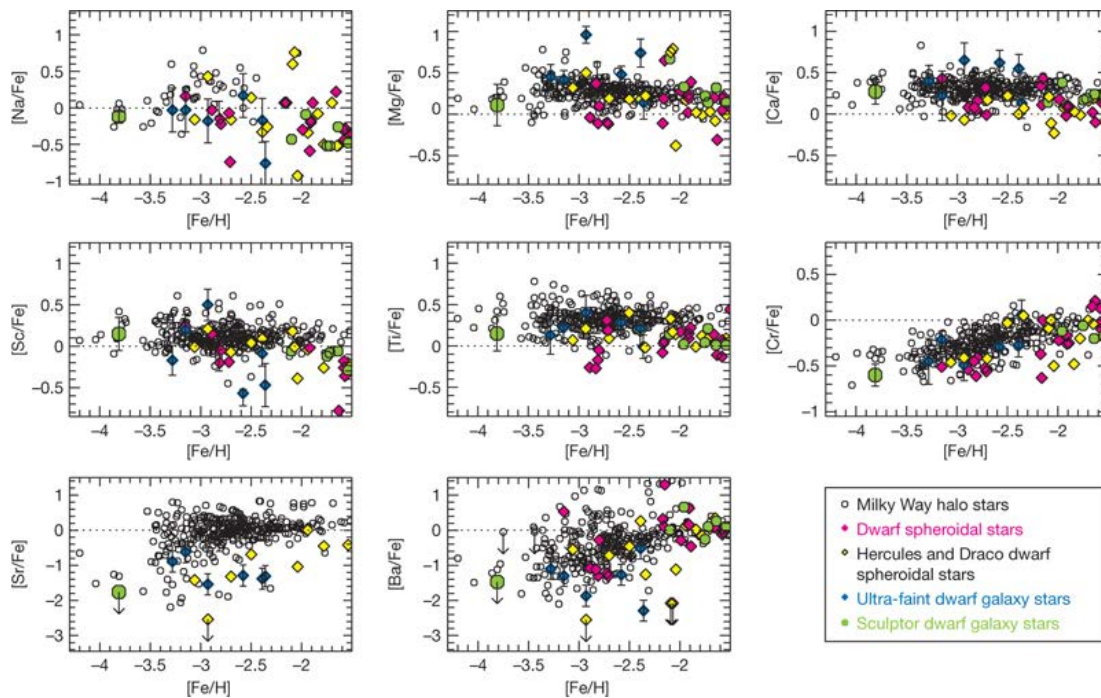
Figure 7.10: Abundance ratios as function of iron abundance in S1020549 and other metal-poor stars from literature. In eight elements, S 1020549 (Big green filled circles, at [Fe/H] = -3.8 ) is compared with halo stars (Black circles), ultra-faint dwarf galaxy stars (blue diamond) and the brighter dwarf galaxy stars (pink and yellow diamond). Smaller green circles indicate higher metallicity Sculptor targets (Frebel et al. 2010). Elemental abundance ratios show that this star has a chemical pattern nearly identical to that of similarly metal-poor halo stars.
