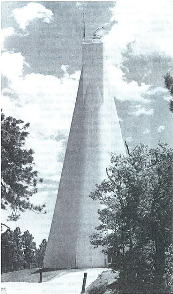
Solar physics. The 7-year-old Solar Vacuum Tower Telescope at Sacramento Peak Observatory in New Mexico provides critical data about solar flares, magnetic fields, and the velocities of matter in the solar atmosphere. Its 30-inch fused quartz entrance window is 136 feet above ground level, and the bottom of the evacuated optical system is 193 feet below ground.
