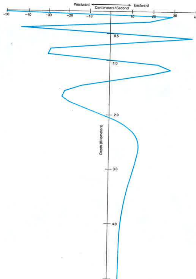
Equatorial tides. An 8-year record (top) of the north-south components of wind at the Maldives Islands, very near the Equator in the Indian Ocean, shows the periodic changes associated with the monsoon. Carl Wunsch of MIT used these annual cycles and a meteorological model to calculate the expected effects on ocean water movement below the surface (right), a calculation that agrees well with actual measurements (left) made 1,000 miles west of the Maldives by James Luyten of Woods Hole Oceanographic Institution. These findings explain how certain tidal variations and parts of the Equatorial Undercurrent system are actually a result of ocean/atmosphere interactions.
