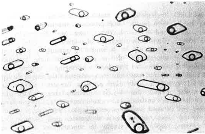
Mineral history. New methods for studying microscopic pockets of fluid trapped in larger crystals now permit the reconstruction of details of how hydrothermal ore deposits were formed. At the left, small bubbles in fluid inclusions of a fluorite crystal can reveal the temperature of the solution when it was entrapped. At the right, a scanning electron micrograph of an opened inclusion shows different minerals that have crystallized from the entrapped fluid.
