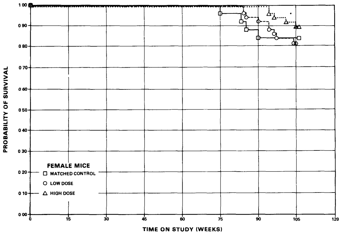
Figure 4. Survival Curves for Mice Administered Diazinon in the Diet
