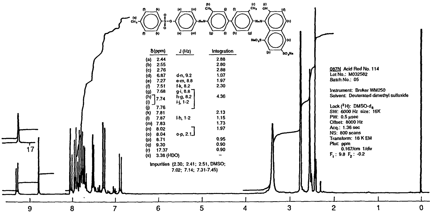
Figure F2 Nuclear Magnetic Resonance Spectrum of C.I. Acid Red 114
