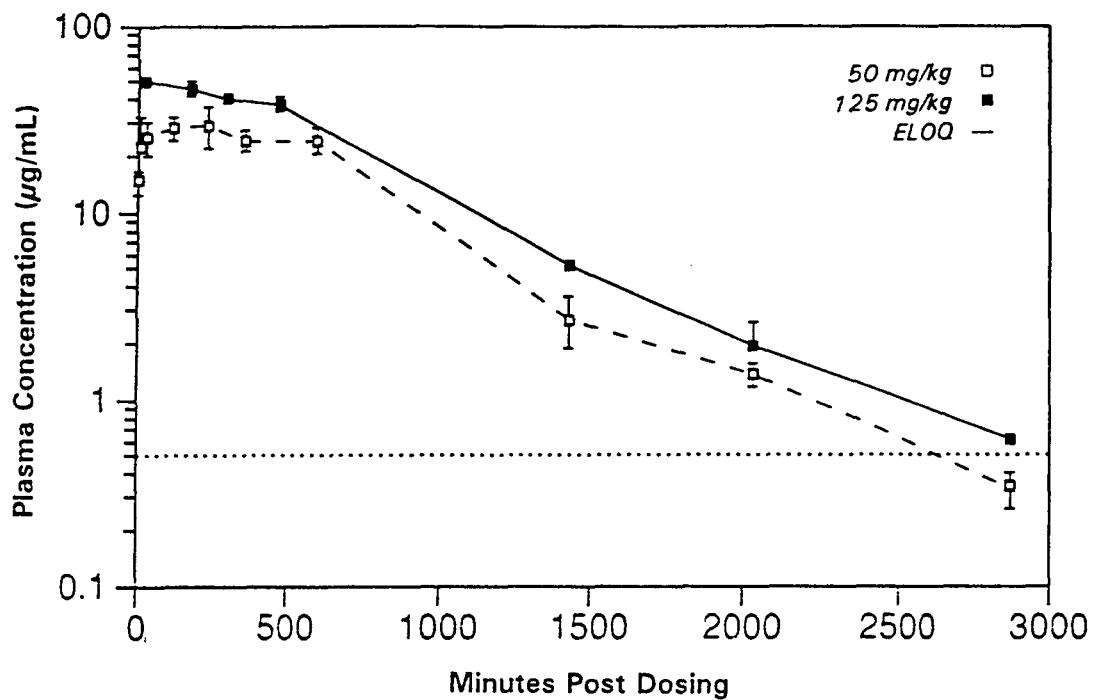
FIGURE O5 Plasma Concentrations of Total Phenolphthalein in Male B6C3F 1 Mice After a Single Gavage Dose of 50 or 125 mg/kg
