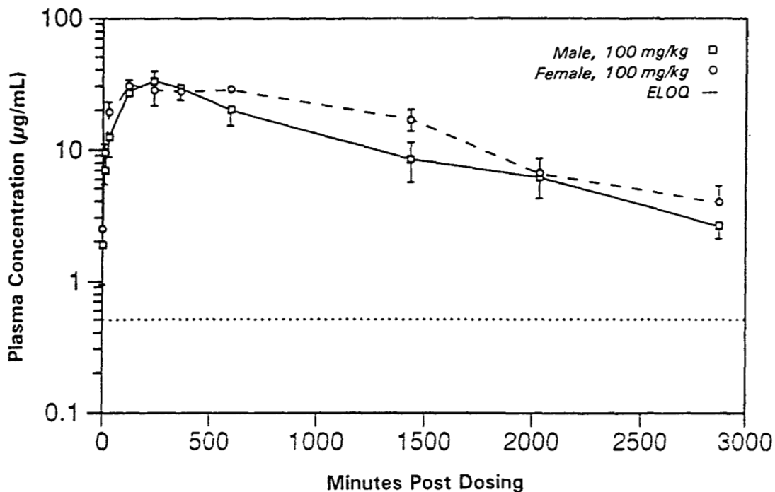
FIGURE O3 Plasma Concentrations of Total Phenolphthalein in Male and Female F344/N Rats After a Single Gavage Dose of 100 mg/kg
