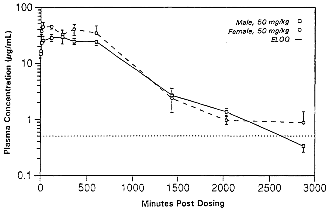
FIGURE O7 Plasma Concentrations of Total Phenolphthalein in Male and Female B6C3F 1 Mice After a Single Gavage Dose of 50 mg/kg
