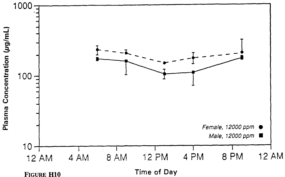
FIGURE H10 Plasma Concentrations of Total Phenolphthalein in Male and Female Mice After Exposure to 12,000 ppm in Feed for 2 Years
