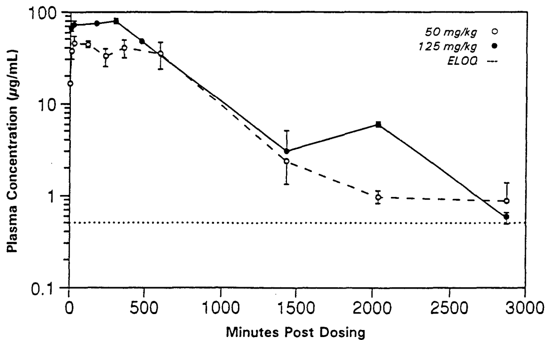
FIGURE O6 Plasma Concentrations of Total Phenolphthalein in Female B6C3F 1 Mice After a Single Gavage Dose of 50 or 125 mg/kg
