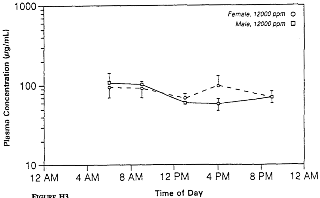
FIGURE H3 Plasma Concentrations of Total Phenolphthalein in Male and Female Rats After Exposure to 12,000 ppm in Feed for 2 Years
