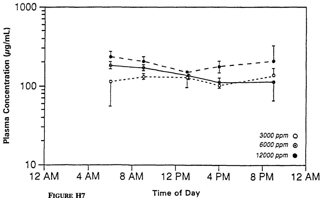
FIGURE H7 Plasma Concentrations of Total Phenolphthalein in Female Mice After Exposure to 3,000, 6,000, or 12,000 ppm in Feed for 2 Years
