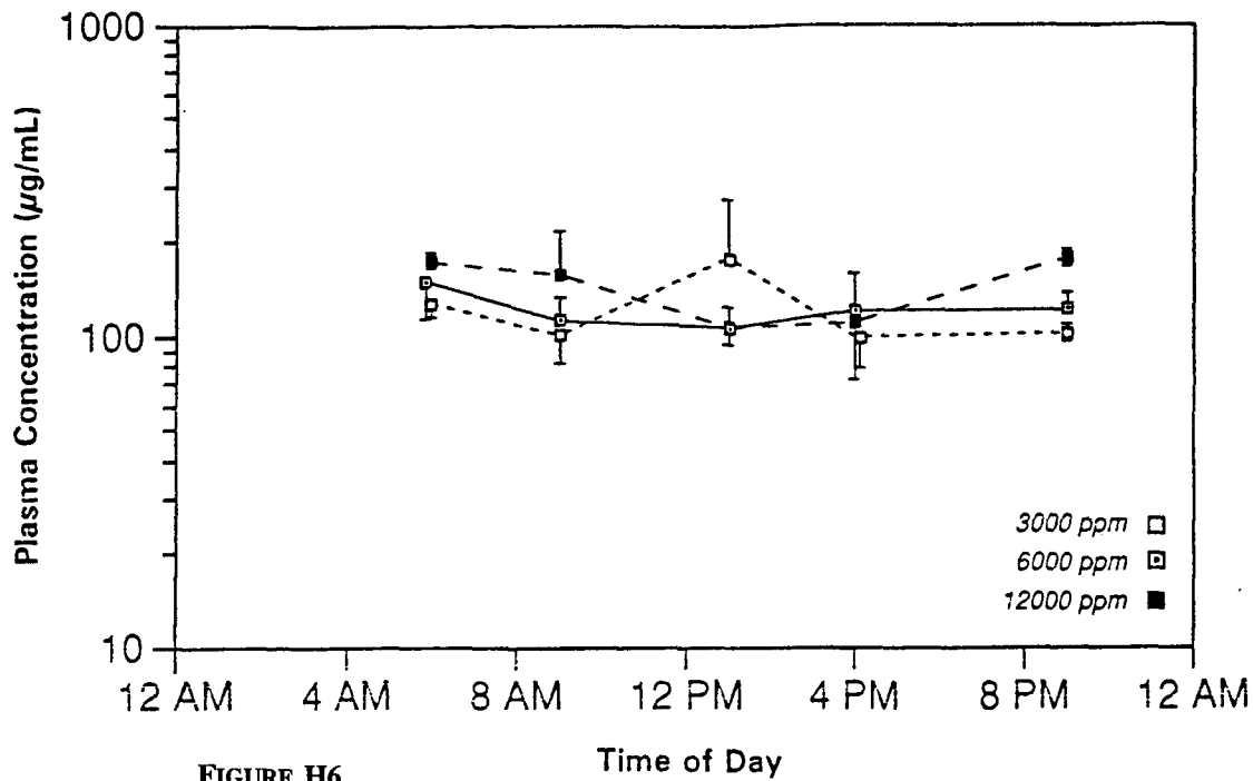
FIGURE H6 Plasma Concentrations of Total Phenolphthalein in Male Mice After Exposure to 3,000, 6,000, or 12,000 ppm in Feed for 2 Years
