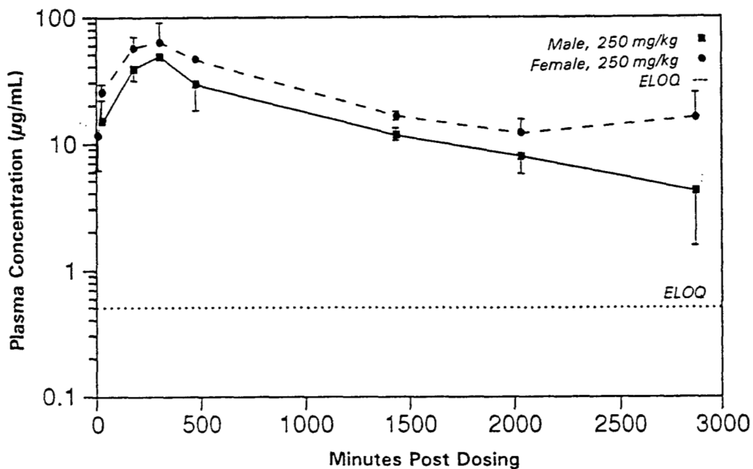
FIGURE O4 Plasma Concentrations of Total Phenolphthalein in Male and Female F344/N Rats After a Single Gavage Dose of 250 mg/kg
