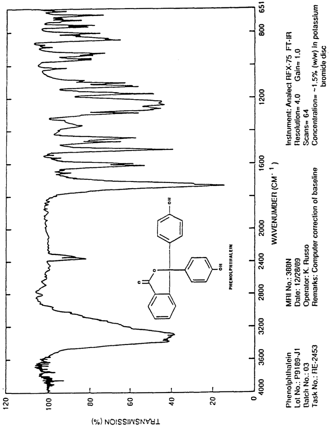
FIGURE J1 Infrared Absorption Spectrum of Phenolphthalein
