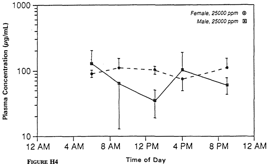
FIGURE H4 Plasma Concentrations of Total Phenolphthalein in Male and Female Rats After Exposure to 25,000 ppm in Feed for 2 Years
