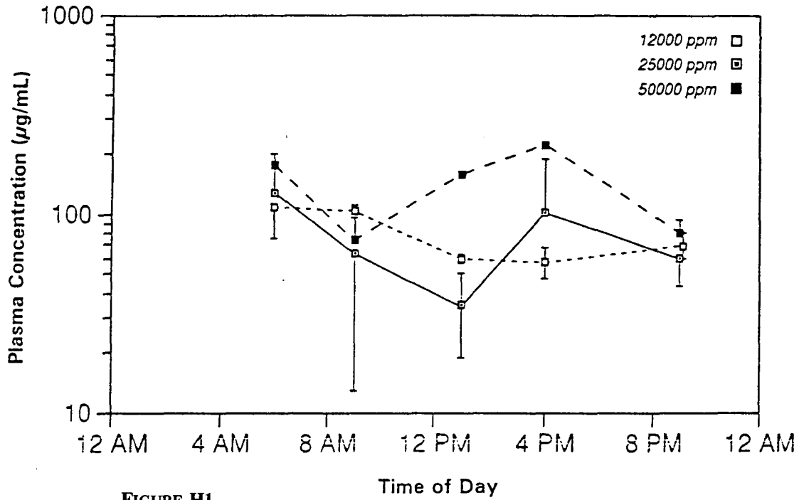
FIGURE H1 Plasma Concentrations of Total Phenolphthalein in Male Rats After Exposure to 12,000, 25,000, or 50,000 ppm in Feed for 2 Years
