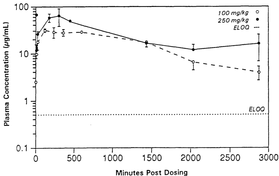
FIGURE O2 Plasma Concentrations of Total Phenolphthalein in Female F344/N Rats After a Single Gavage Dose of 100 or 250 mg/kg
