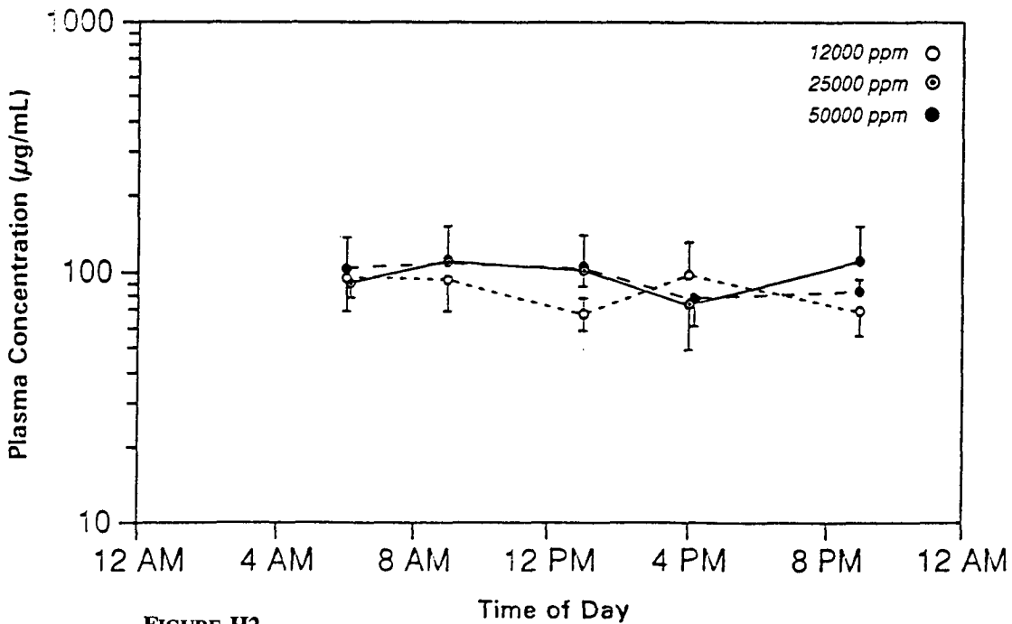
FIGURE H2 Plasma Concentrations of Total Phenolphthalein in Female Rats After Exposure to 12,000, 25,000, or 50,000 ppm in Feed for 2 Years
