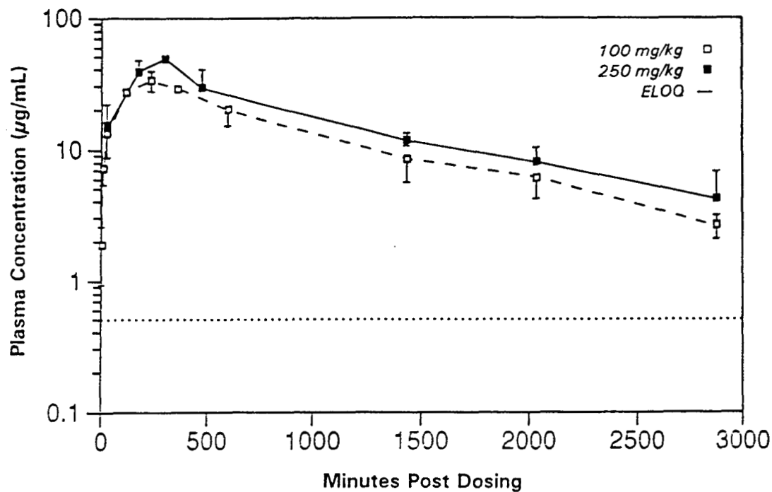
FIGURE O1 Plasma Concentrations of Total Phenolphthalein in Male F344/N Rats After a Single Gavage Dose of 100 or 250 mg/kg
