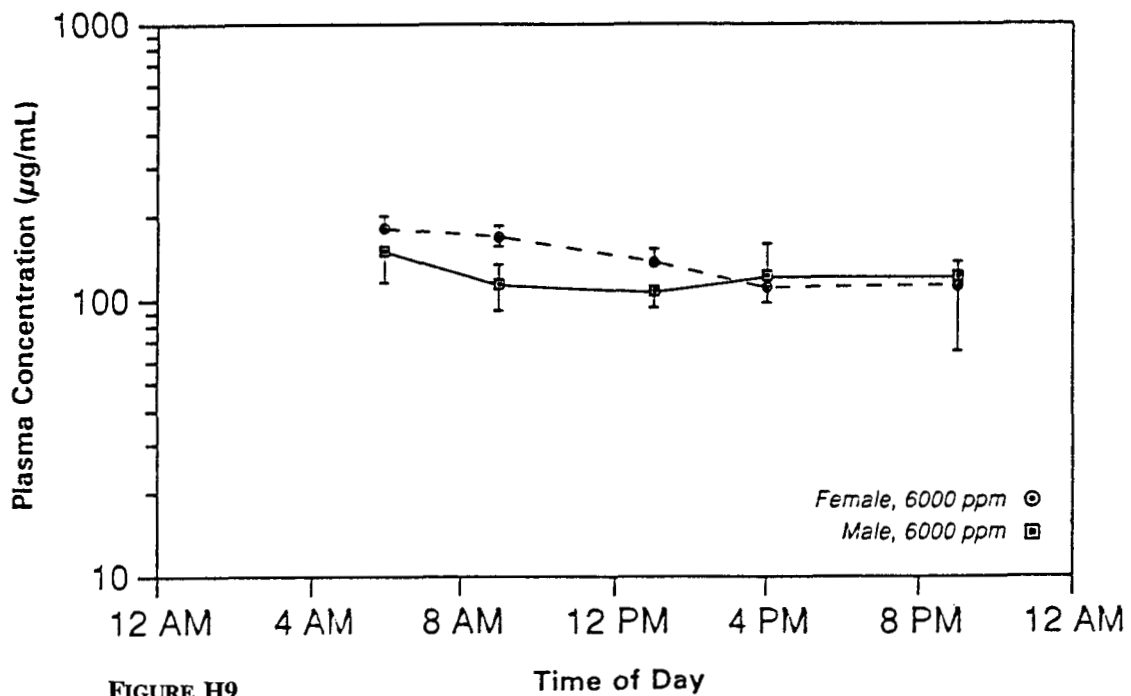
FIGURE H9 Plasma Concentrations of Total Phenolphthalein in Male and Female Mice After Exposure to 6,000 ppm in Feed for 2 Years
