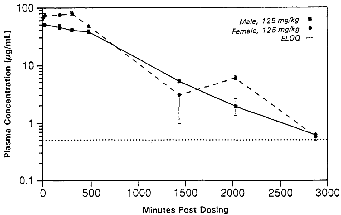
FIGURE O8 Plasma Concentrations of Total Phenolphthalein in Male and Female B6C3F 1 Mice After a Single Gavage Dose of 125 mg/kg
