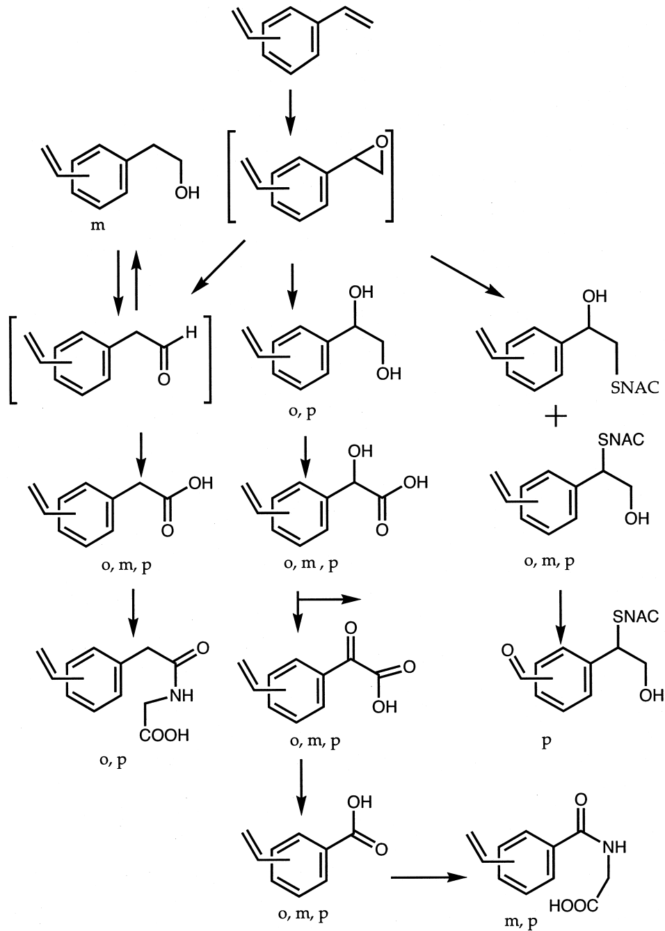
FIGURE 2 Metabolic Pathway for Divinylbenzenes
