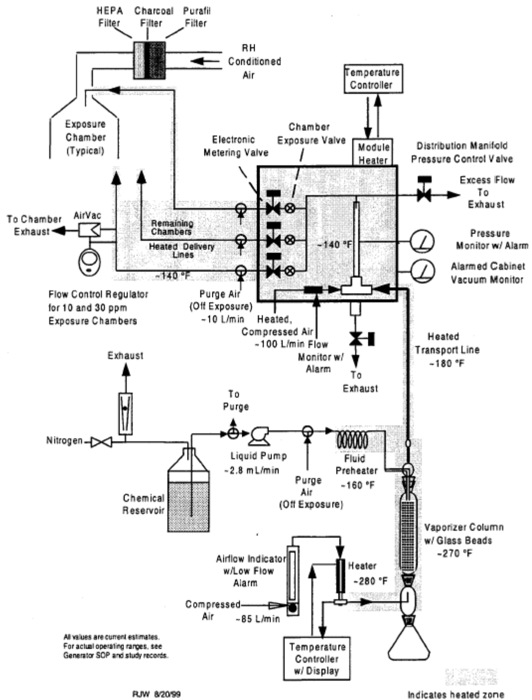
FIGURE I4 Schematic of the Vapor Generation and Delivery System in the Inhalation Studies of Divinylbenzene-HP
