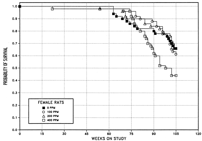
FIGURE 3 Kaplan-Meier Survival Curves for Male and Female Rats Exposed to Divinylbenzene-HP by Inhalation for 2 Years
